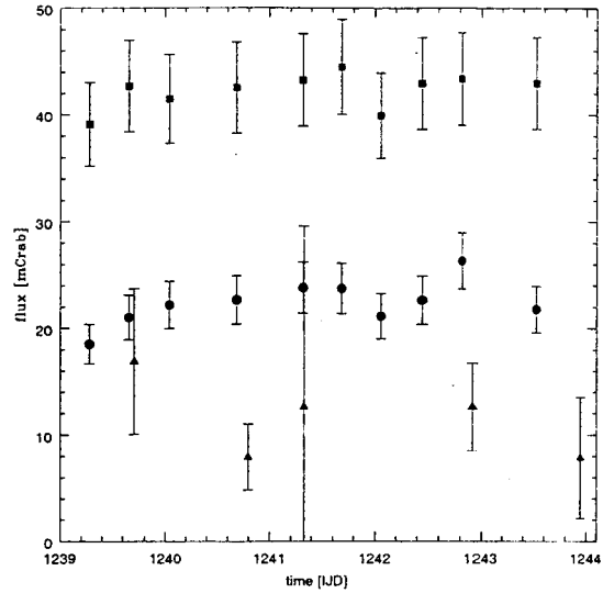
Fig. 1.— INTEGRAL and RXTE/ASM light curves in Crab units. The squares and circles represent the 20–100 keV ISGRI and 5–20 keV JEM-X2 lightcurve, respectively. Fluxes were extracted from model fits to the data. The triangles are RXTE/ASM 1.5–12 keV daily averages.
