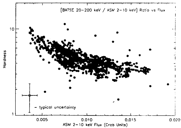
Fig. 6.— Spectral hardness derived from the BATSE and RXTE data, versus the RXTE/ASM flux. A softer spectrum is correlated with a higher flux. The error bars on the lower left show the typical uncertainties of the measurements.
