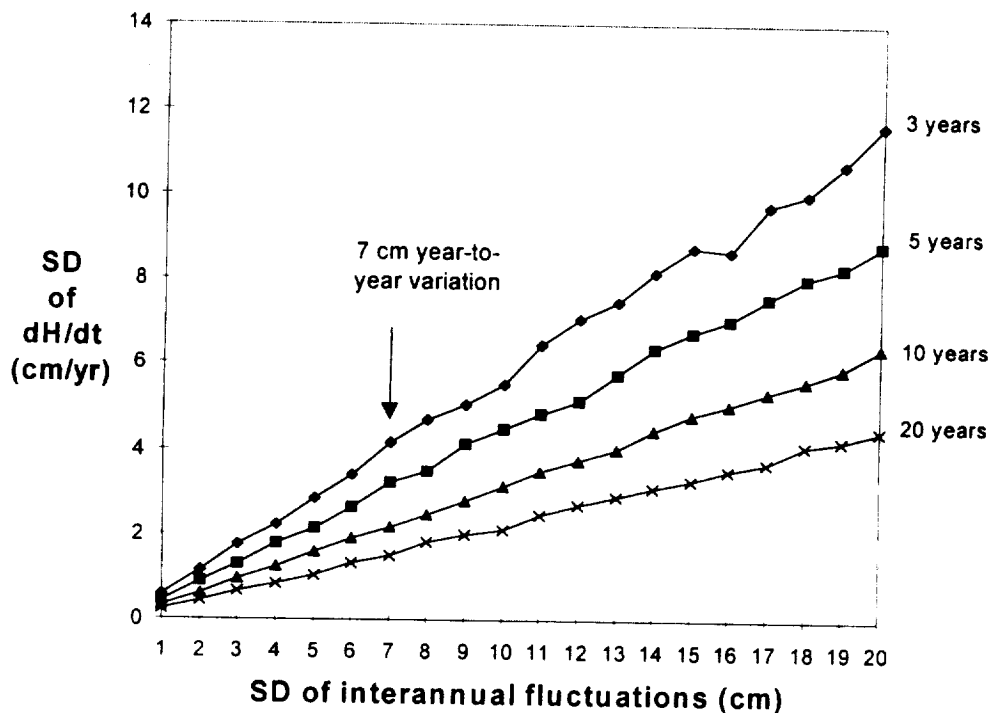
Figure 2. Uncertainty in dH/dt results associated with random interannual variations in surface elevation for time periods of 3 to 20 years. Results were derived from a Monte Carlo simulation.
