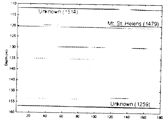
Figure 1(b). Radar echogram of internal layers observed at NGRIP (110-160m).
