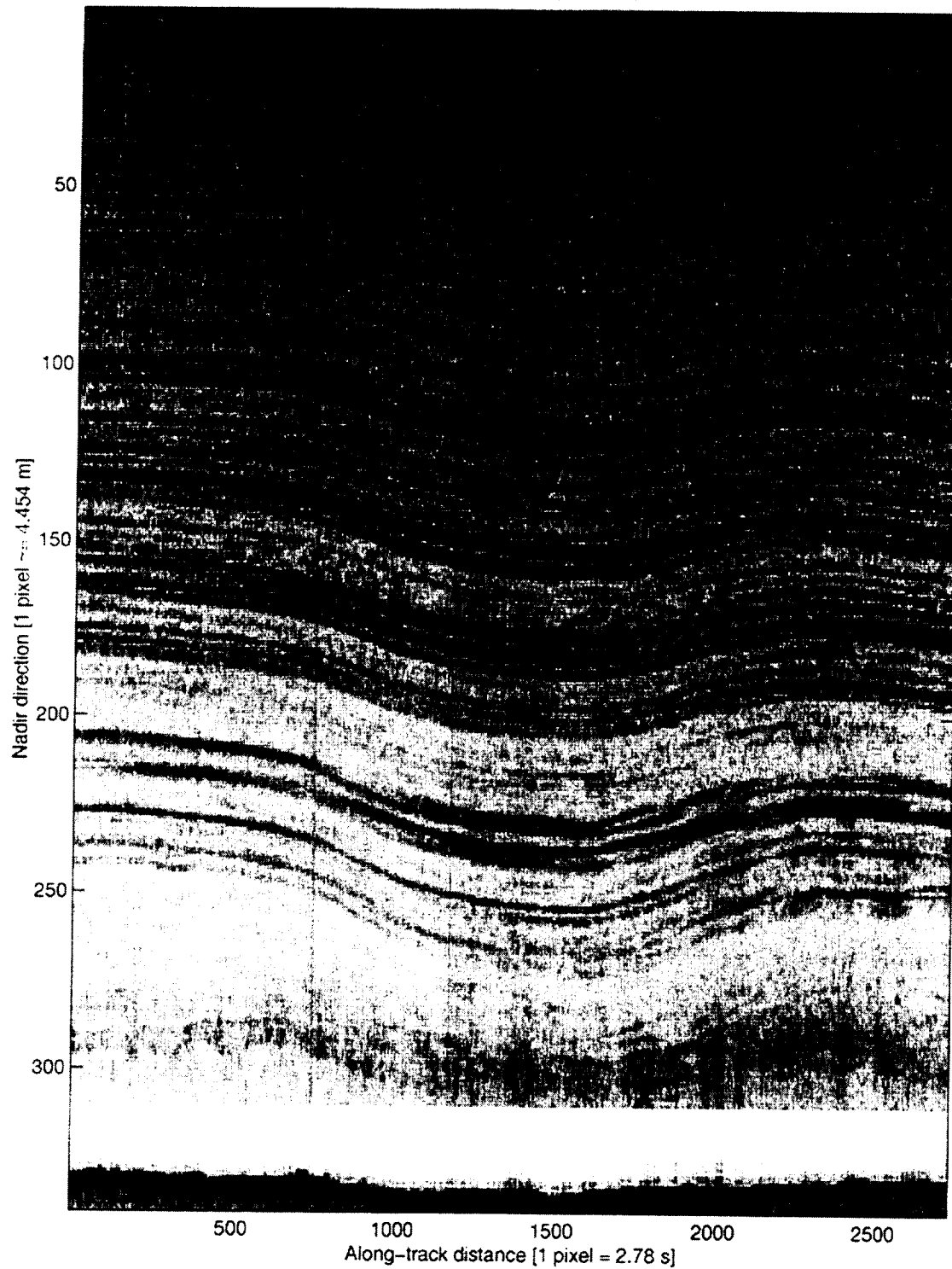
Figure 5. Expanded bottom view of the NGRIP radio echogram. Internal layer around pixel 300 is at a depth of about 2880 m. The bottom depth is about 3080 m at pixel 345.
