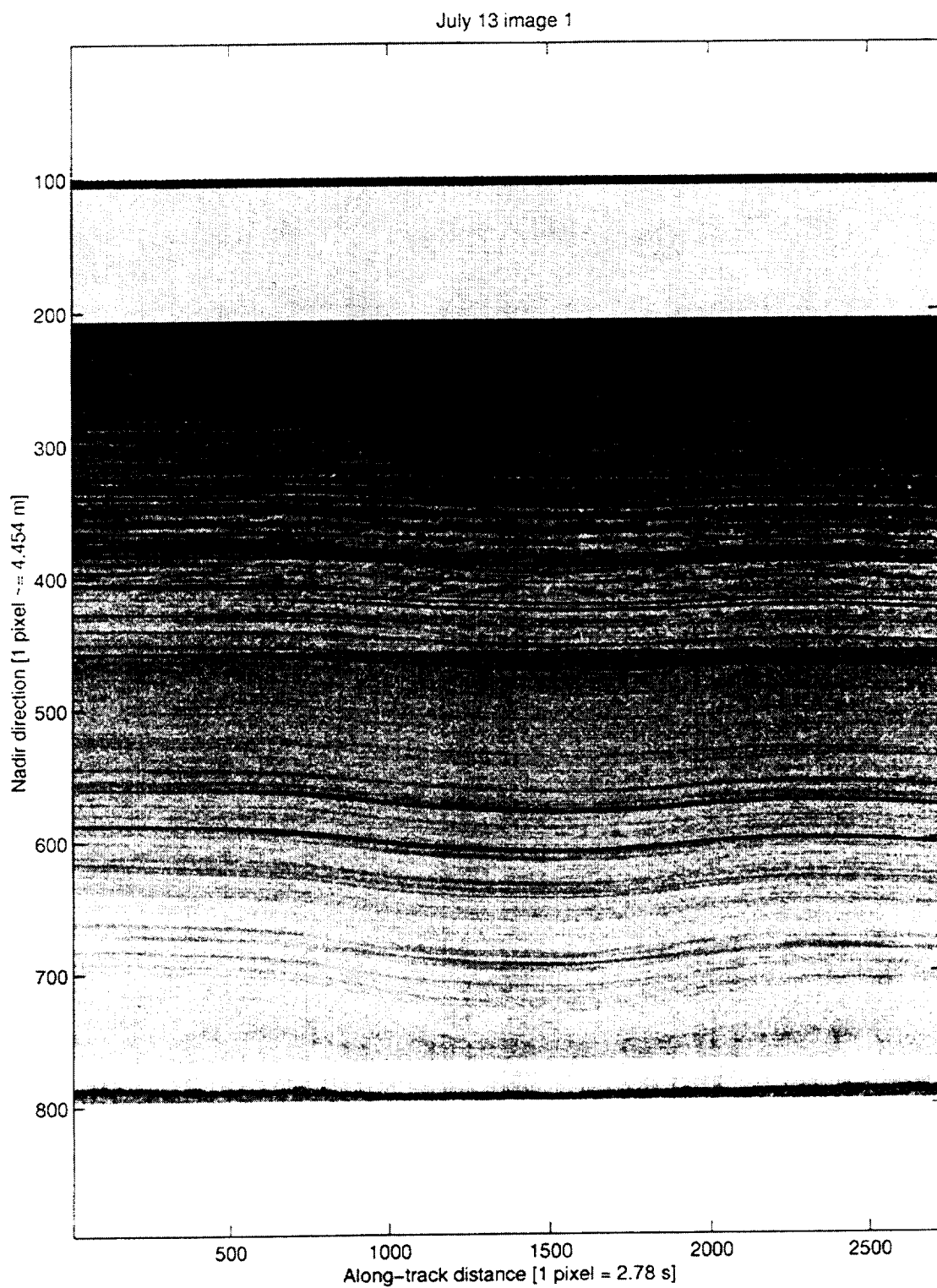
Figure 4. Radio echogram collected at NGRIP, Greenland.
