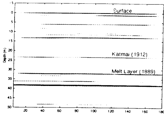
Figure 1(a). Radar echogram of internal layers observed at NGRIP (0-50m).
