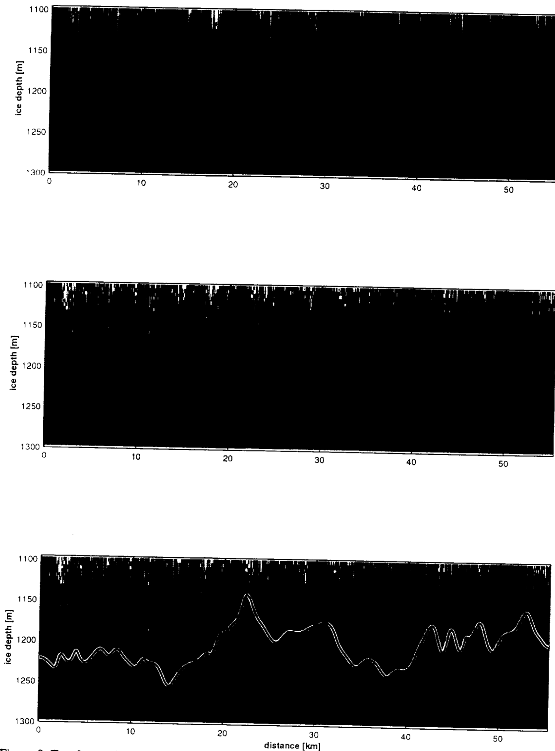
Figure 3. Top frame shows unfocused radar data. Middle frame shows focused radar data with a weak internal layer signal-to-noise ratio improved. Bottom frame shows the detected internal layer. Data were collected over Southwest Greenland.
