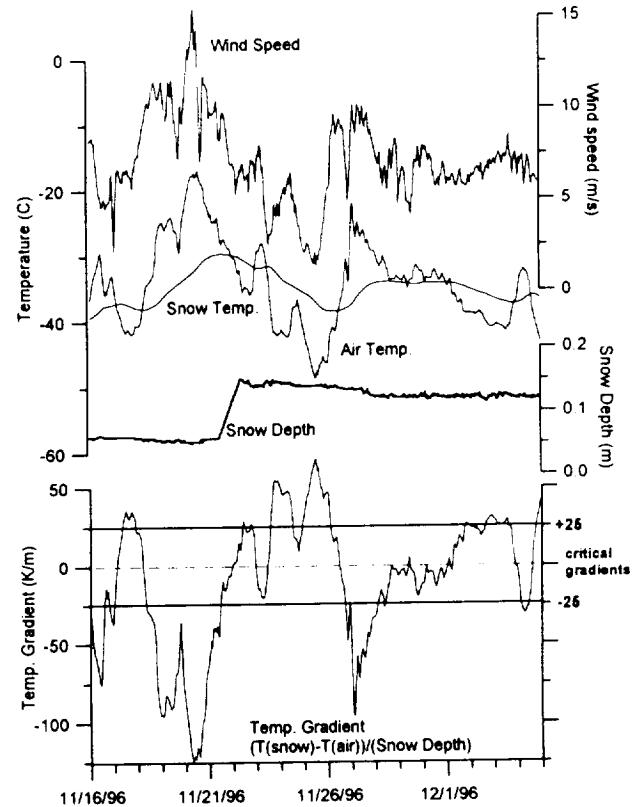
Fig. 6: Hourly automatic weather station record of wind speed, air and snow temperatures, and snow height for Tunu-N in north-east Greenland (Fig. 1). The zero level for the snow height represents the summer 1996 height, and the position of the first snow temperature thermistor. The temperature gradient in the top snow layer exceeds the critical value of 25 \text{ K m}^{-1} necessary for faceted crystal development several times
