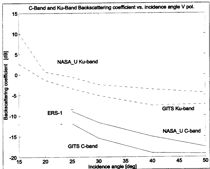
Figure 1: Comparison between Ground-based and ERS-1 (C-band) backscattering coefficients.
