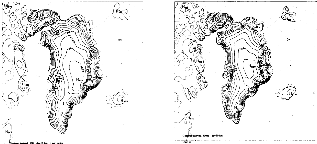
Figure 2. (a) The topography of Greenland and adjacent areas (in meters with a contour interval of 300 m); (b) same as (a) but based on Ekholm (1996). Notice the large difference over Greenland just to the south of 70°N.
