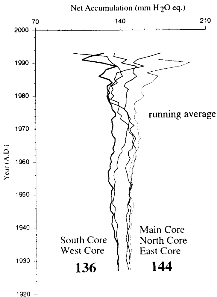
Figure 1. Net accumulation for various shallow cores at the Humboldt Site in Greenland.
