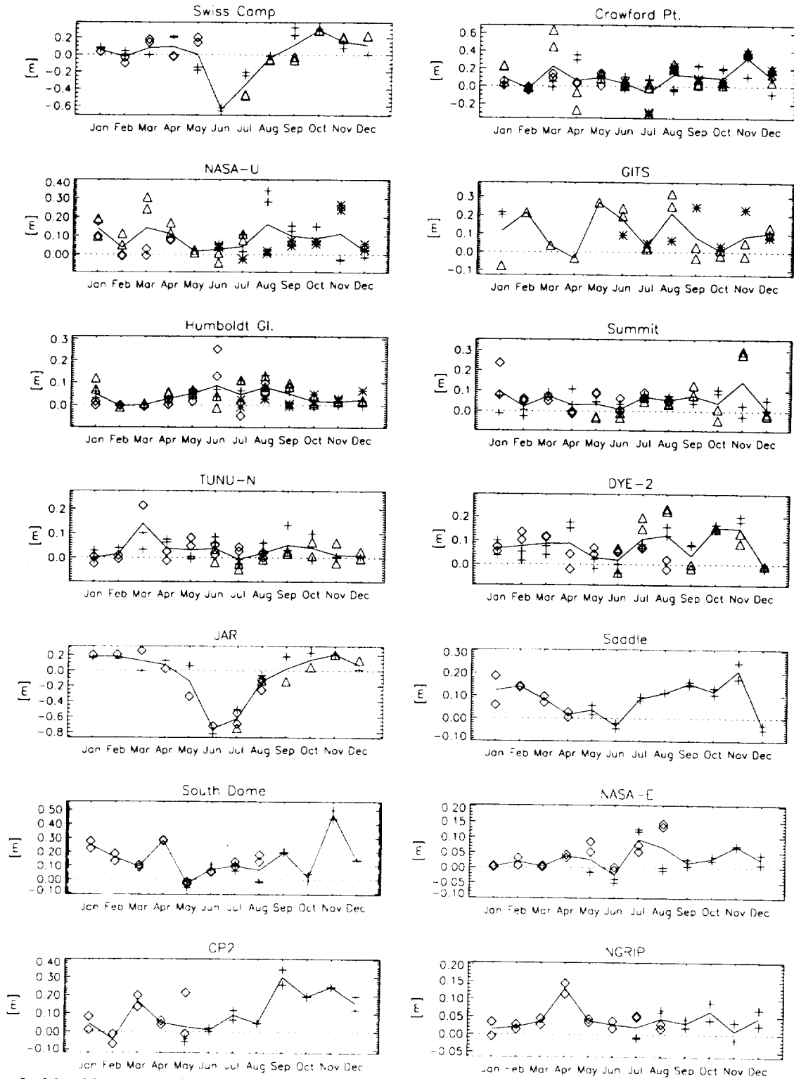
Fig. 2: Monthly mean surface height change: * - 1995, Δ - 1996, + 1997, ◊ 1998, ___ - average.
