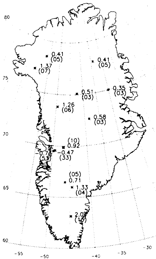
Figure 1: Mean annual elevation changes (in meters) as observed at the GC-Net AWS sites. In parentheses are the standard deviations ( \sigma ) in cm. after detrending. In the case of JAR, the westernmost station well into the ablation zone, \sigma can be reduced from 51 cm to 16.5, when only the ablation period is considered (taken to be May 15 th – September 15 th ). Elevation changes average 60 cm per month during the summer months.
