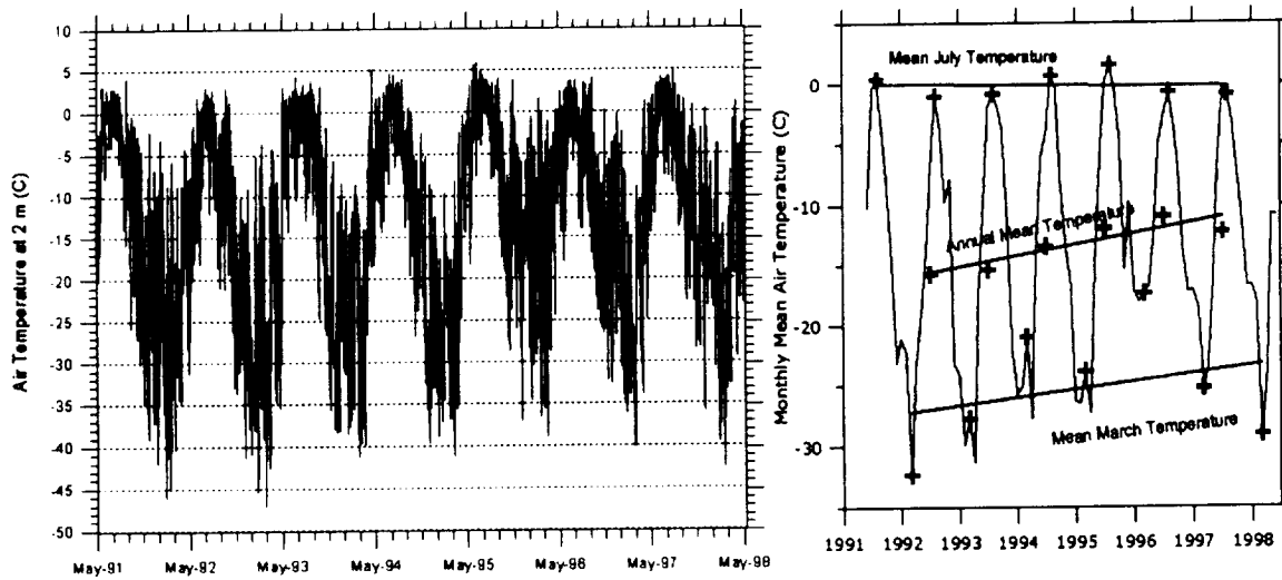
Fig. 3: Hourly and mean monthly air temperatures for the Swiss Camp (ETH/CU AWS) for 1991-1998. A linear regression line is shown for the July mean temperature, March mean temperature and annual mean temperature.
