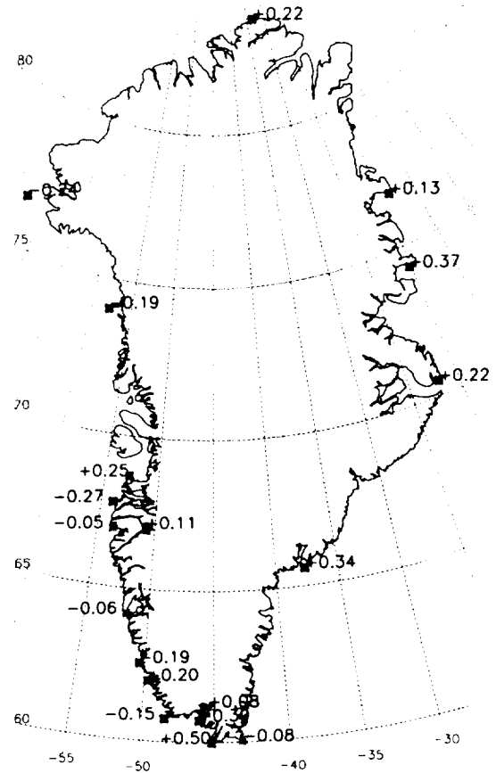
Figure 2: Deviation of average 1993-1997 summer (June – August) temperatures from the 1979-1997 mean. Positive values indicate that the period recent years were anomalously warm at the weather station site, while negative values indicate that the recent period was colder.
