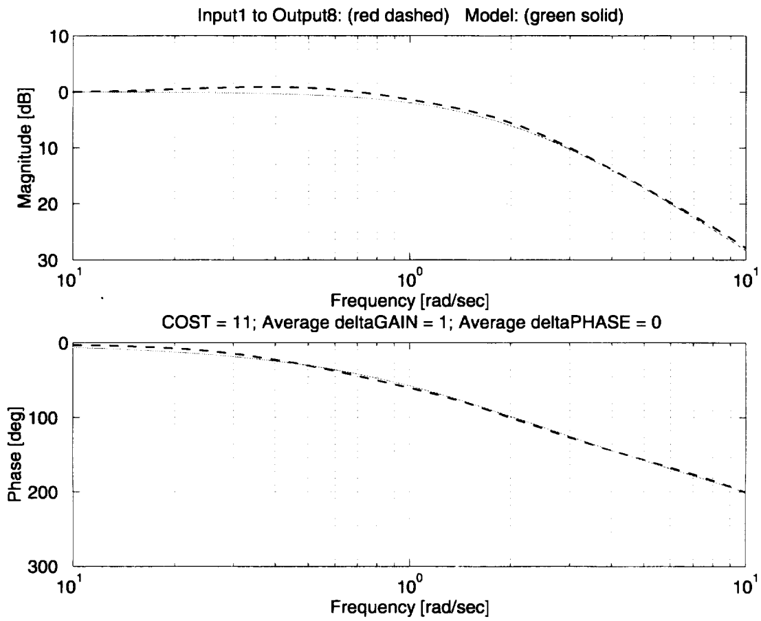
Figure 27. Supporting plot for the model following spec with optimized solution (pitch).
