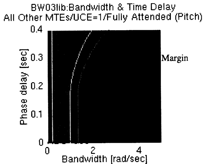
Figure 6. Bandwidth specification with a 0.4 design margin.
