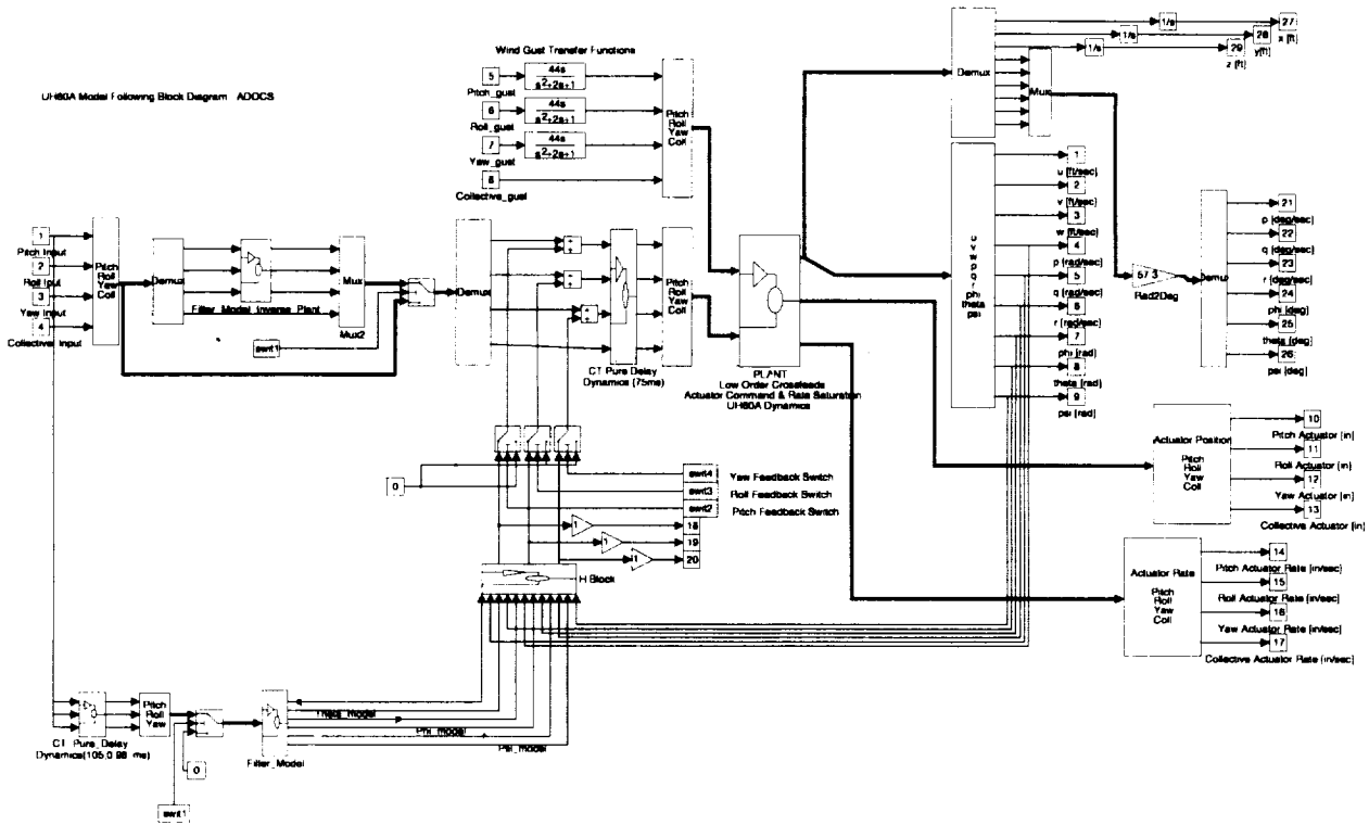
Figure 11. UH-60A model following control law.
