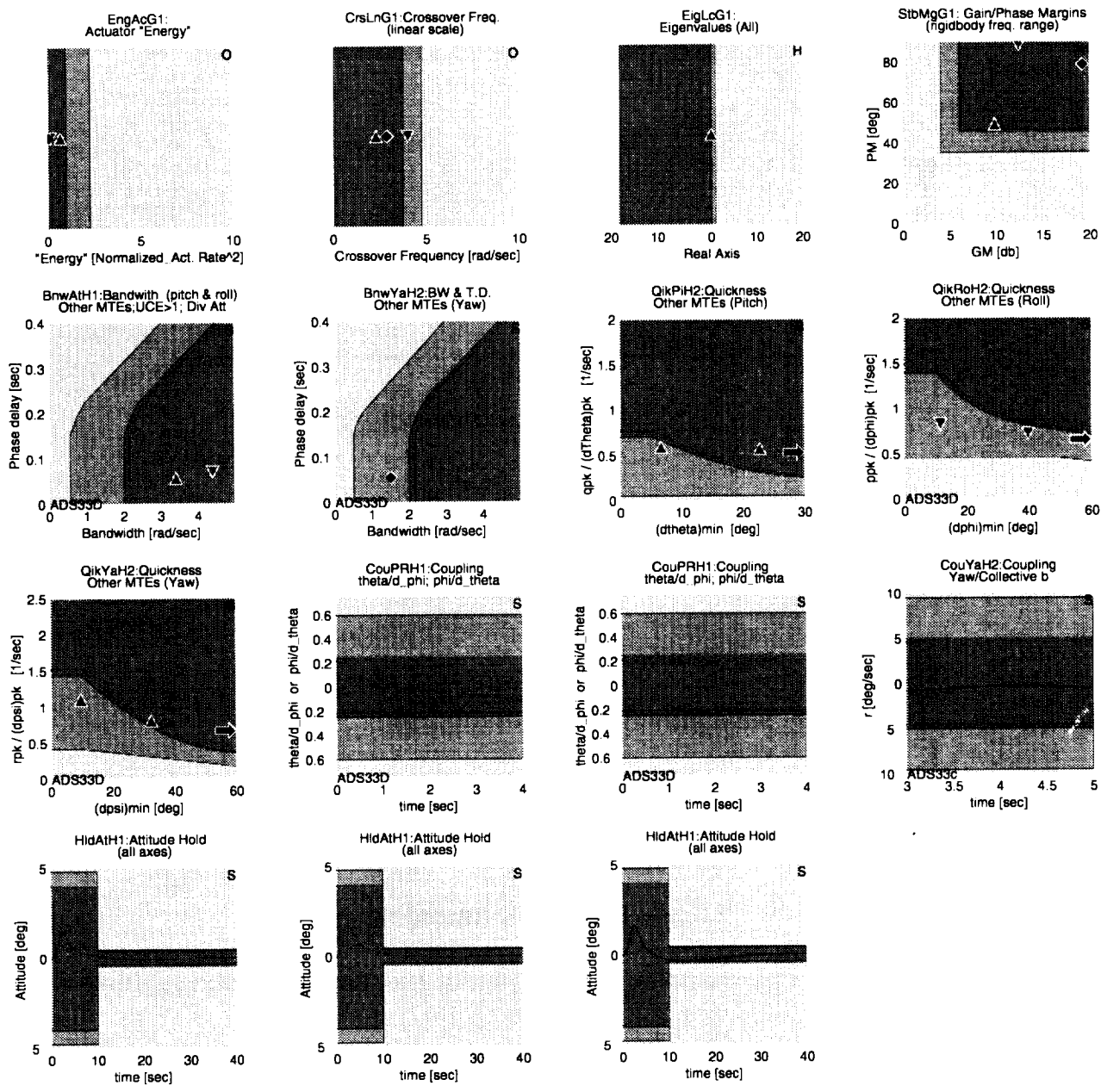
Figure 13. Handling quality analysis of baseline control laws.
