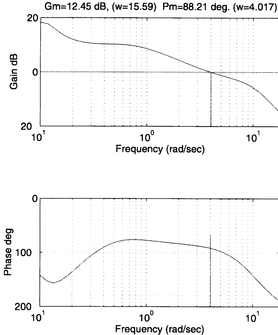
Figure 16. The broken loop frequency response for the roll channel for the baseline solution.
