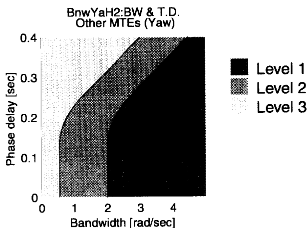
Figure 1. Example ADS-33 bandwidth specification.
