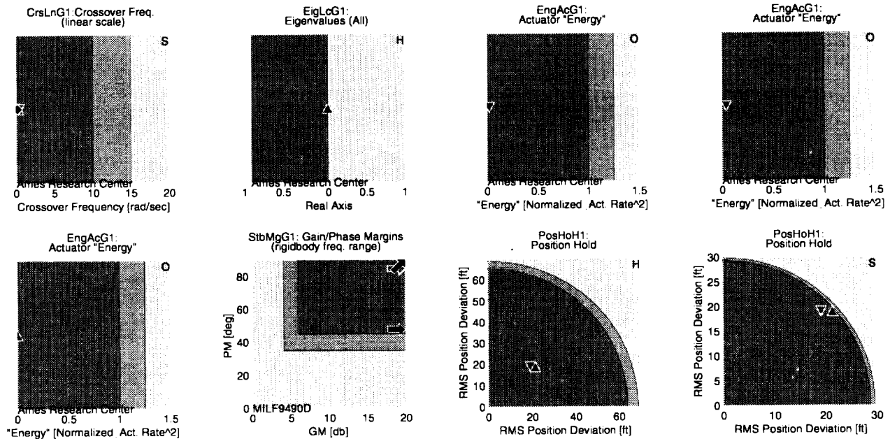
Figure 38. Large RMS position (minimized roll actuator energy).
