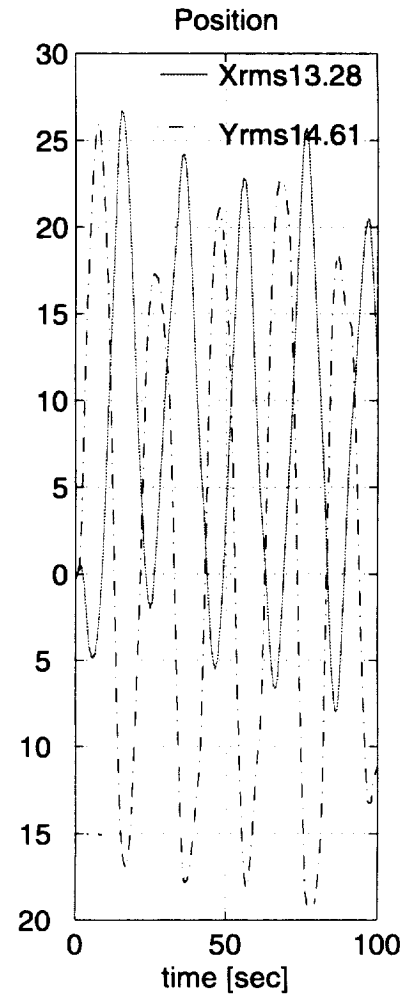
Figure 36. Time history plot of the helicopter's position for medium RMS position.
