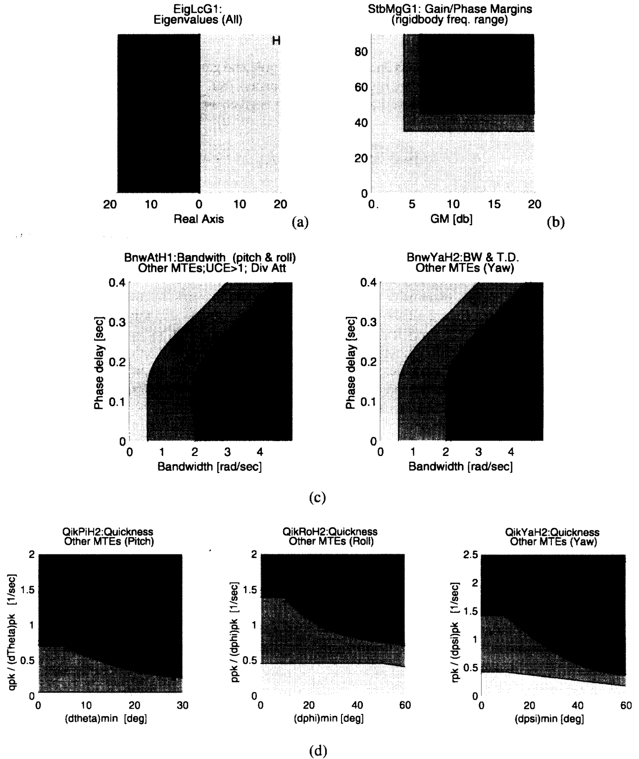
Figure 12. Specifications used in ADS-33 control law design. (a) Eigenvalue stability. (b) Gain and phase margin. (c) Bandwidth. (d) Quickness specifications.
