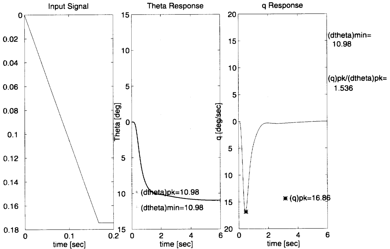
Figure 19. The supporting plots for the roll quickness specification for small input signal once it has achieved Level 1.
