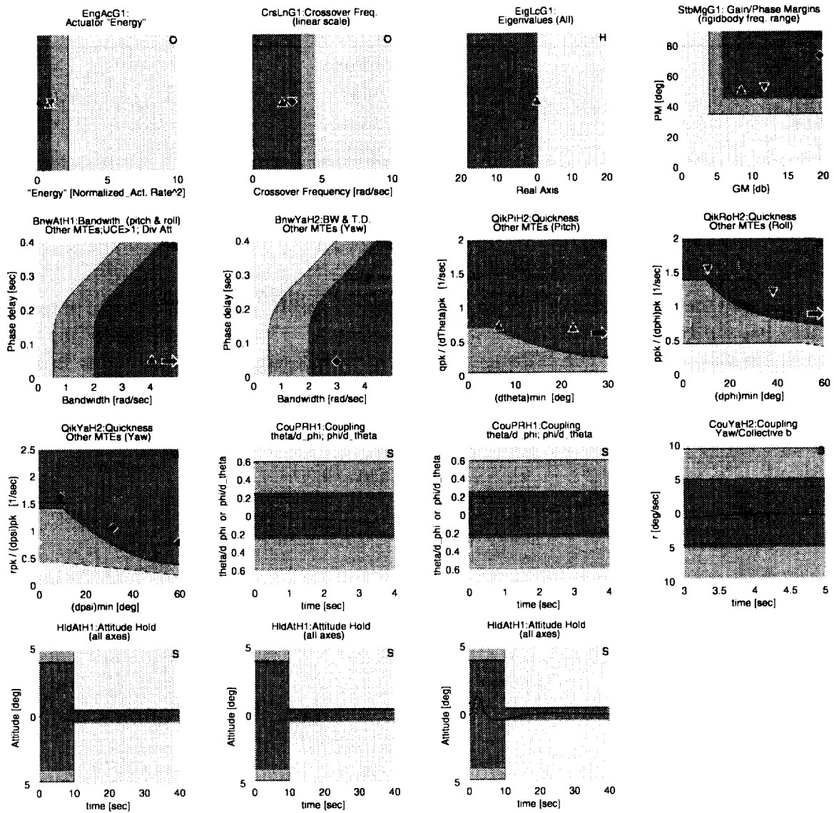
Figure 17. CONDUIT optimized solution.
