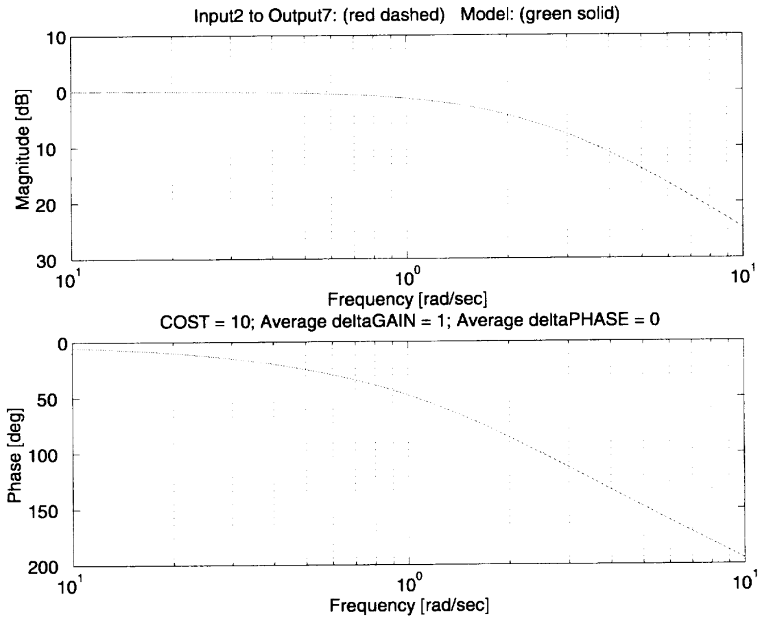
Figure 28. Supporting plot for the model following spec with optimized solution (roll).
