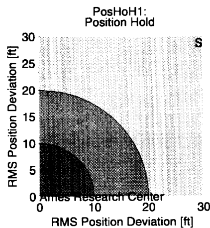
Figure 31. The position hold specification.
