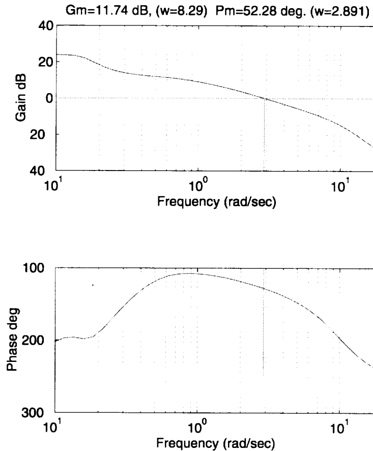
Figure 20. Roll channel gain and phase margin supporting plot after tuning in CONDUIT environment.
