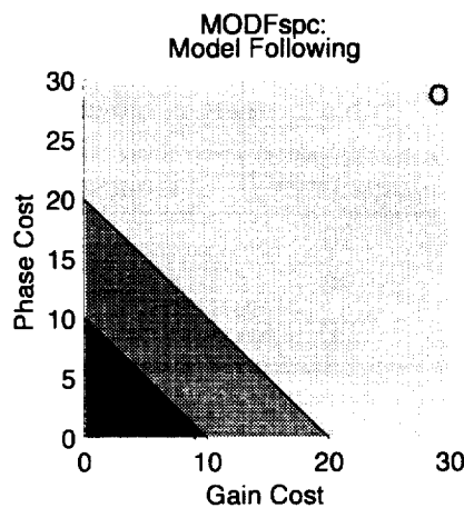
Figure 21. The model following specification.
