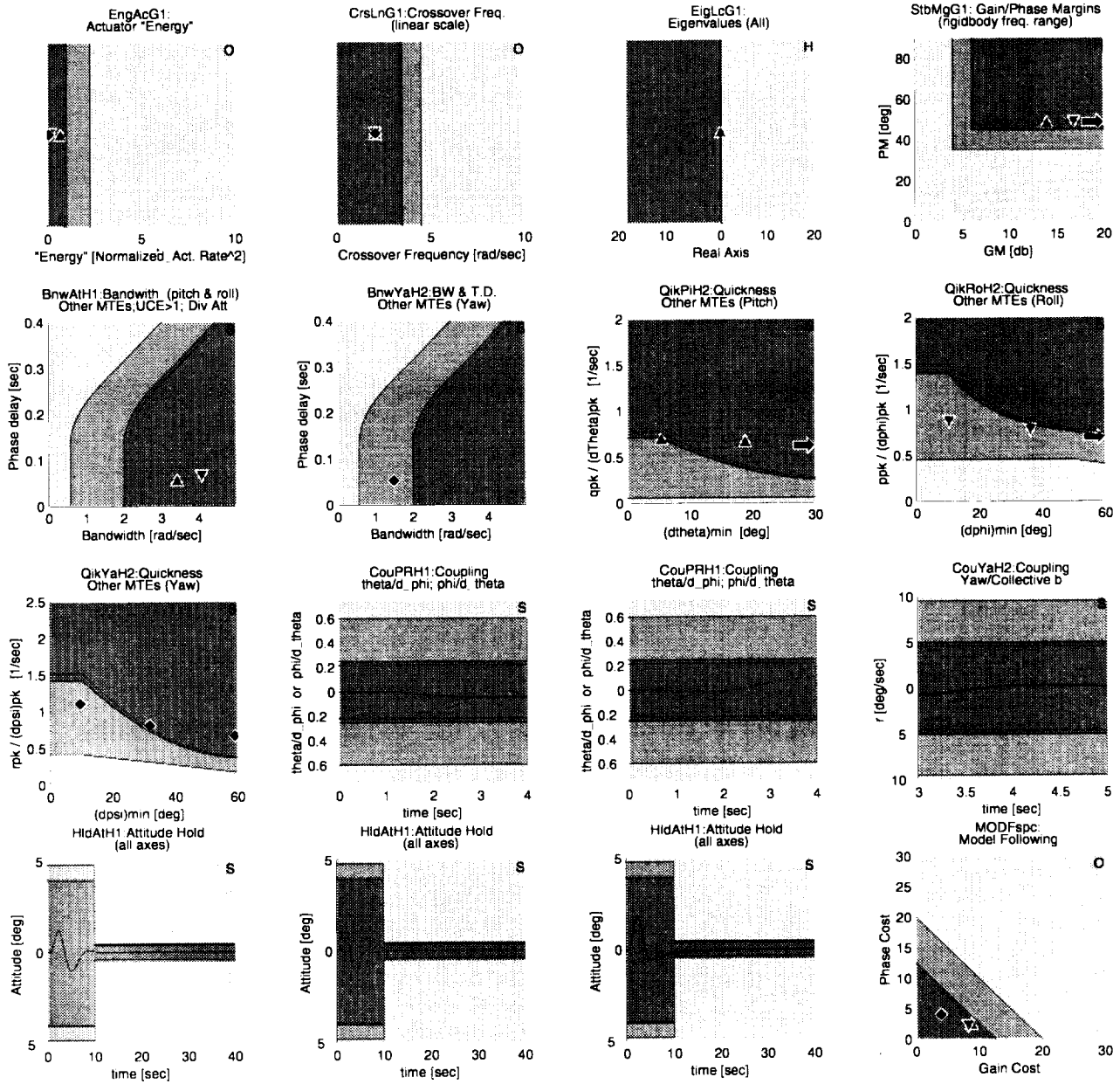
Figure 26. CONDUIT's optimized parameters for the model following solution.
