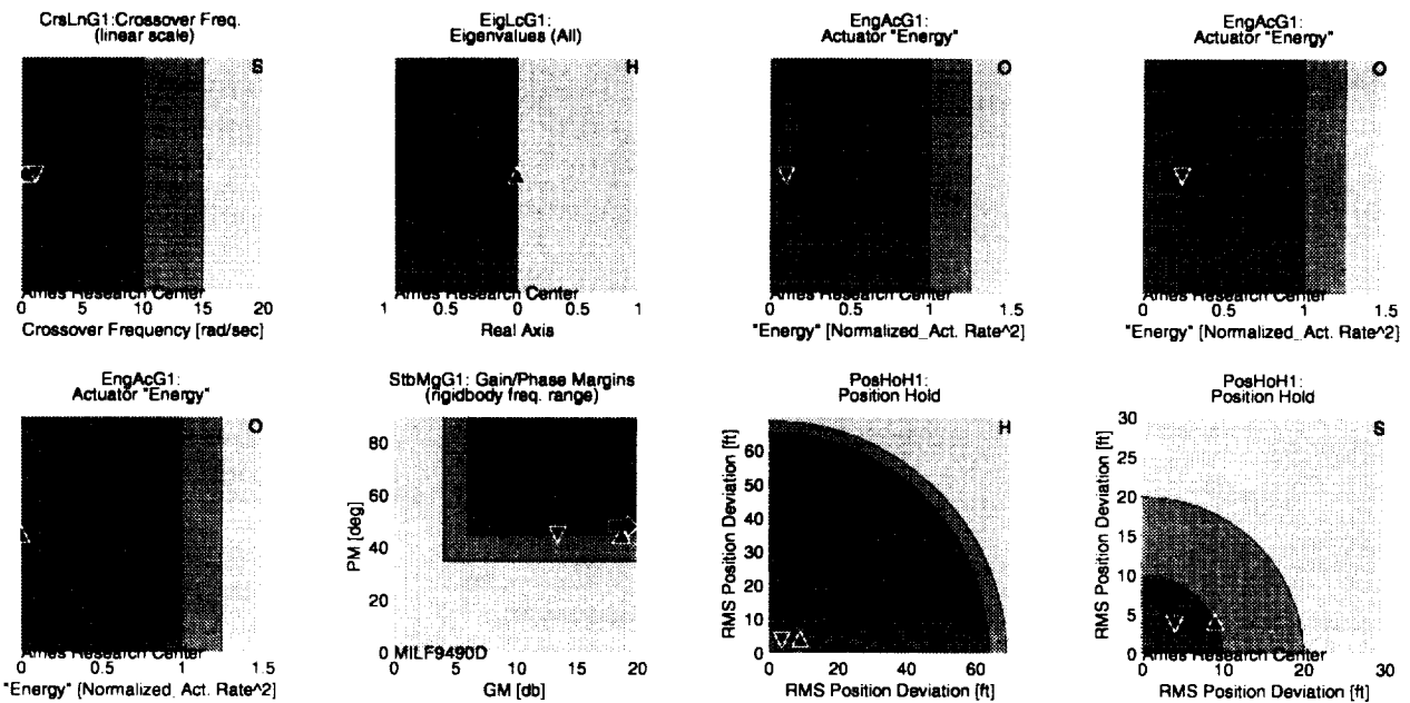
Figure 32. Wind gust solution for minimized RMS position.
