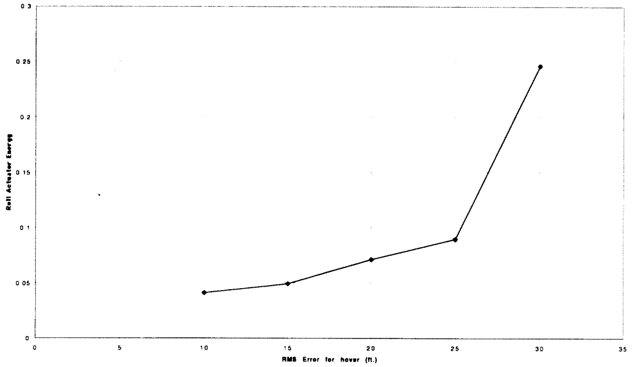
Figure 41. The trade-off between hover hold and actuator energy.
