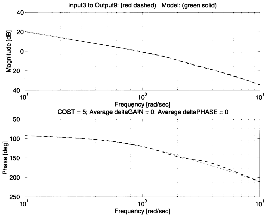
Figure 25. Supporting plot for the model following spec (yaw).
