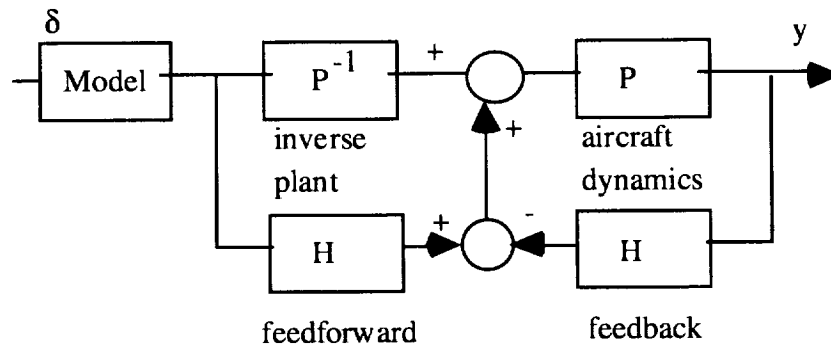
Figure 10. Model following block diagram.
