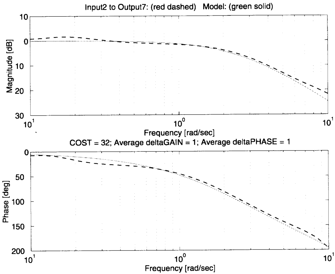
Figure 24. Supporting plot for the model following spec (roll).
