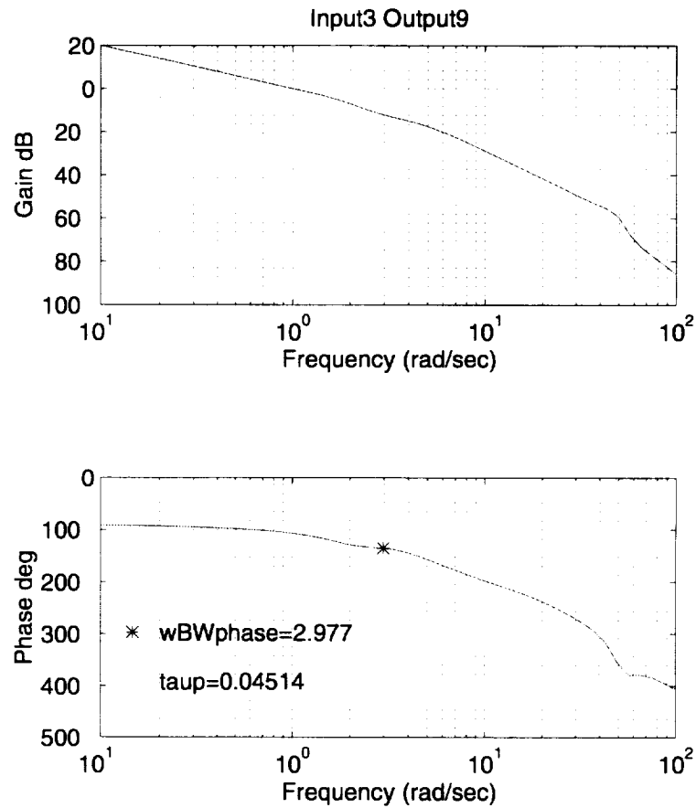
Figure 18. Yaw bandwidth supporting plots.
