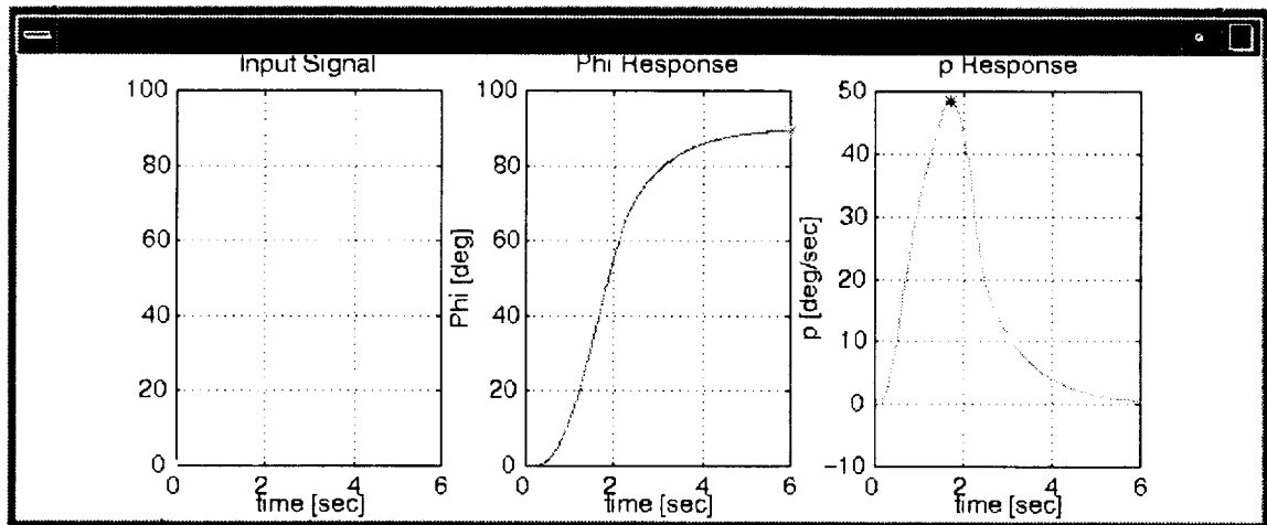
Figure 2. Example of supporting information required for the ADS-33 quickness specification.
