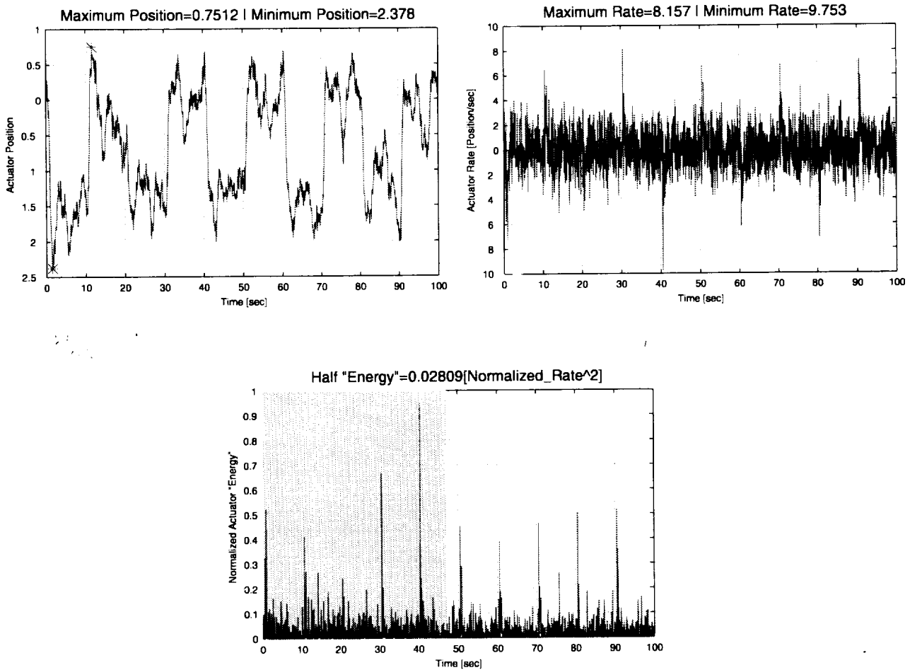
Figure 40. Supporting plot for actuator energy (roll) with saturation in the actuator rate.
