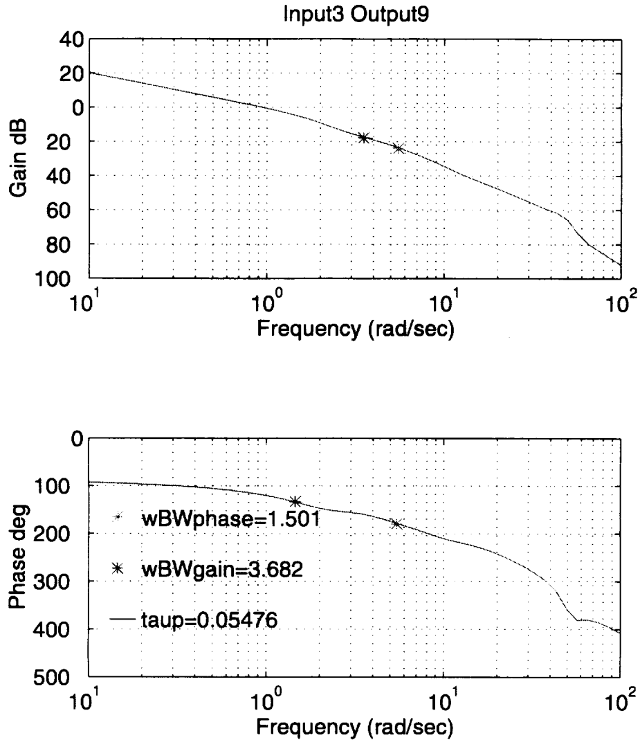
Figure 14. Showing the bandwidth for the yaw channel using baseline design parameters.
