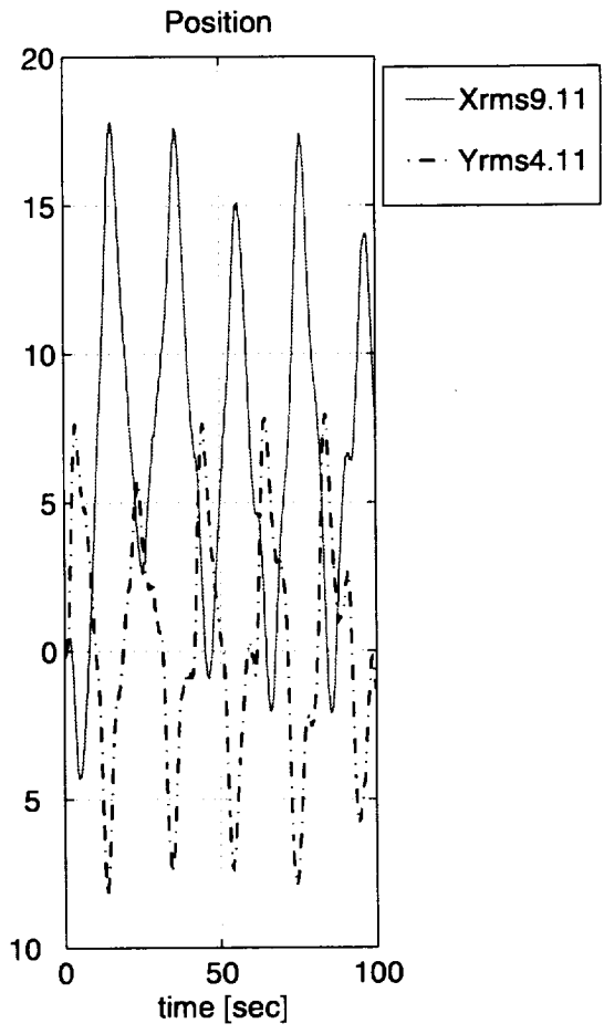
Figure 33. Time history plot of the helicopter's position for minimized RMS position.
