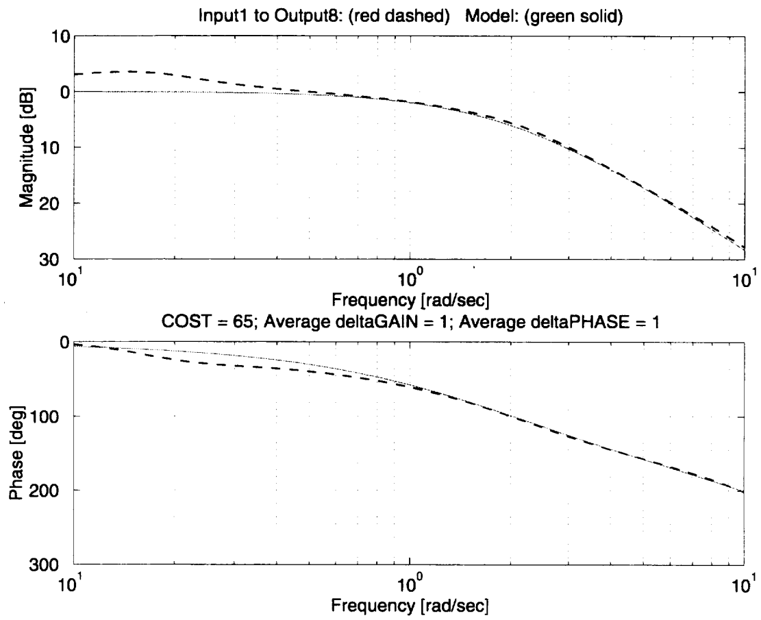
Figure 23. Supporting plot for the model following spec (pitch).
