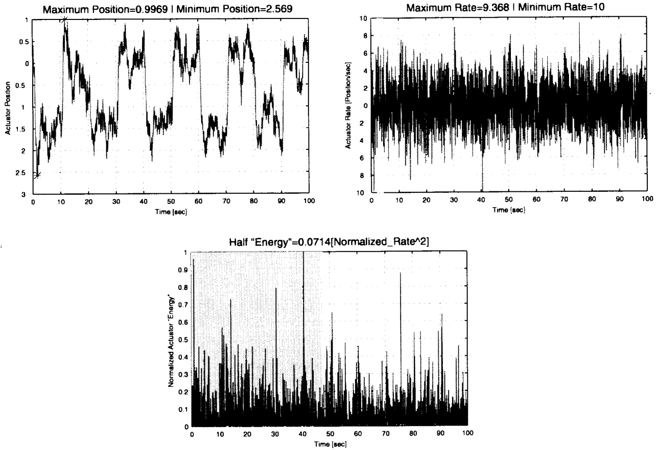
Figure 37. Supporting plot for actuator energy (roll) with saturation in the actuator rate.
