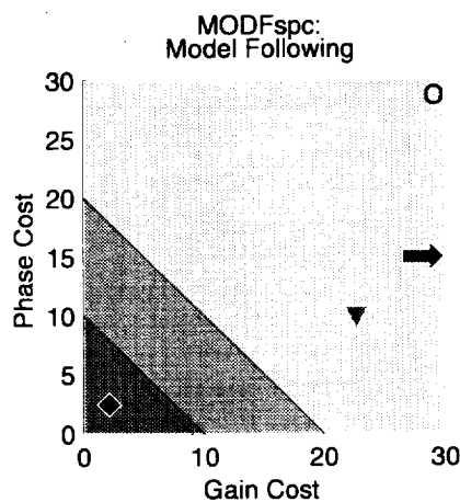
Figure 22. Model following specification for the baseline design parameters.
