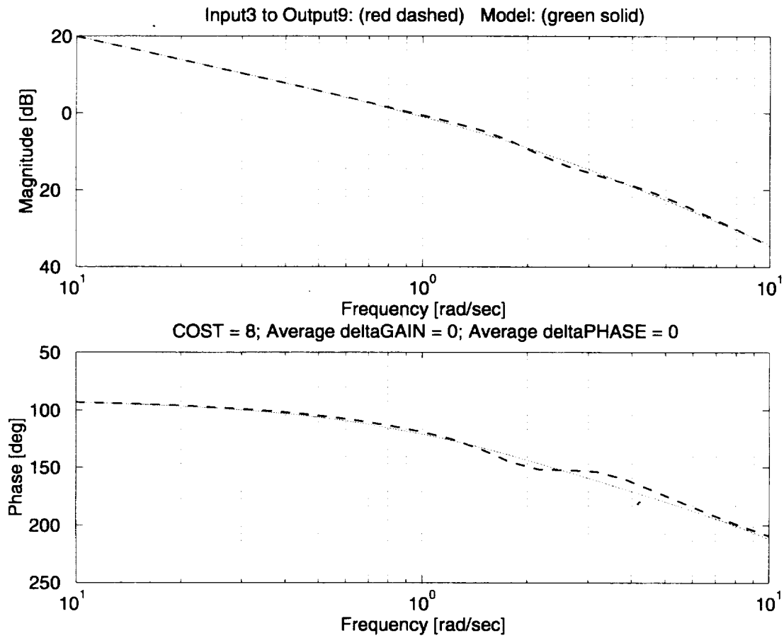
Figure 29. Supporting plot for the model following spec with optimized solution (yaw).
