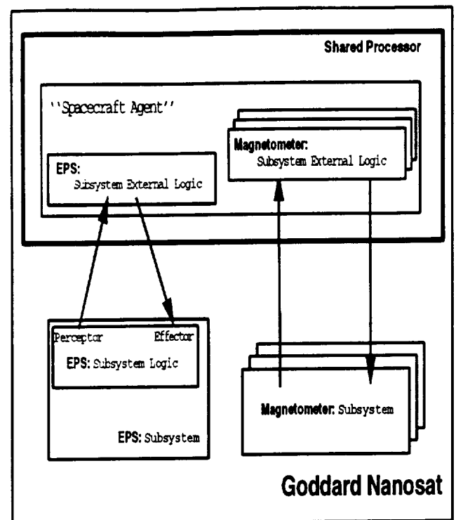
Figure 1. Nanosat EPS control concept.
