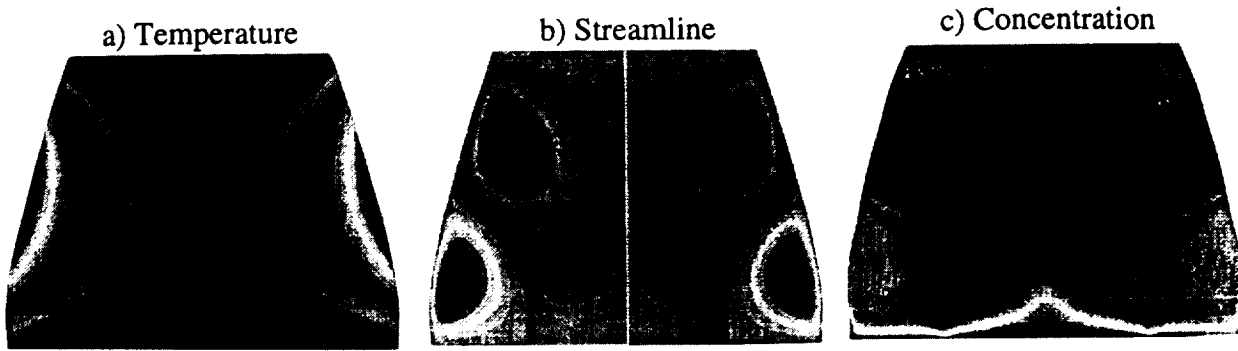
Fig. 6 a) Temperature, b) Flow, and c) Concentration Fields for a Thermocapillary Convection Dominated Case ( Ma = 2.4 , Ra, 2,4(10)^{-4} , Pr=10 , Sc=10,000 ).
