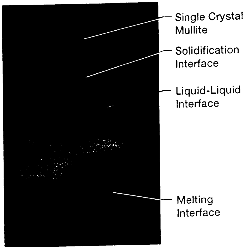
Fig. 2 High Resolution Digital Images Captured During Mullite Crystal Growth
