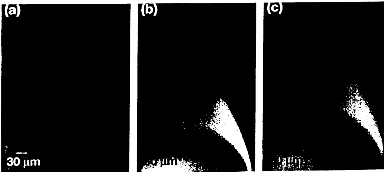
Fig. 3 a) Initiation of Single Crystal Growth, b) Subsequent Occurrence of Large Facets, c) Non-centro-symmetric Position of Crystal Fiber Relative to Melt as a Result of Faceted Growth.
