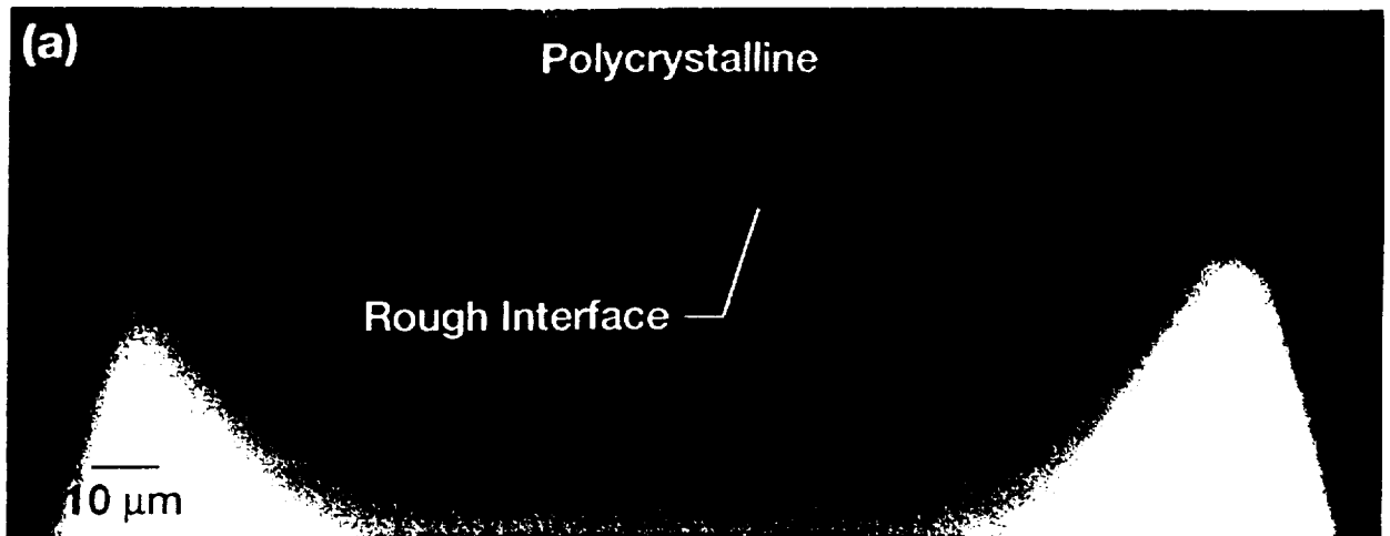
Fig. 4 High Resolution Digital Image of a Rough Domed Liquid-Solid Interface in a Poly-Crystalline Growth.
