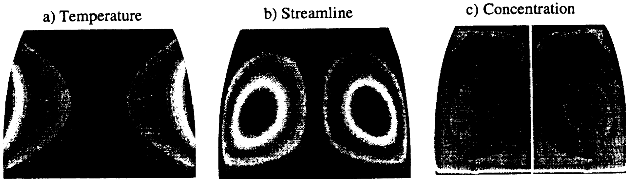
Fig. 7a) Temperature, b) Flow, and c) Concentration Fields for a Natural Convection Dominated Case ( Ma = 2.4 , Ra, 24. , Pr=10 , Sc=10,000 ).
