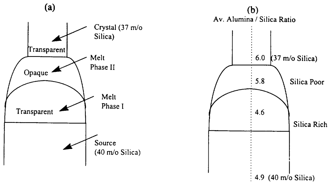
Fig. 1 a) Schematic of Phase-Separated Melt in The Float Zone Setup, and b) Qualitative Alumina/Silica Concentration Map.
