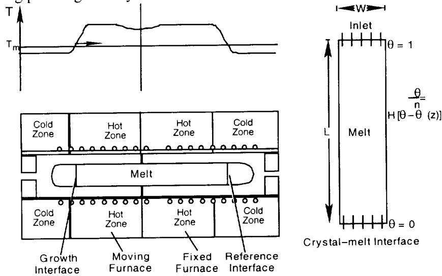
Fig. 1 The MEPHISTO set-up (bottom-left), temperature profile (top left) and computational model (right). T_m denotes the melting temperature.
