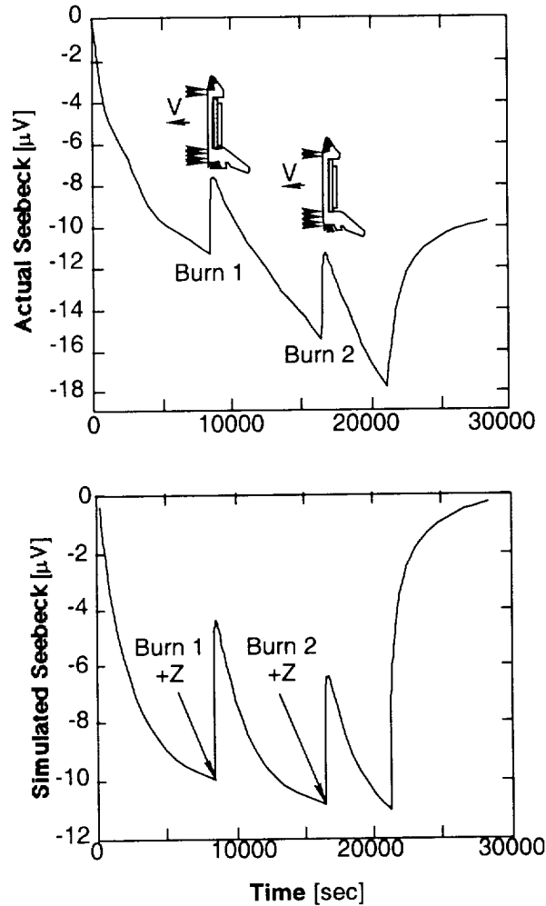
Fig. 2 (a) Actual and (b) predicted Seebeck signal for a 25 second and 15 second burn oriented parallel to the crystal-melt interface.
