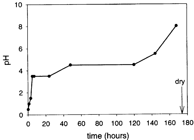
Figure 7. Values of pH over time of HCl solution on AA2024
