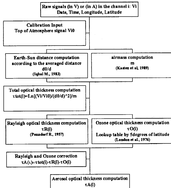
Diagram 2. Sun photometer data processing
