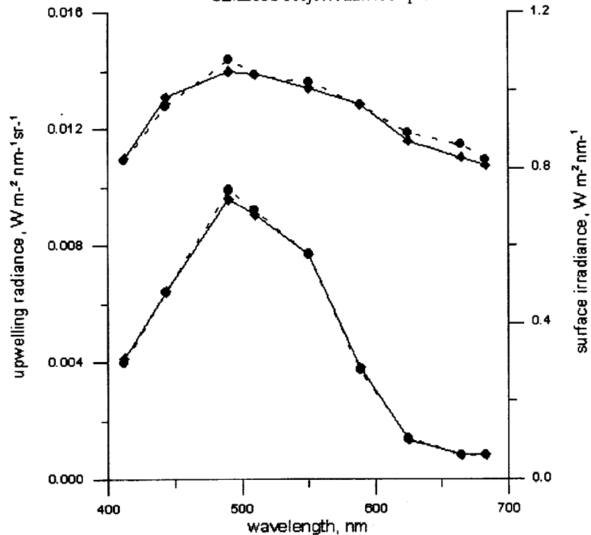
Figure 1. Results of intercalibration between the floating spectroradiometer and MER-2040 at St.2; upper curves - surface irradiance, lower - upwelling radiance; ♦ - floating spectroradiometer, • - MER-2040.
