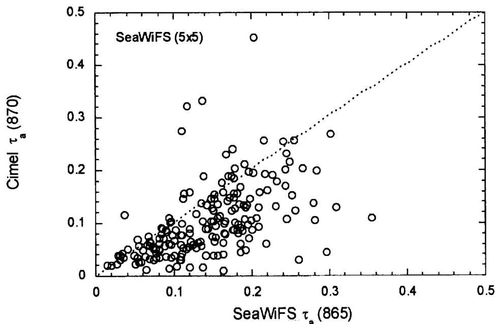
Figure 2. The retrieval SeaWiFS aerosol optical thickness \tau_a(\lambda) compared with the ground in situ measurements from AERONET at 865 nm (870 nm for CIMEL Data).
