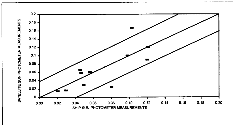
Figure 2. Comparison between satellite and ship derived optical depths (870nm).
