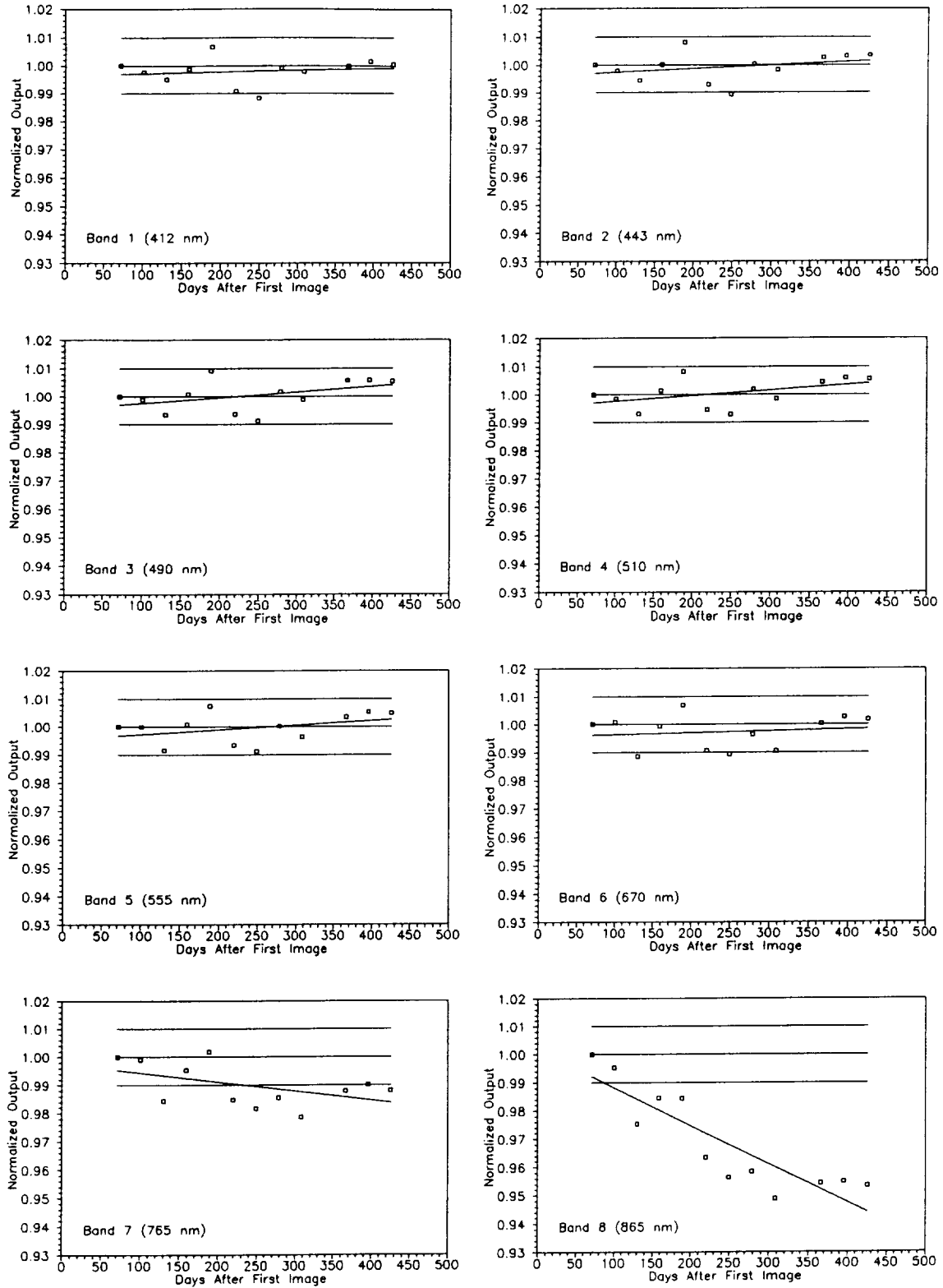
Figure 4. Changes in radiometric sensitivities of the SeaWiFS bands from the lunar measurements. The time series are normalized to unity for the first lunar measurement in November 1997. The horizontal lines with values of 0.99, 1.00, and 1.01 are visual references.
