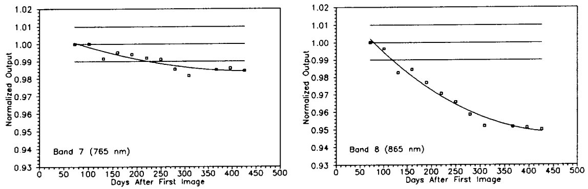
Figure 6. Changes in SeaWiFS bands 7 and 8. The time series for these bands use the modified exponential function from Equation (10).
