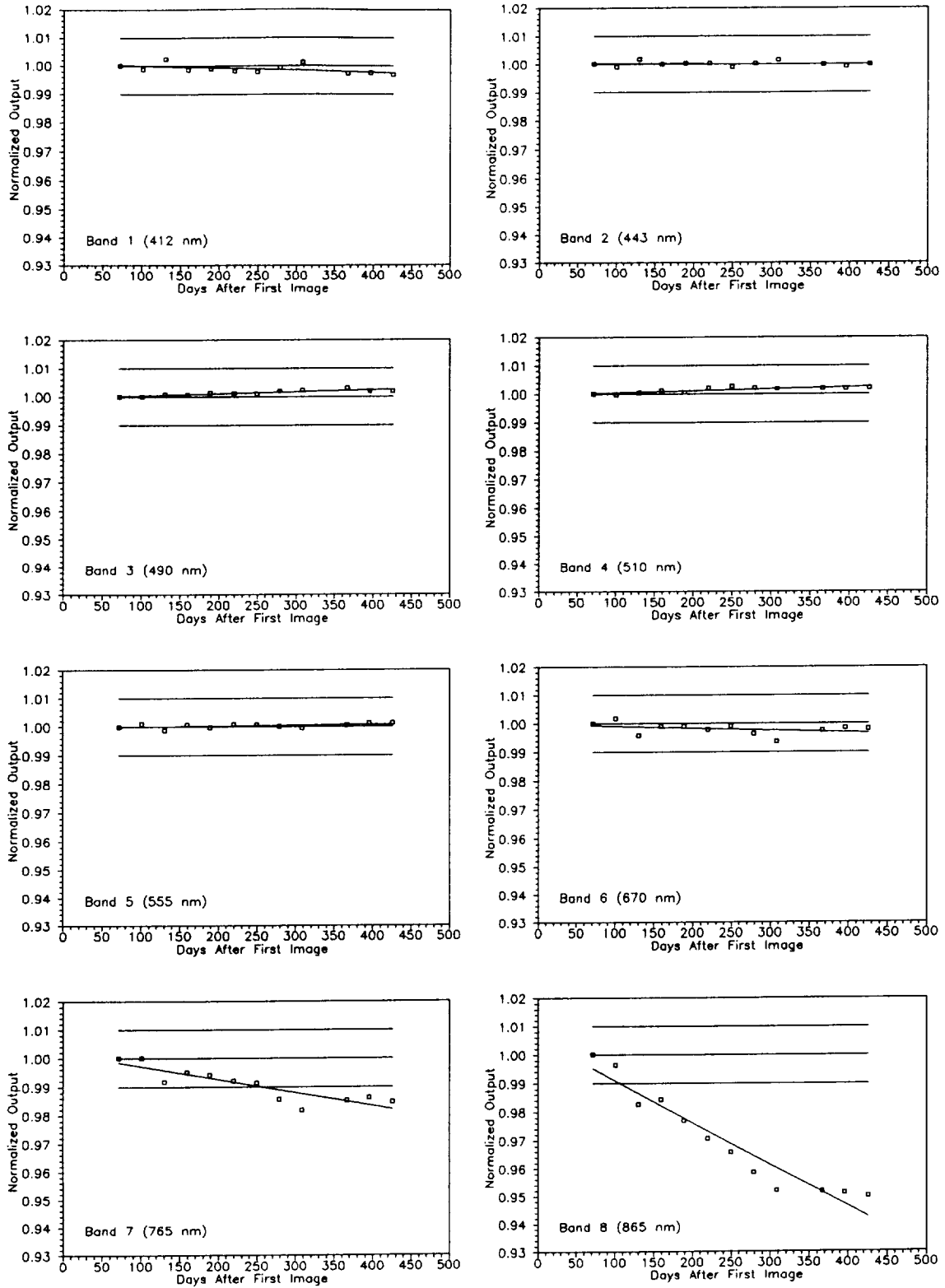
Figure 5. Changes in the SeaWiFS bands after normalization to the average of bands 1 through 6. The scatter of the data points about the trend lines is substantially reduced, compared to Figure 4.
