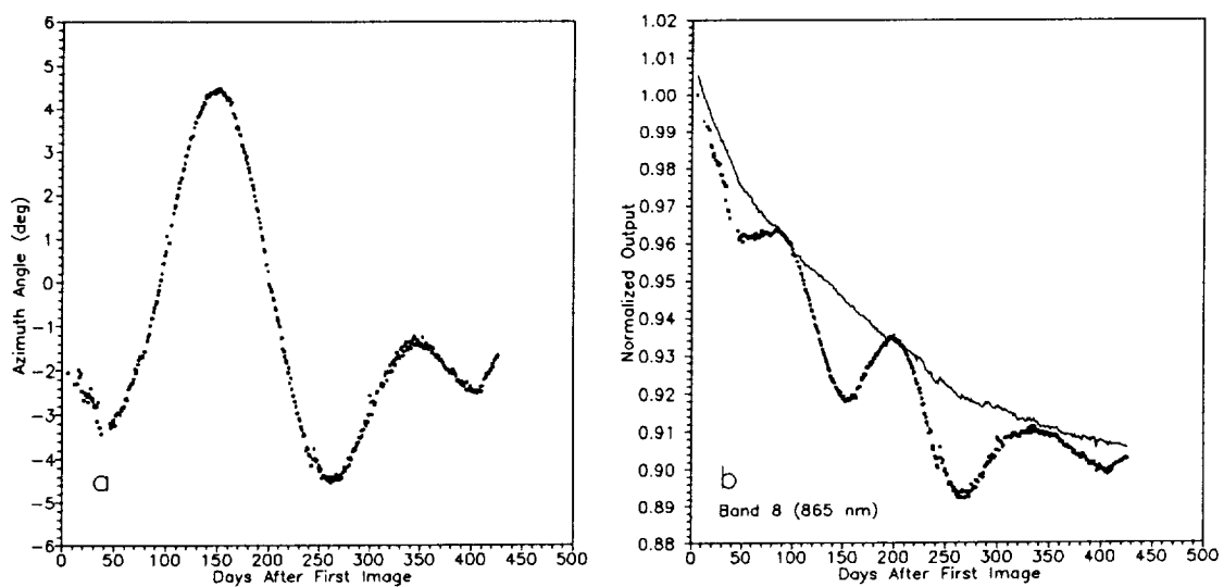
Figure 8. Azimuth angle correction for solar diffuser measurements by SeaWiFS band 8.
