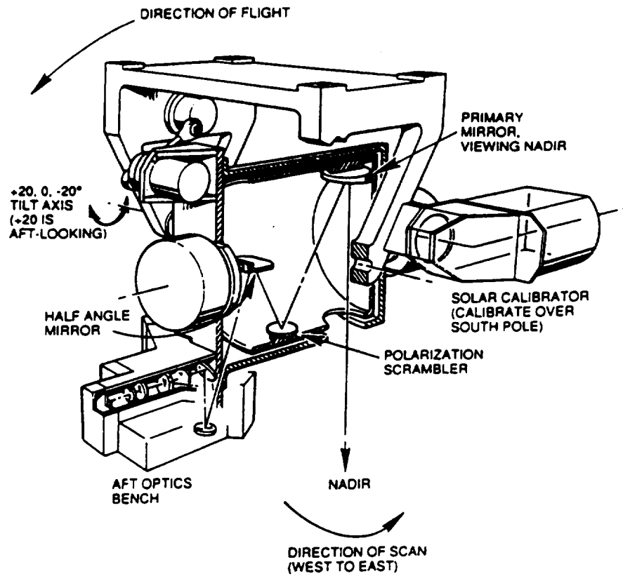
Figure 1. The SeaWiFS scanner assembly. The scanner mounts to the spacecraft using the four mounting points at the top of the figure.
