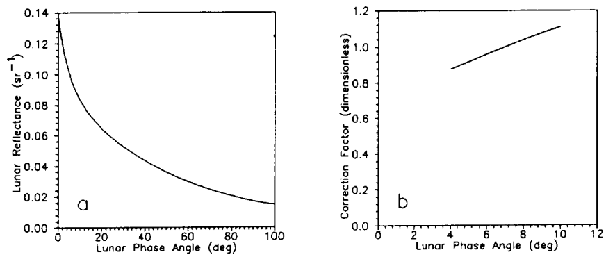
Figure 3. Disk integrated reflectance versus lunar phase angle.
