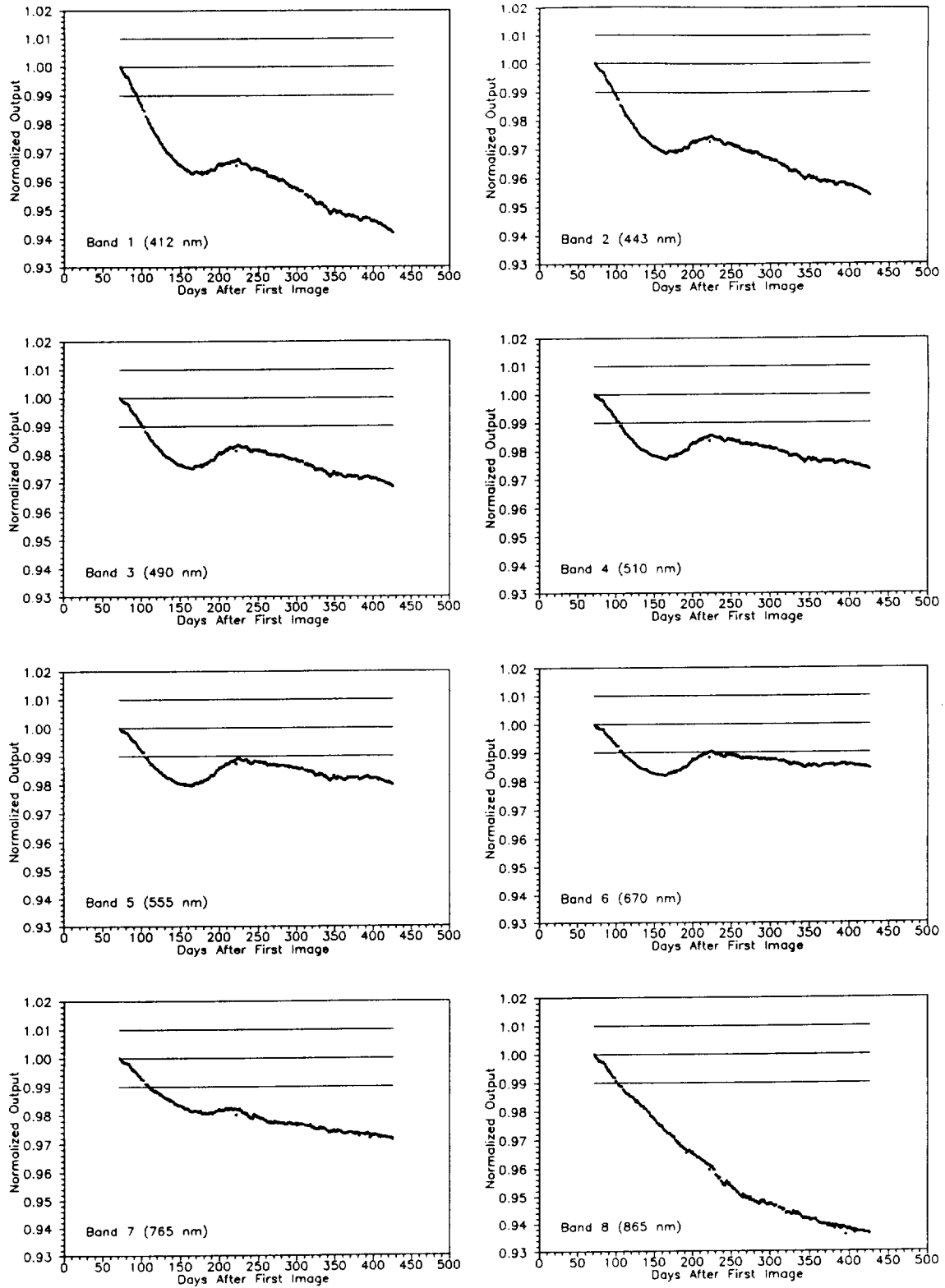
Figure 9. Trends in the solar diffuser measurements for the SeaWiFS bands. There are 356 measurements in each panel. The format for this figure duplicates that for Figures 4 and 5.
