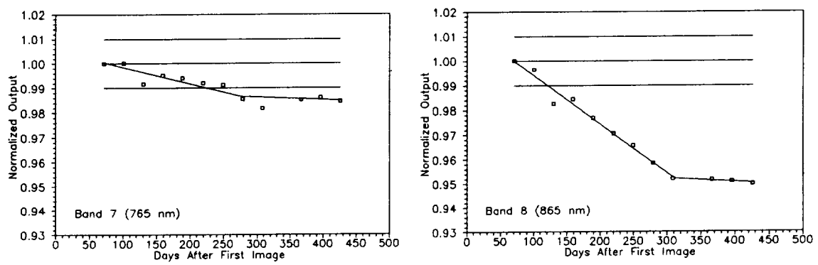
Figure 7. Two piece linear fits to the lunar-based trends for SeaWiFS bands 7 and 8.
