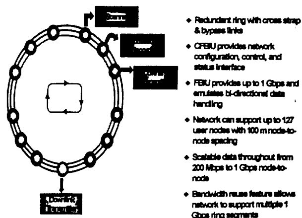
Figure 1. SFODB Fiber Optic Network
