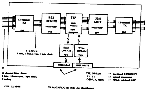
Figure 5. Parallel SFODB Block Diagram - FBIU
