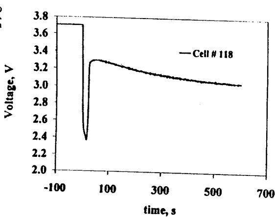
Delay at 100 mA at -40 C
