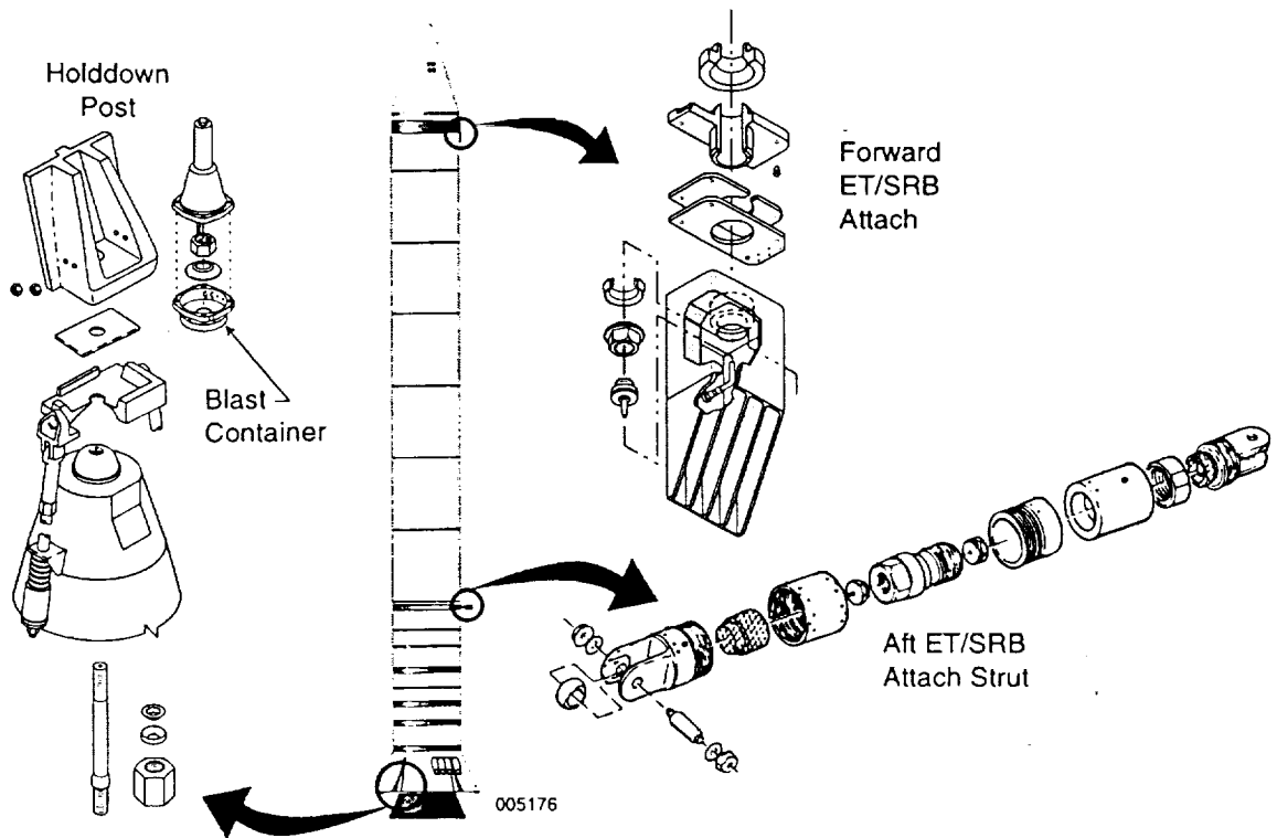
Figure 2. Solid Rocket Booster with Blast Container
