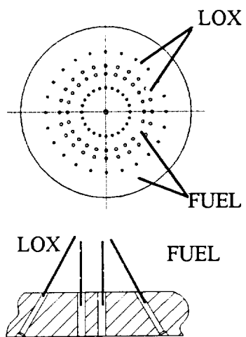
Figure 2: Split Triplet Injector (F-OO-F) (a) Injector Face, (b) Injection Element
