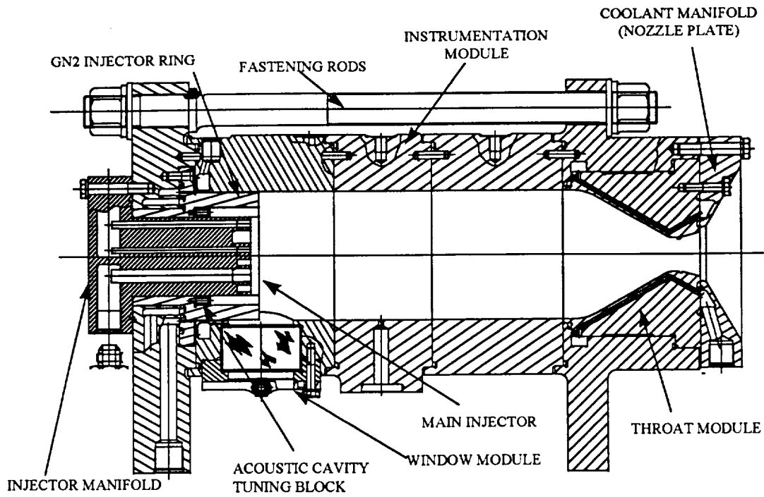
Figure 1: MCTA with an Injector Assembly
