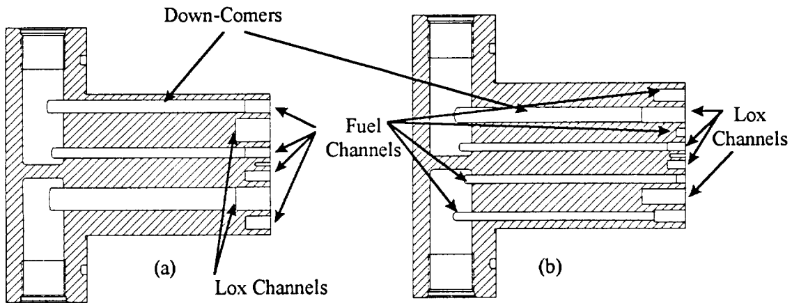
Figure 5: Injector Cores of Impinging Injectors, (a) Unlike-Doublet (F-O-F-O) (b) Split-Triplet (F-OO-F) and Unlike-Doublet (F-O-O-F)
