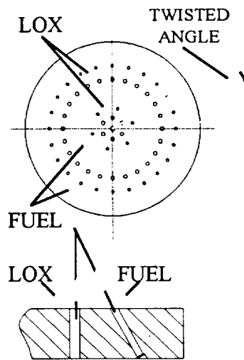
Figure 3: Unlike doublet Injector (F-O-F-O) (a) Injector Face, (b) Injection Element
