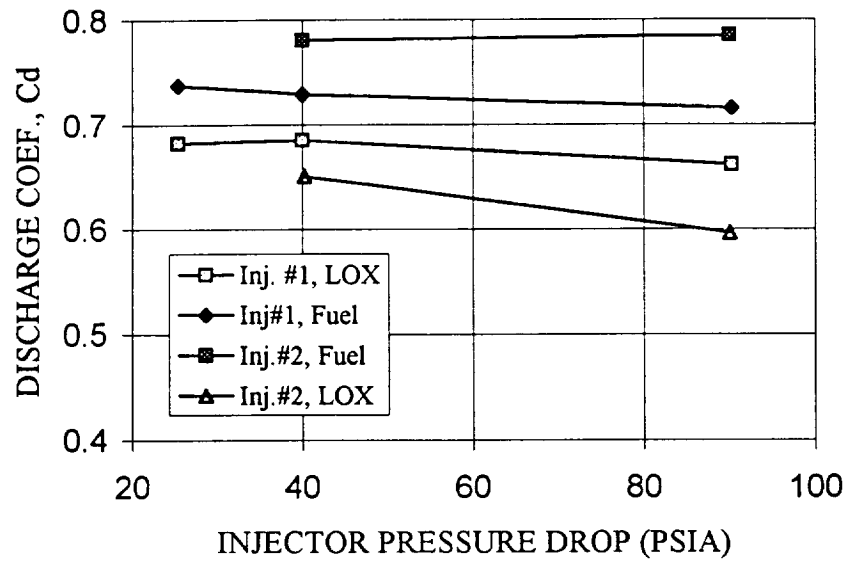
Figure 4: Injector Discharge Coefficients of Injector # 1 (Split-Triplet) and Injector # 2 (Unlike-Doublet)
