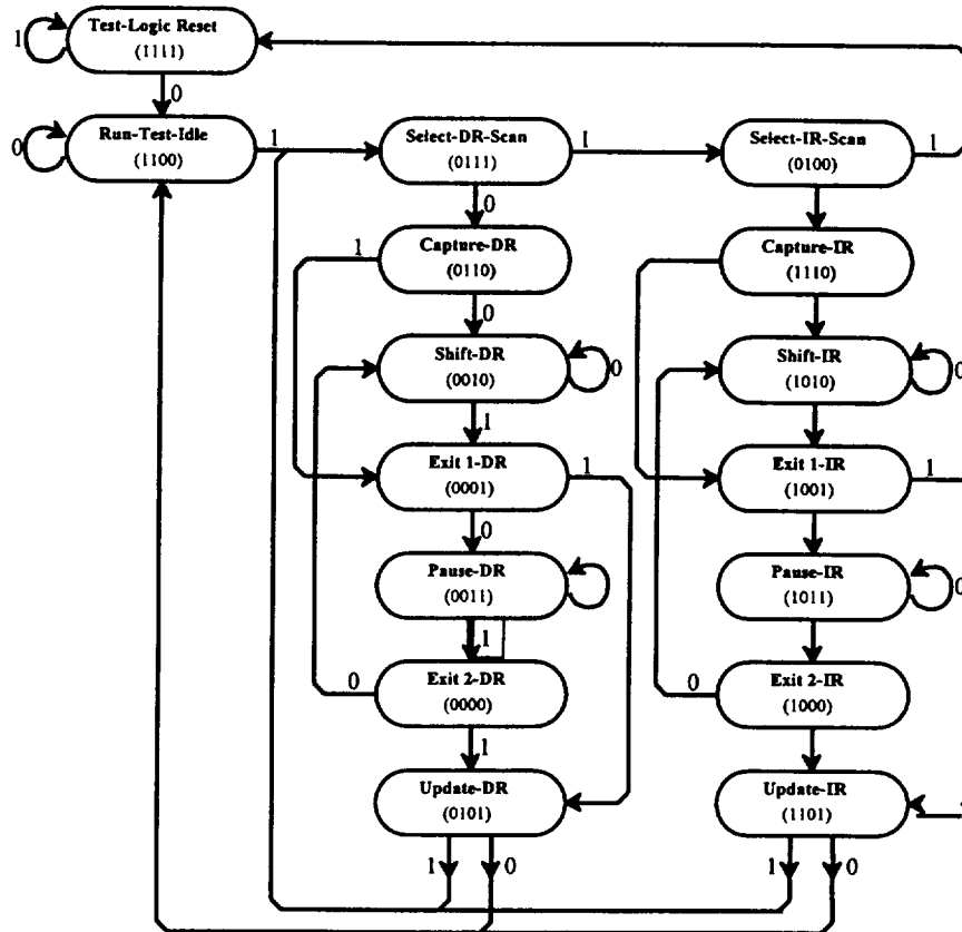
Figure 4: TAP Controller State Diagram
