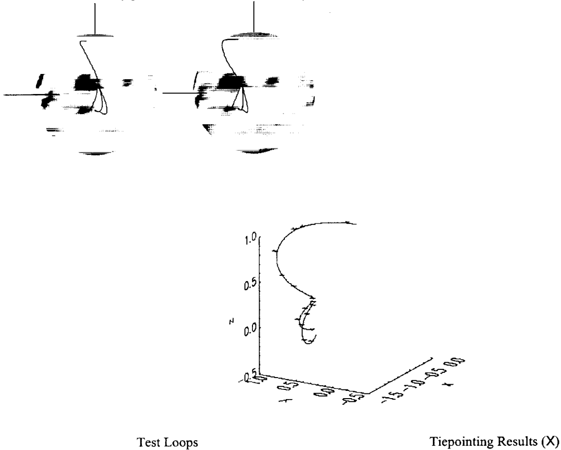
Fig. 2. Test of determination of 3D loop geometry on known loops. The test stereo image pair (top) was created by viewing the known loops from two angles separated by 15° (This pair may be viewed in stereo by relaxing your eye focus). The (x,y,z) location of points (X's) determined by triangulation from the stereo pair are plotted over the known test loops (solid curves). Agreement is excellent.
