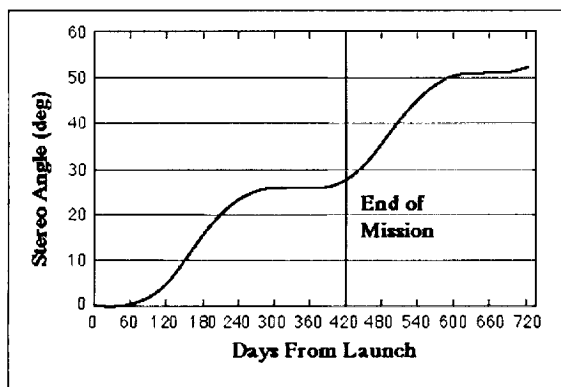
Fig. 4 (old 7-1_ : SXCI Spacecraft
