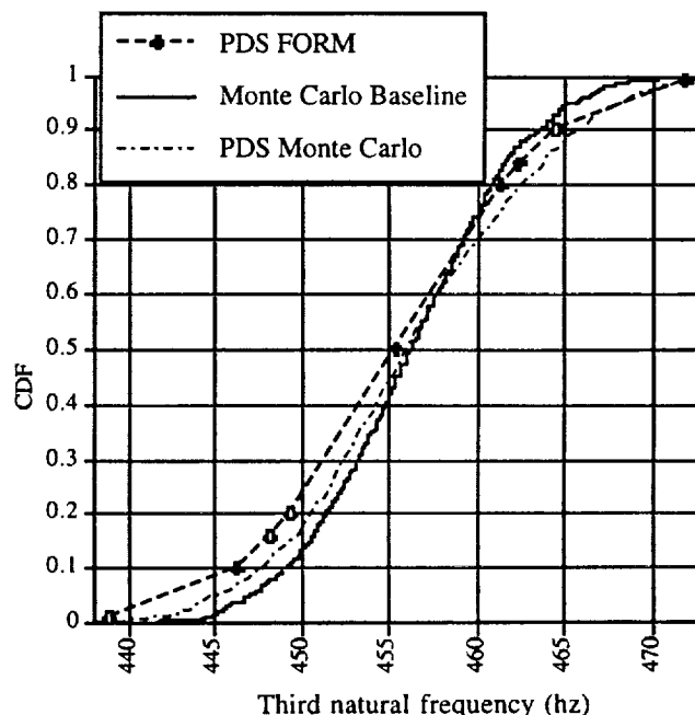
Figure 3 Two bladed-disk mode 3 natural frequency comparing Monte Carlo with PDS
