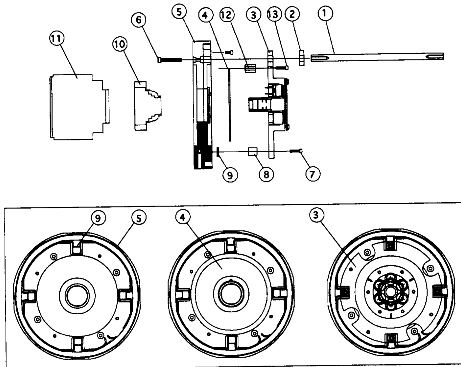
Fig. 7. Engineering assembly drawing of the ATA. The parts labeled 1-13 correspond to the 1) support rod, 2) plastic spacer, 3) DPA, 4) amplifier circuit board, 5) ambient temperature plate, 6) 6-32×19 mm fasteners, 7) 6-32×12 mm fasteners, 8) thermal conductors, 9) TEC, 10) F-to-C mount adaptor, 11) objective lens, 12) Delrin spacer, and 13) 6-32×25 mm fasteners (nylon). The bottom three smaller drawings indicate some of the interior components in greater detail.
