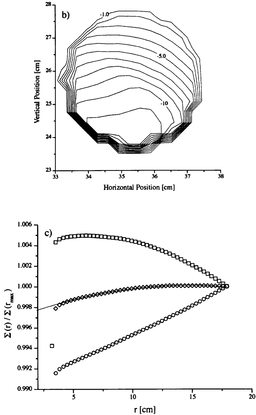
Fig. 17. (cont.) Relative spatial responsivity, h(x,y) , for channel 2 of the SXR, which was on gain 1,000. b) A contour plot of data, in 1V increments, to illustrate the in-field response. The non-uniformity within the field of view is because of vignetting. c) The normalized and integrated net signals are determined using a background of \langle b \rangle = -6.440 mV. The area used for the normalization was 35.84 cm square. The open diamonds, squares, and circles correspond to \langle b \rangle , b_- ( -6.943 mV), and b_+ ( -5.398 mV), respectively. The solid line is a quadratic fit to the normalized sums using \langle b \rangle for r > 4.16 cm.
