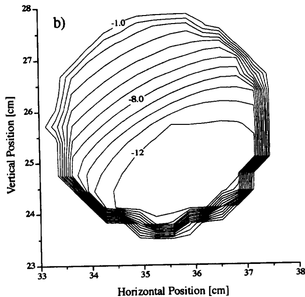
Fig. 16. Relative spatial responsivity, h(x, y) , for channel 1 of the SXR, which was on gain 100. a) A contour plot of data, in non-uniform increments, to emphasize the out-of-field response. The increments between the contours in the out-of-field region are 2.2 mV, 1.5 mV, and 1.1 mV. b) A contour plot of data, in 1 V increments, to illustrate the in-field response. The non-uniformity within the field of view is because of vignetting.
