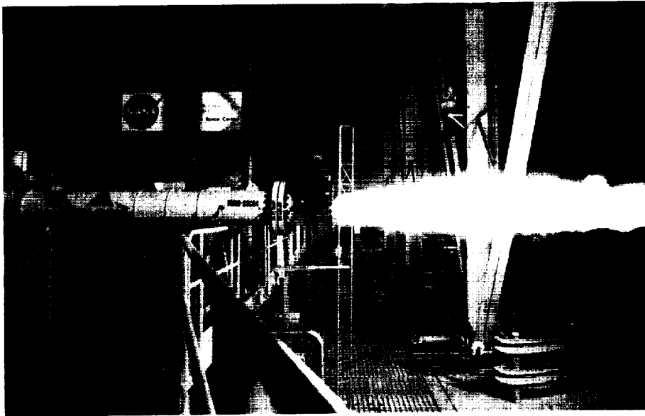
The test-firing of a commercial hybrid rocket motor is one example of Stennis Space Center's partnership with private companies for propulsion development testing. A 10,000-pound-thrust hybrid rocket motor undergoes a test-firing in 1994 at Stennis Space Center's E-1 test Facility. The E-1 Test Facility shown above was formerly known as the Component Test Facility. (SSC-94-707-6)
