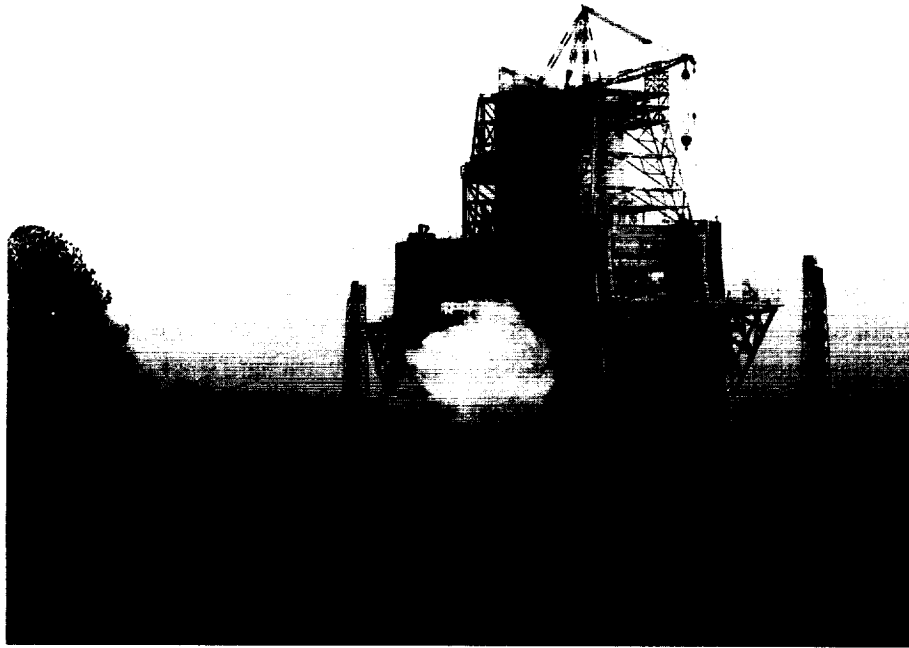
NASA's John C. Stennis Space Center in Hancock County, MS, flight certifies all of the main engines that help power the Space Shuttle into Earth's orbit. Shown on the "B" stand, B-1 test position, is a static firing of a Space Shuttle Main Engine. One of the many tame deer, which share the SSC environment, studies a "common place" test-firing. (SSC-96-129-15)
