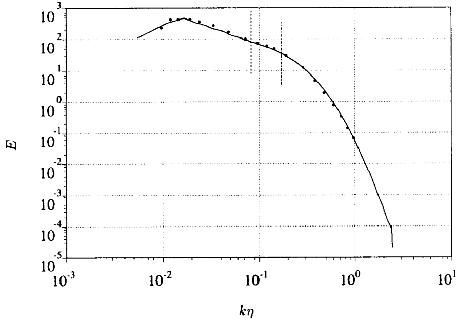
FIGURE 2. Spectrum of the 512^3 DNS ( Re_\lambda = 63.5 ). Also shown are the cuts used to produce the 64^3 and 32^3 synthetic LES fields. \bullet : Comte-Bellot and Corrsin experimental data at Re_\lambda = 65.1 . k normalized by Kolmogorov scale \eta .
