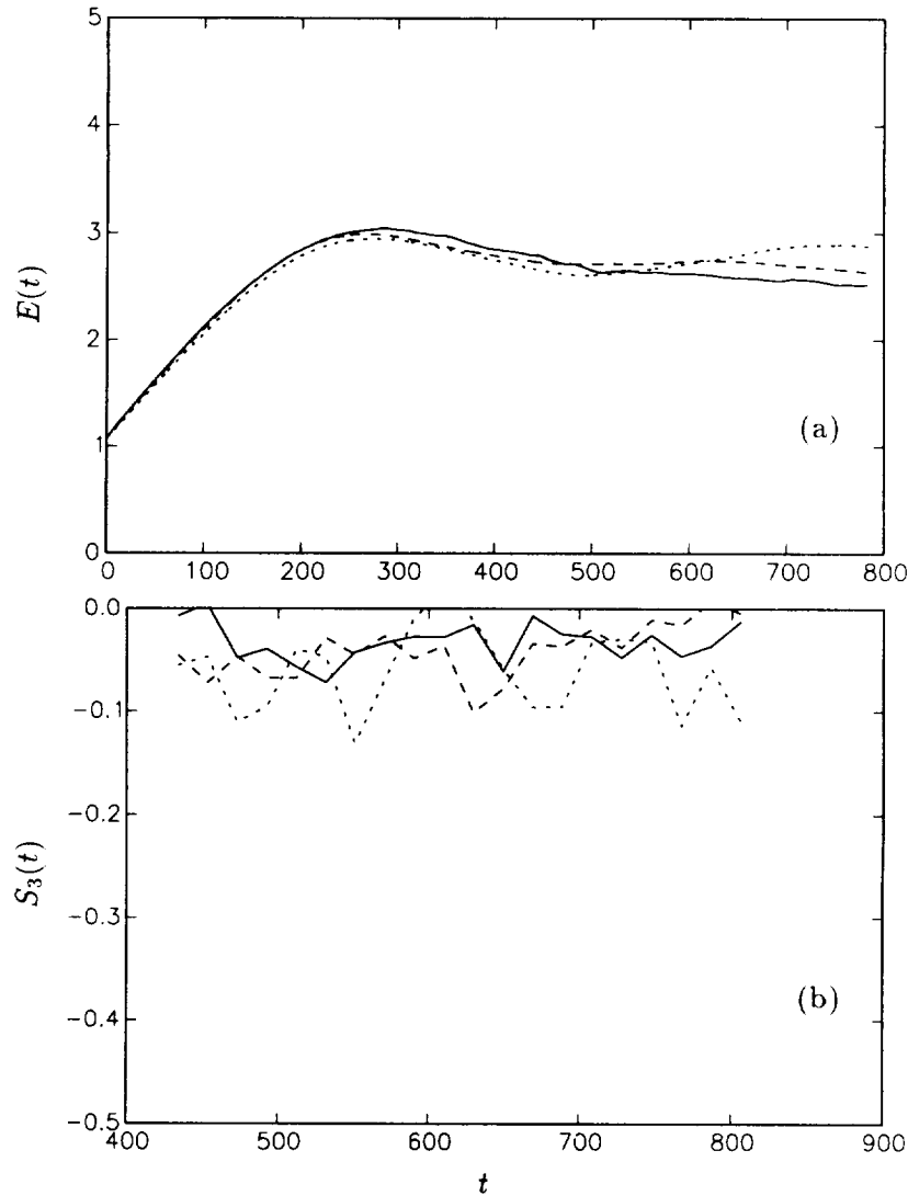
FIGURE 4. Eddy-viscosity models on pencil-like grid ( 128 \times 128 \times 16 ). (a) energy as a function of time for dynamic model (—), modified Smagorinsky (⋯⋯) and Smagorinsky-Deardoff (----). (b) derivative skewness in the worst resolved direction, same symbols as above.
