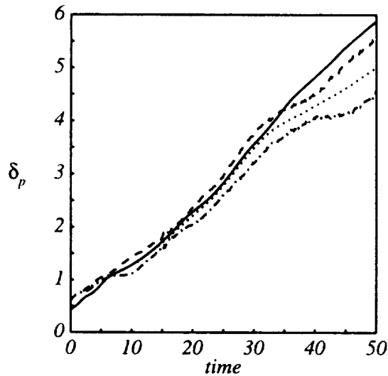
FIGURE 3. Product thickness for S = 1 (—; not affected by the asymmetry) and for S = 8 (---) and 1/8 (----), corresponding to a flip experiment, for \epsilon = 0.45 , Re = 500 and Pr = 1 . ..... : common value for S = 8 and 1/8 when \epsilon = 0 .
