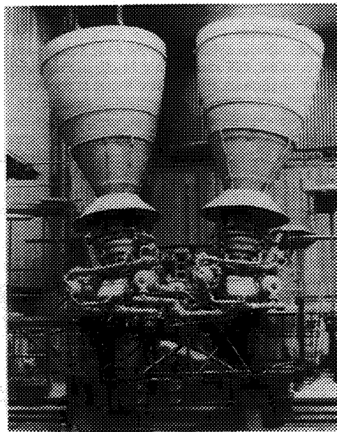
Fig. 7 RD-701 dual-fuel engine mock-up.
