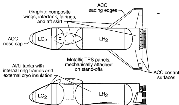
Fig. 4 SSV material assumptions.
