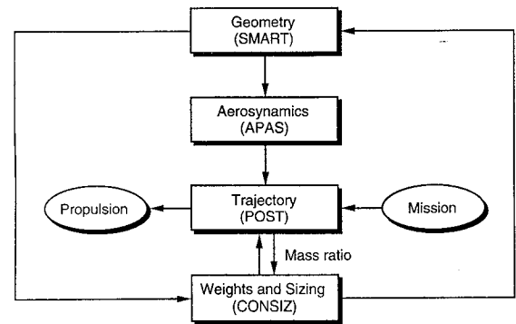
Fig. 1 AMLS vehicle design process.
