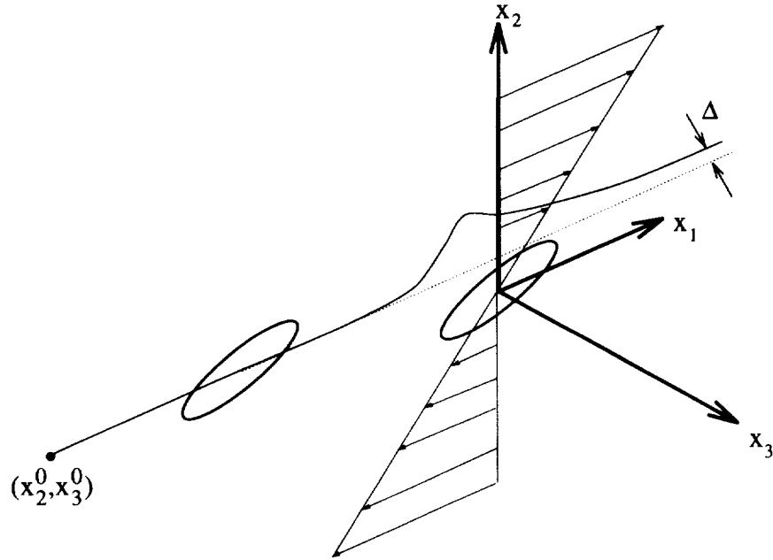
Figure 1: Schematic of relative trajectory between pair of deformable interacting drops in shear flow.
