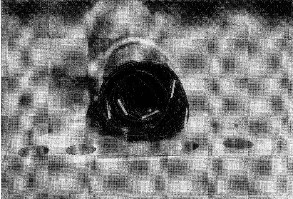
Figure 6. Development Unit Stowed Package with Wrap Discontinuities.
