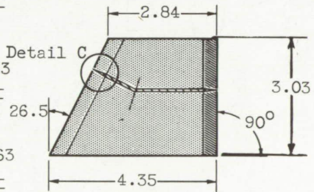
Fin C; fin area, 10.88; aspect ratio, 1.69.
