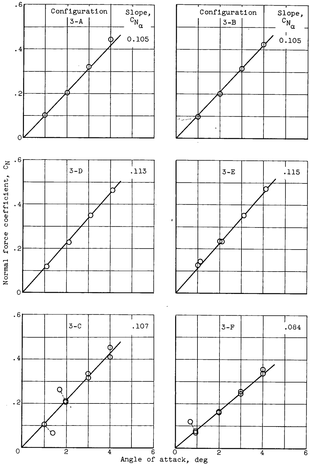
(c) Tested with nose 3.
