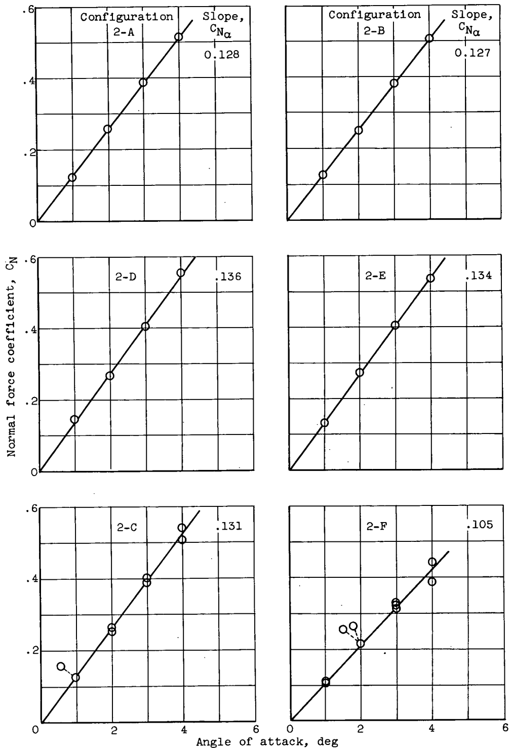
(b) Tested with nose 2.
