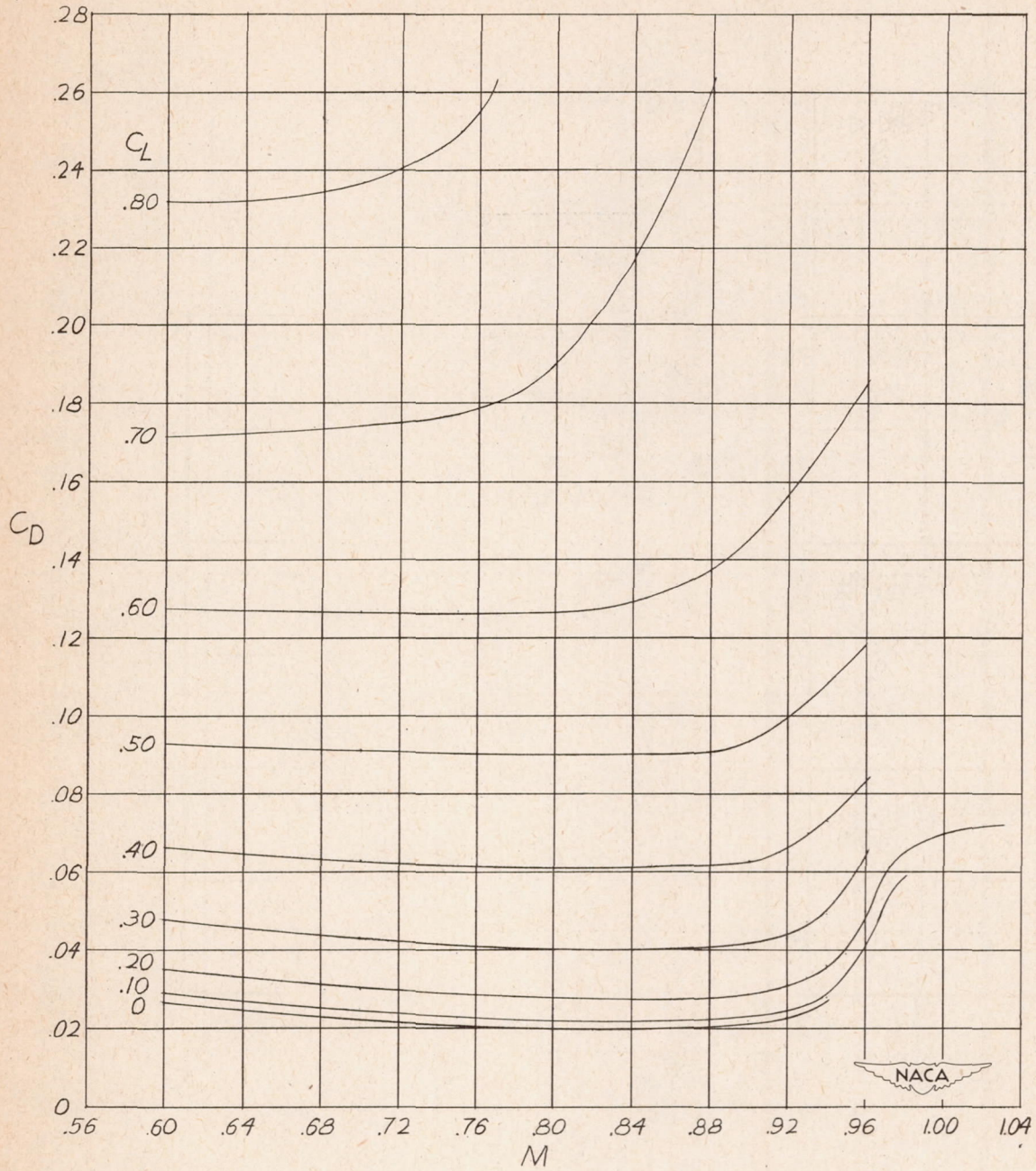
Figure 9.- Variation of drag coefficient with Mach number for various constant lift coefficients.
