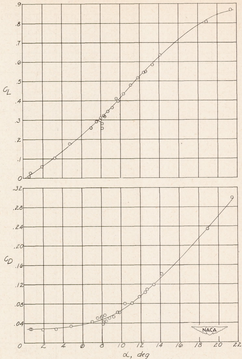
(a) M = 0.60 .
