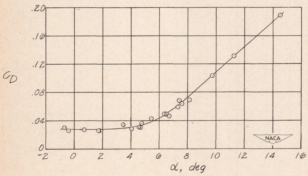
(h) M = 0.93 .
