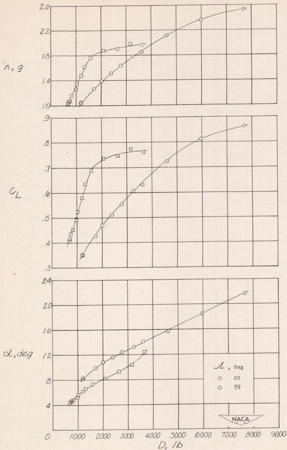
Figure 13.- Comparison of performance of 20^\circ and 59^\circ sweptback configurations in pull-ups at a Mach number of 0.74 and an altitude of 42,000 feet.
