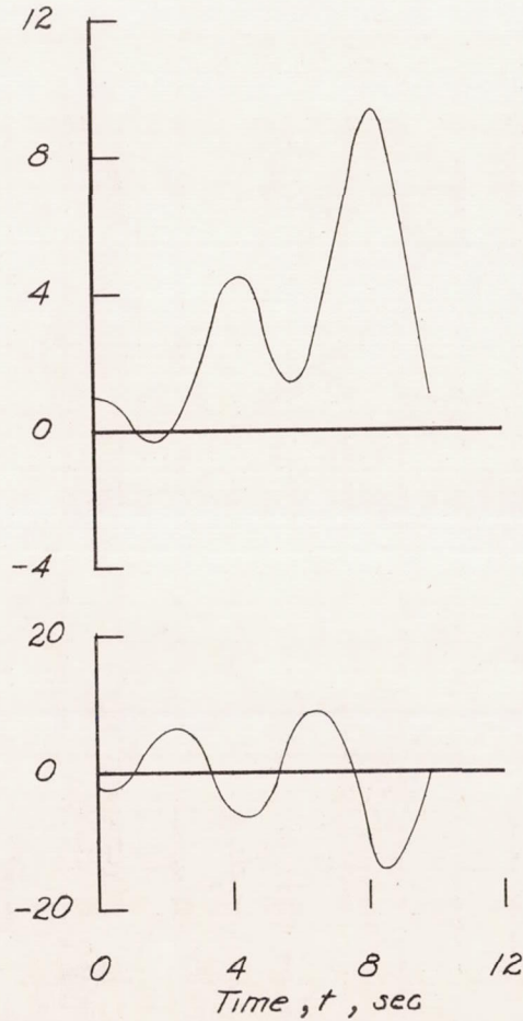
(a) Without autopilot.
