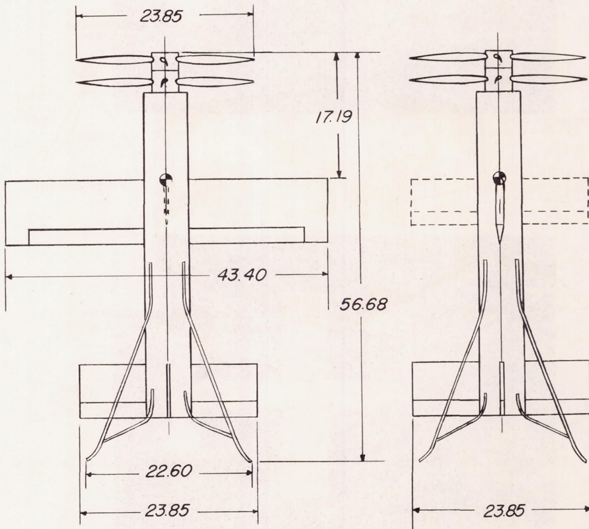
Figure 3.- Vertically rising airplane model showing the important dimensions. All dimensions in inches.
