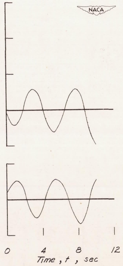
(b) With autopilot \frac{\delta_e}{\theta} = 2 .
