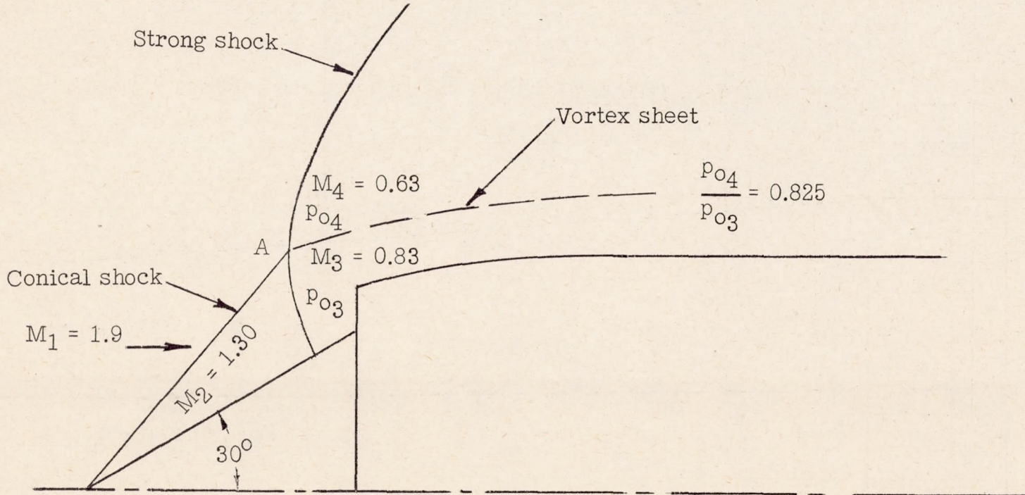
Figure 4.- Aerodynamic phenomena of an inlet having a 30° cone-angle central body for subcritical conditions at M = 1.90.
