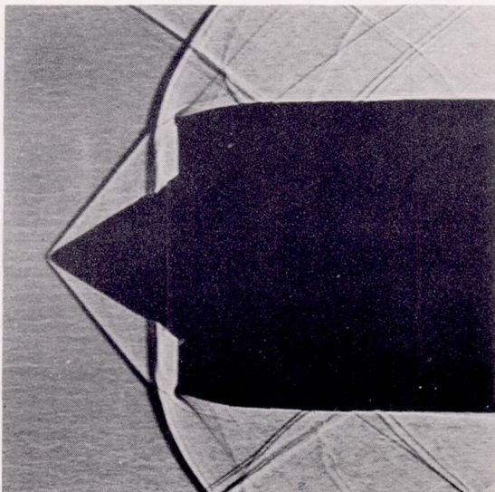
(c) \frac{A_1}{A_2} = 0.72 .
