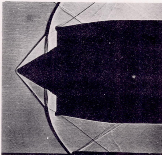
(c) 30^\circ -0.907 central body; cowling C;
