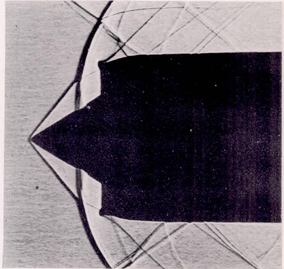
(b) 30^\circ -1.10 central body; cowling D;
