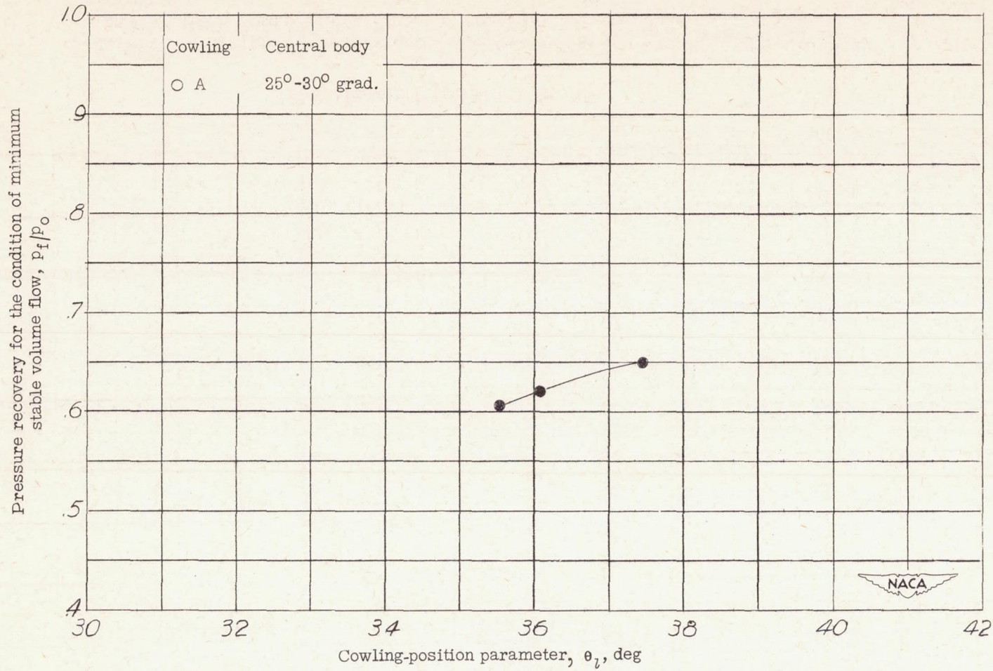
Figure 62.- Pressure recovery of inlets having 25^\circ-30^\circ-1.10 central body as a function of the cowling-position parameter at M = 2.70 .
