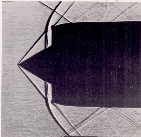
(b) \frac{A_1}{A_2} = 0.81 .
