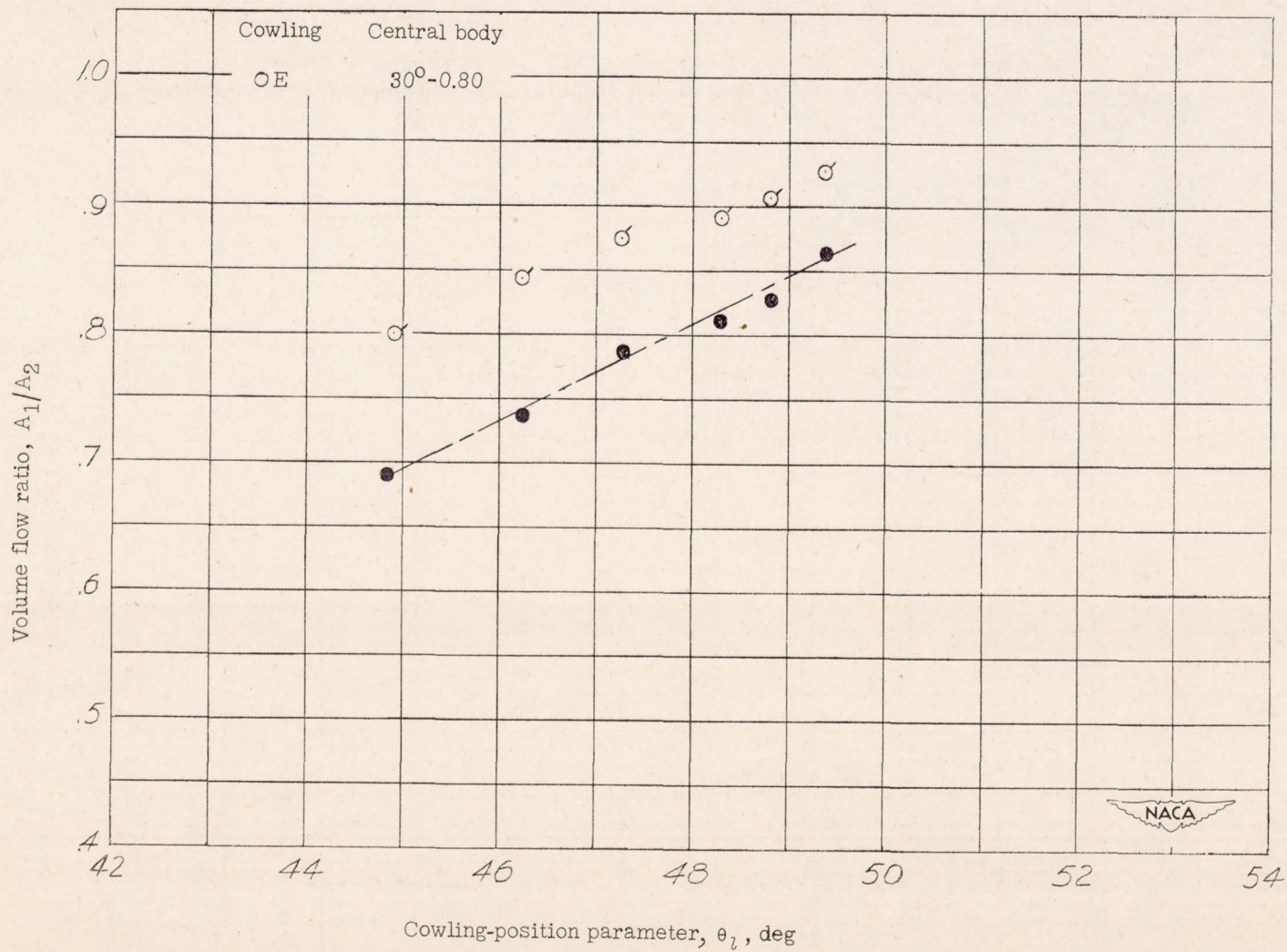
Figure 31.- Volume-flow regulation of inlets having 30^\circ cone-angle central bodies as a function of the cowling-position parameter for \alpha = 8^\circ 30' at M = 1.90 .
