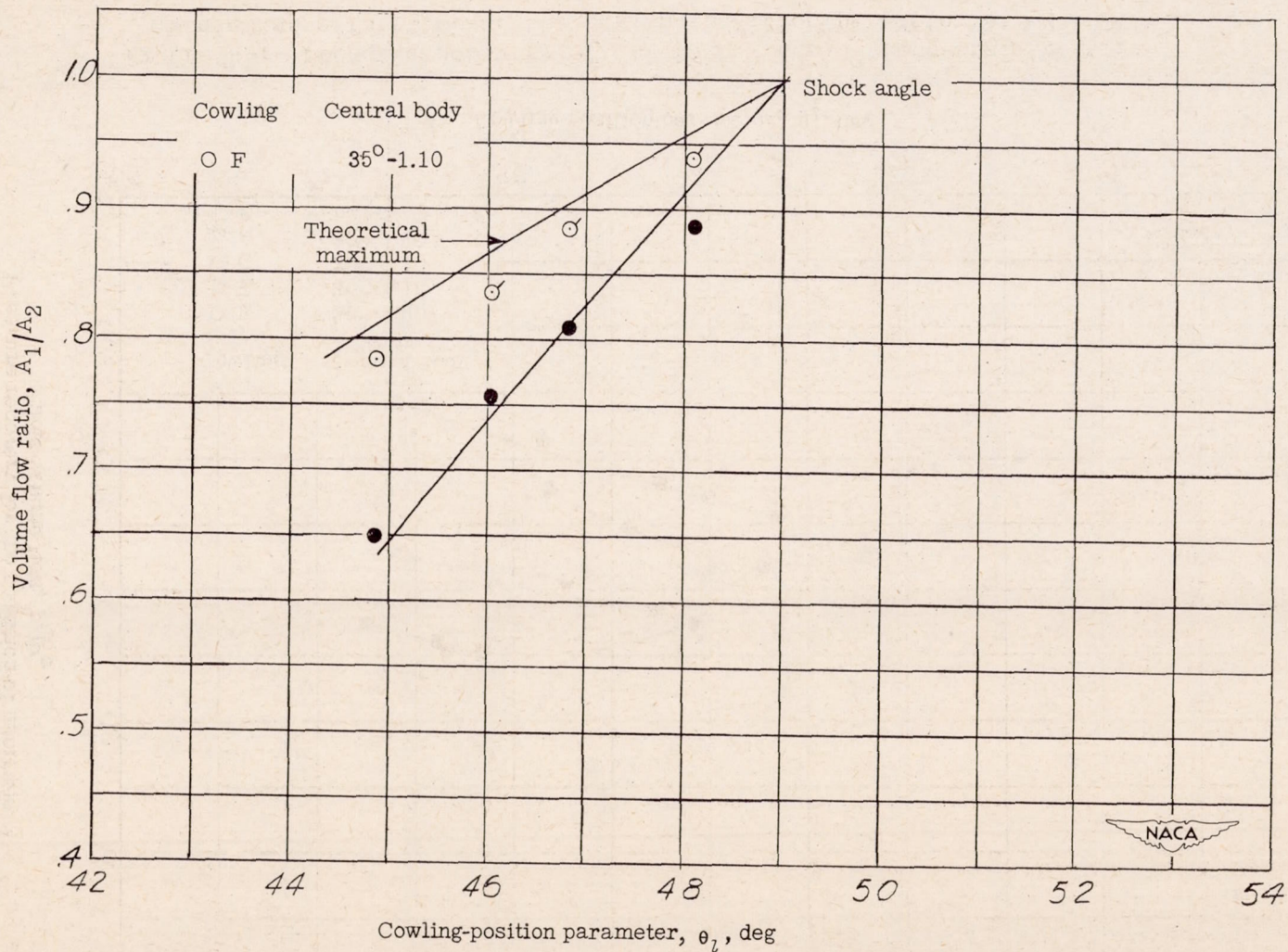
Figure 45.- Volume-flow regulation of inlets having 35^\circ cone-angle central bodies as a function of the cowling-position parameter at M = 2.46 .
