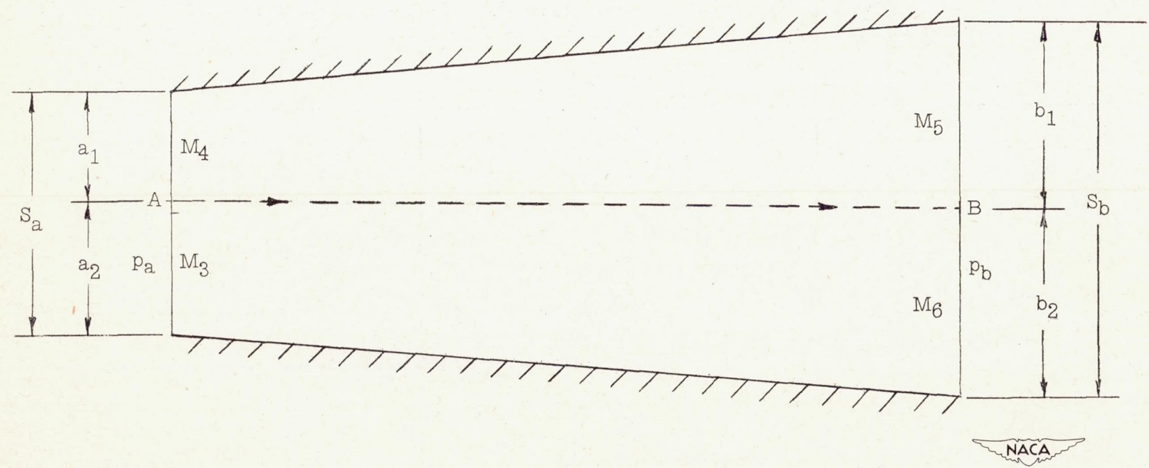
Figure 5.- Subsonic diffusers having two layers of flow having different entropies.
