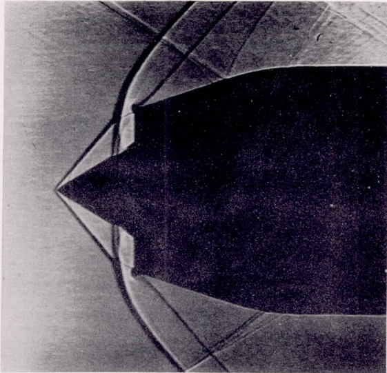
(a) 30^\circ -0.80 central body; cowling E;
