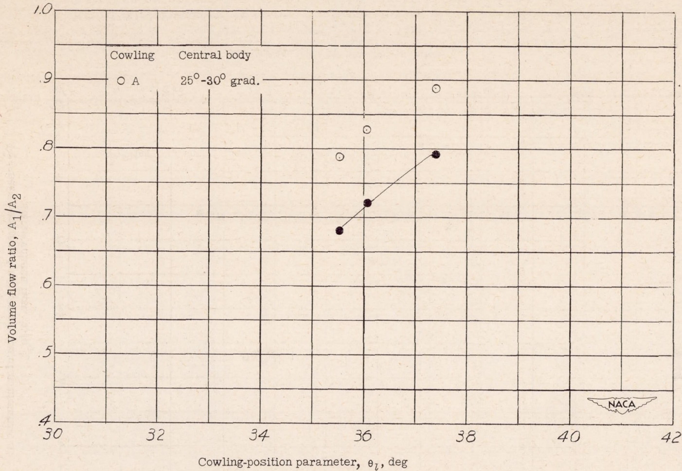
Figure 61.- Volume-flow regulation of inlets having 25°-30°-1.10 body as a function of the cowling-position parameter at M = 2.70 .
