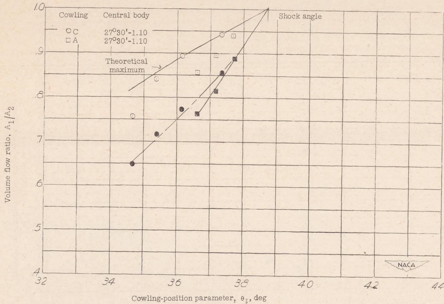
Figure 53.- Volume-flow regulation of inlets having 27^\circ 30' cone-angle central bodies as a function of the cowling-position parameter at M = 2.70 .
