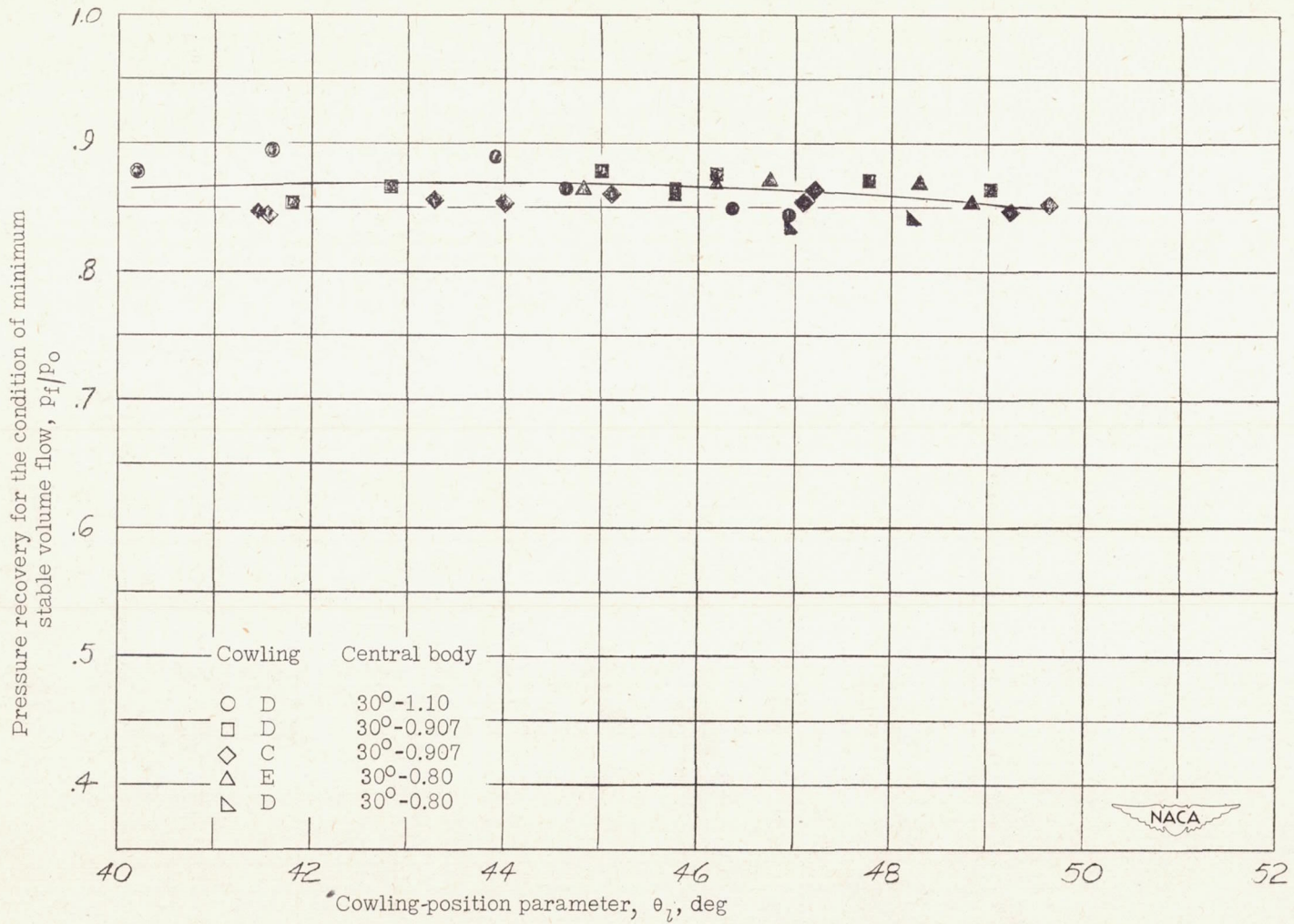
Figure 30.- Pressure recovery of inlets having 30^\circ cone-angle central bodies as a function of the cowling-position parameter at M = 1.90 .
