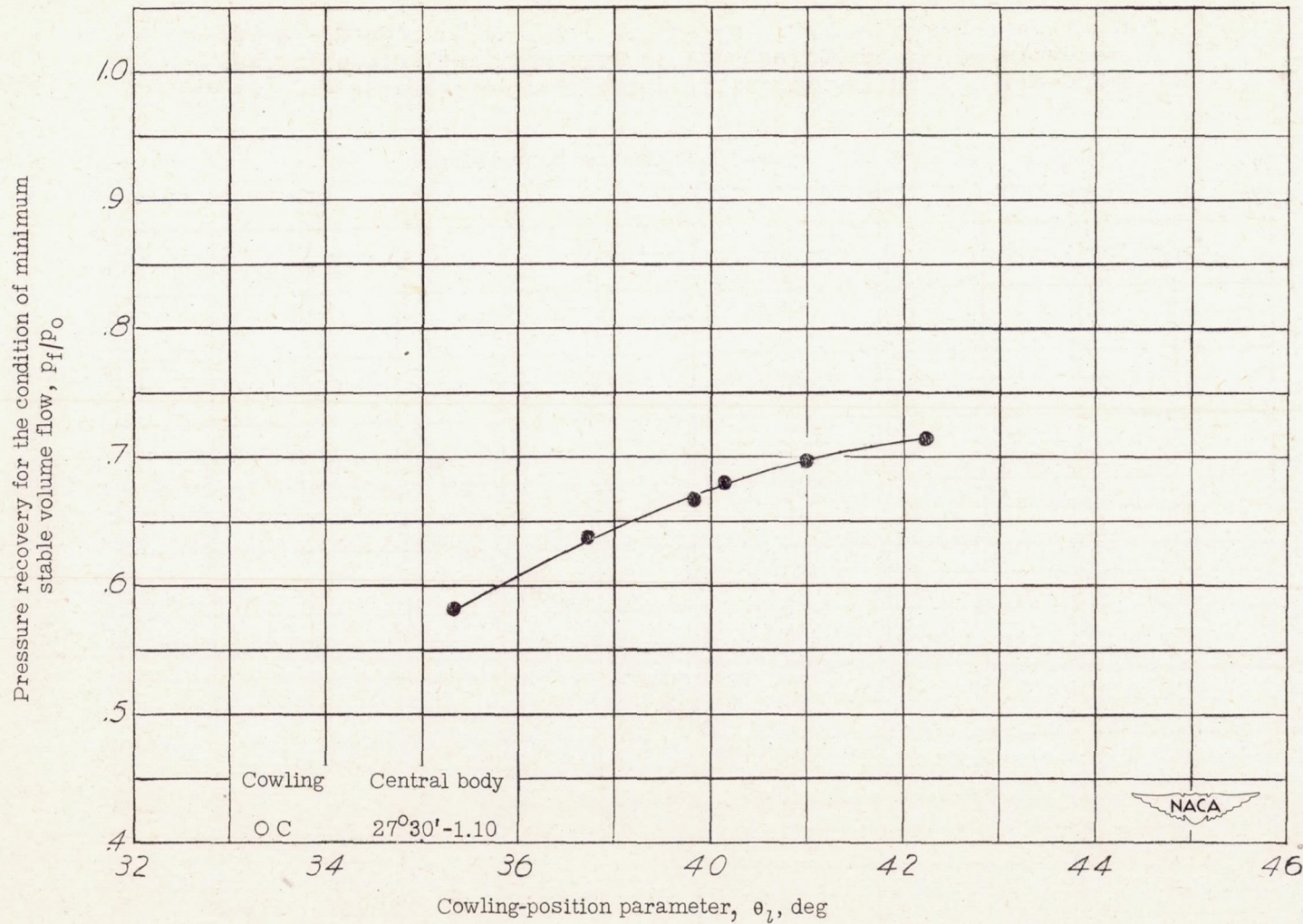
Figure 42.- Pressure recovery of the inlets having 27^{\circ}30' cone-angle central bodies as a function of the cowling-position parameter at M = 2.46 .
