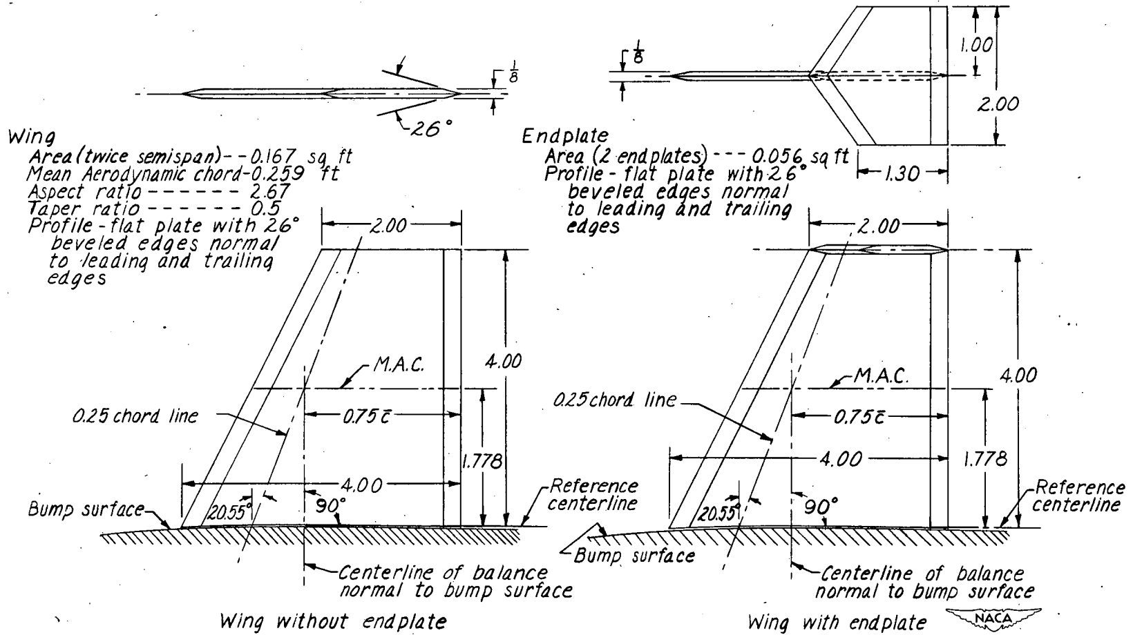
Figure 1.- General arrangement of the two wings swept back 20.55°, one wing with and one wing without an end plate. (All dimensions are in inches unless otherwise noted.)
