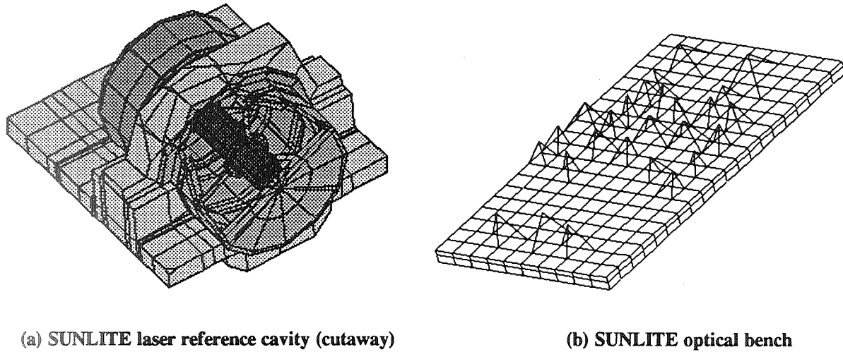
Figure 4. PATRAN models used for both thermal and structural analysis
