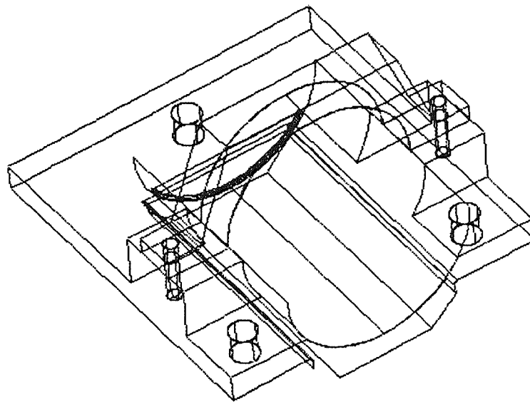
Figure 2. Mount part imported to PATRAN from ProEngineer through IGES file
