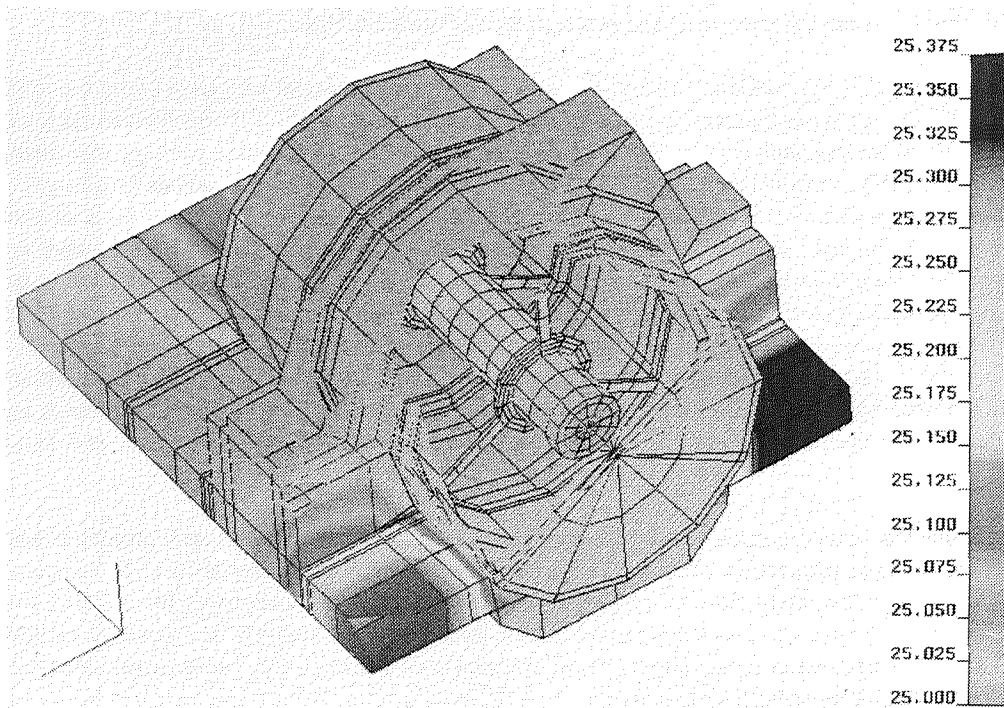
Figure 5. Map of thermal distribution (in degrees C) on laser reference cavity in PATRAN
