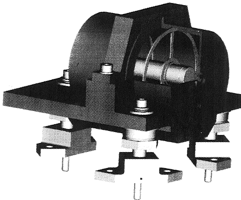
Figure 1. Laser reference cavity as designed and portrayed in Pro-Engineer
