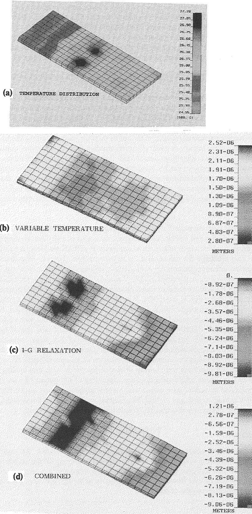
Figure 6. SUNLITE optical bench with progressive mappings: (a) thermal distribution, (b) thermally-driven deflections, (c) mechanical load-driven deflections, and (d) summed deflections
