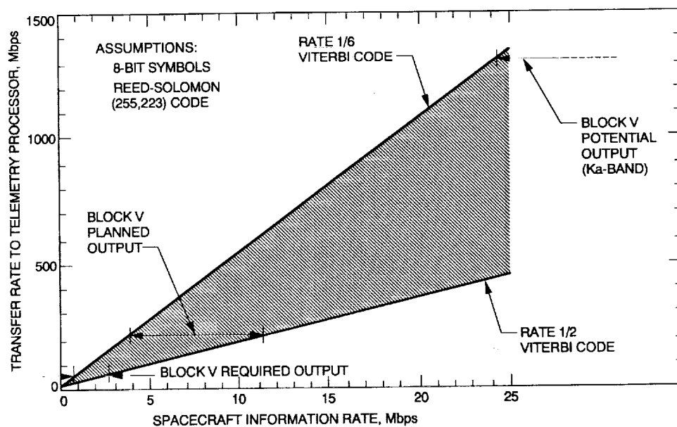
Fig. 6. Block V receiver transfer rate characteristics.
