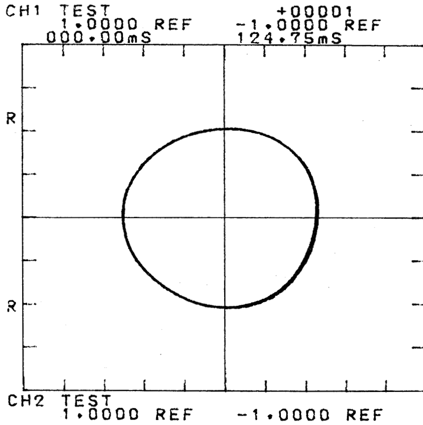
Fig.9 System's synchronous response by experiment (L=1.6cm, c/R=0.1%, m_U=7.6g , n=5280rpm )
