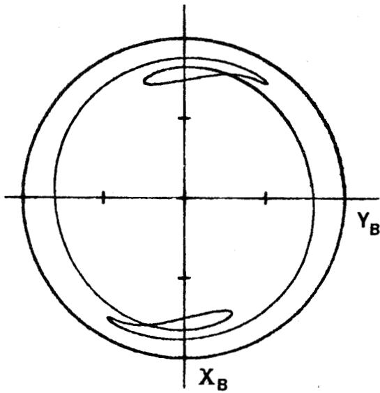
Fig.5 Nonsynchronous response in unstable region ( U=0.4, \beta=0.005, \alpha=0.2, B=0.05, K=0.01, \Omega=2.0 )
