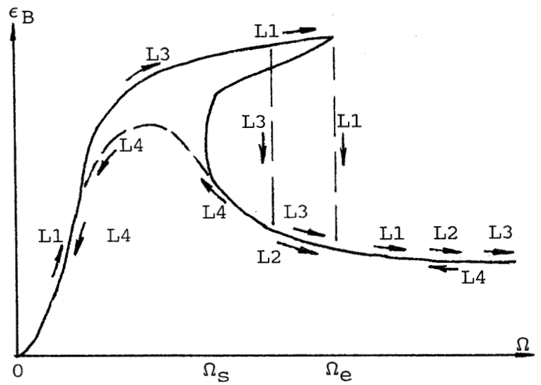
Fig.6 Schematic diagram of the influence of initial rotating speed on bistable jumping
