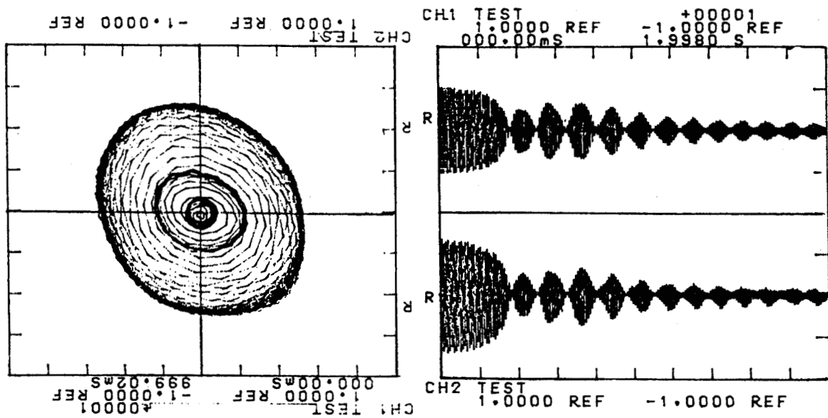
Fig.10 System's bistable response by experiment (L=1.2cm, c/R=0.1%, m_U=4.6g , n=5430rpm )
