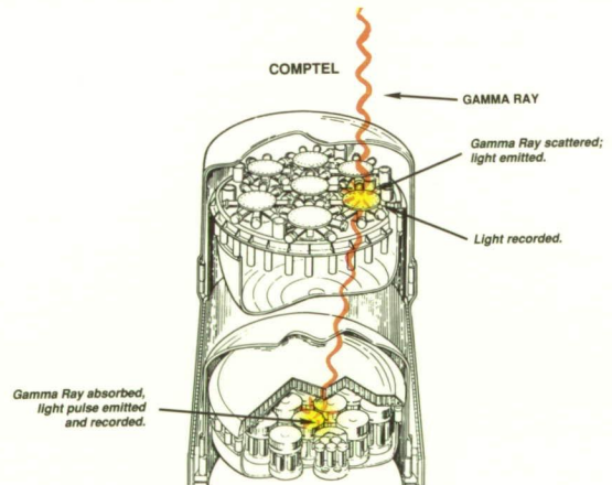
Imaging Compton Telescope (COMPTEL)
