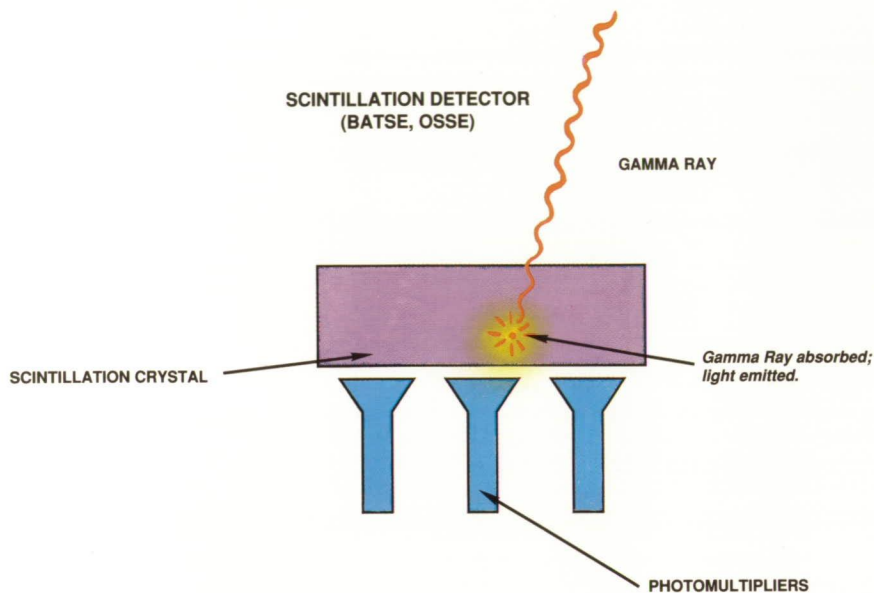
Scintillation detector
