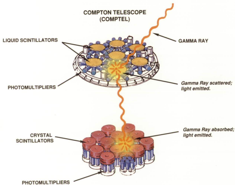
Compton telescope
