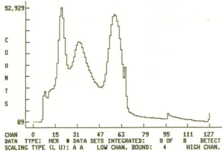
BATSE test spectrum
