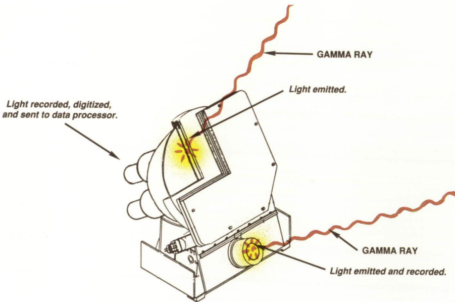
BATSE gamma-ray detection
