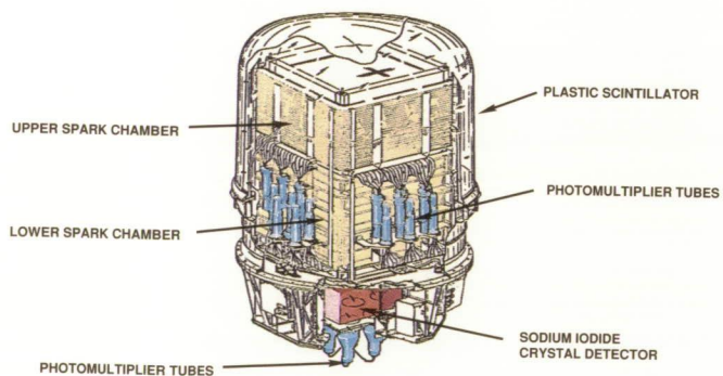
EGRET instrument
