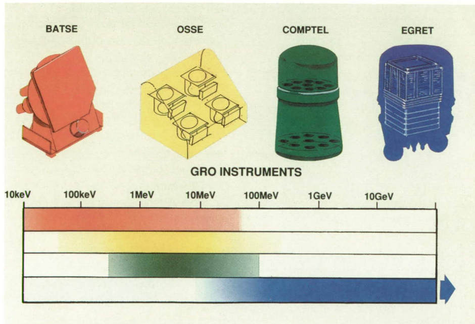
GRO energy range
