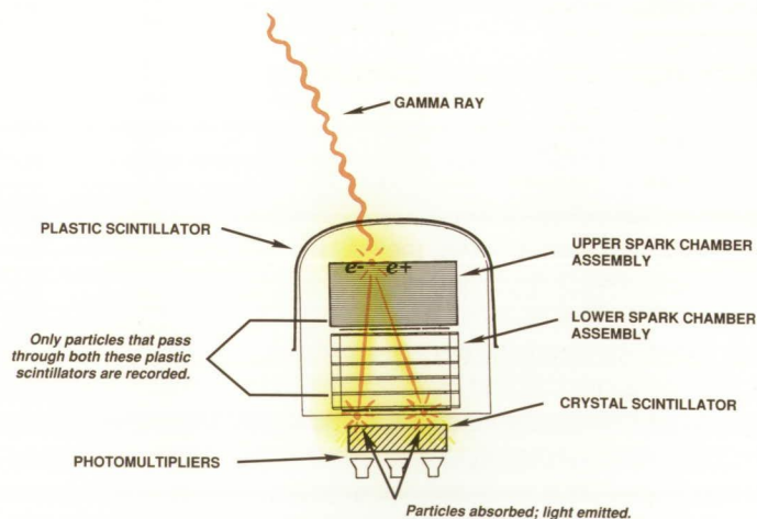
EGRET gamma-ray detection
