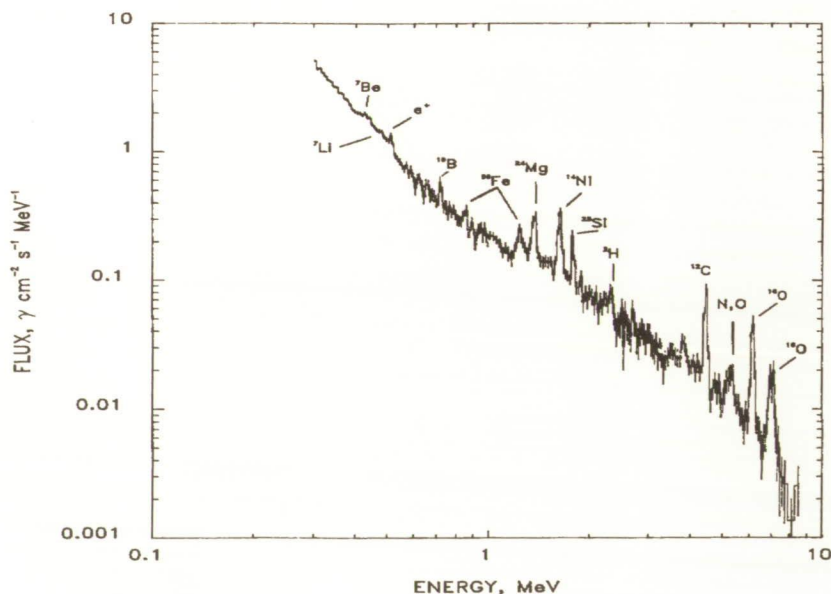
OSSE line spectrum
