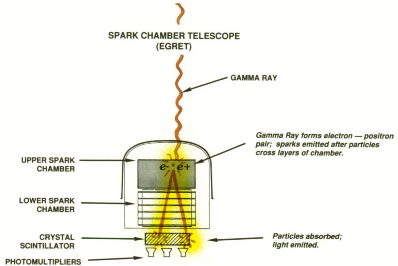
Spark chamber telescope
