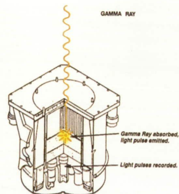
OSSE gamma-ray detection
