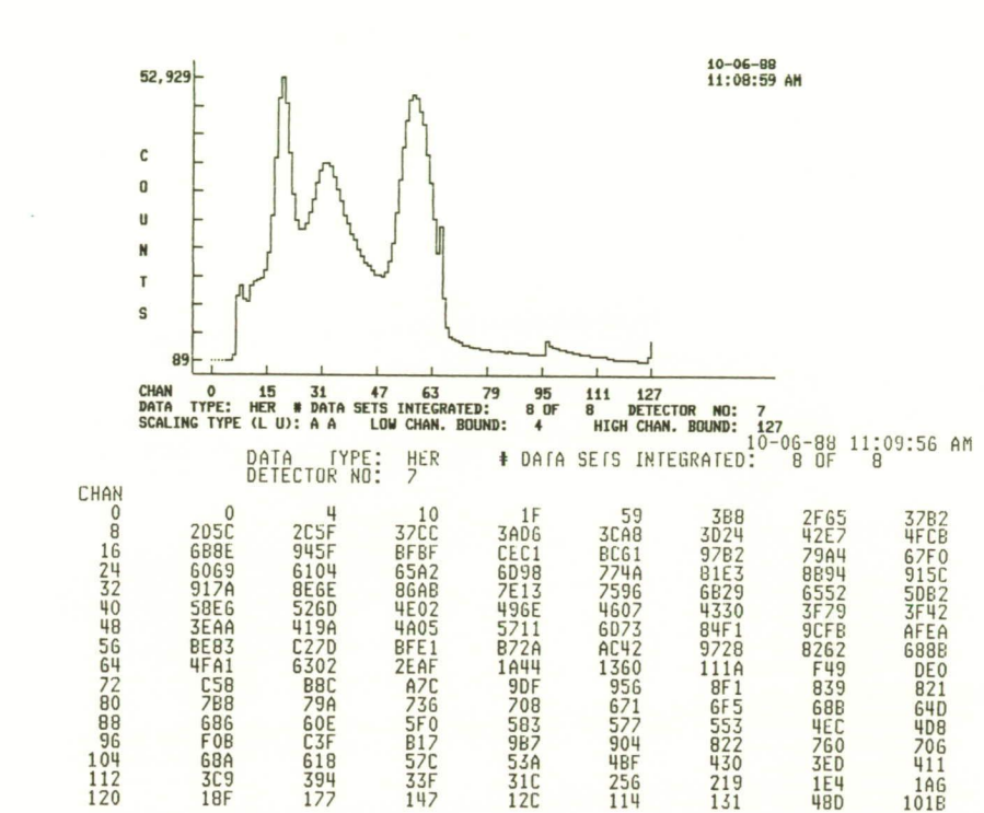
A calibration spectrum from one of the BATSE detectors. The radioactive isotope mercury 203 was used to produce this test spectrum. During a gamma-ray burst, hundreds of spectra will be obtained rapidly from the BATSE detectors in an attempt to better understand the nature of these enigmatic objects.
