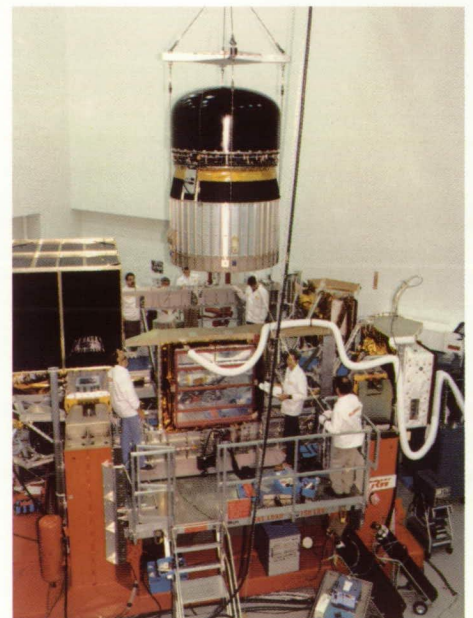
COMPTEL installation
