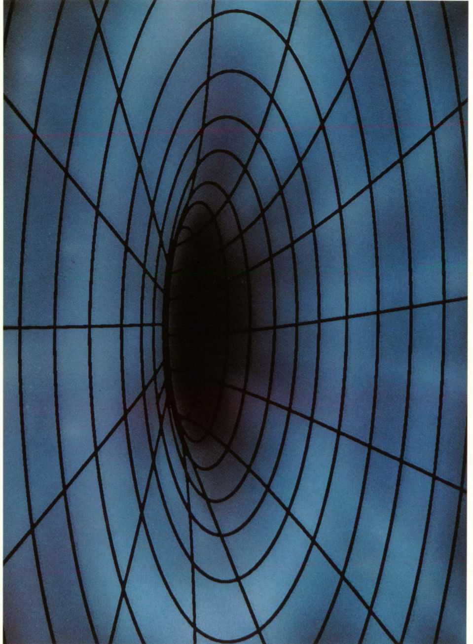
Black hole
