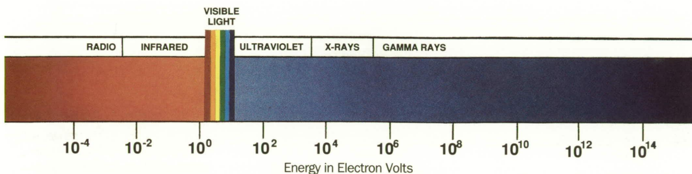
Electromagnetic spectrum
