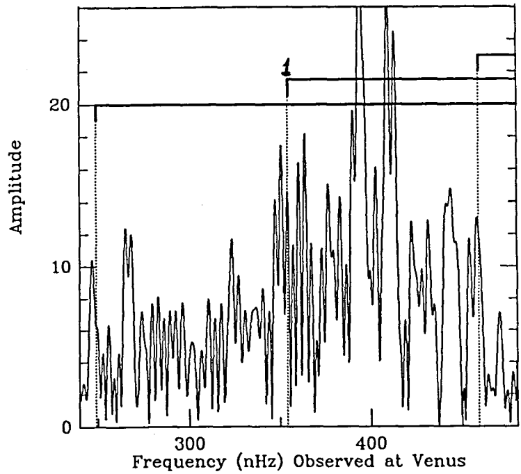
Figure 3--The degree of correspondence of g-mode frequencies (Table 1) with magnified portions of the EUV spectrum (Figure 2). Of the 21 lines, only 5 (marked X) are not detected. The g-mode spectrum appears 3 times due to aliasing at \pm 105 nHz caused by interaction with the lowest harmonic r-mode.
