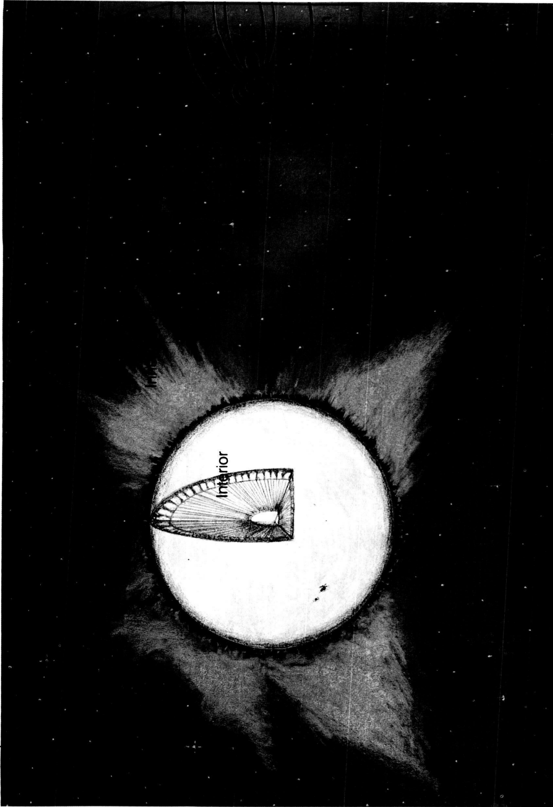
The Five Heliographic Domains
