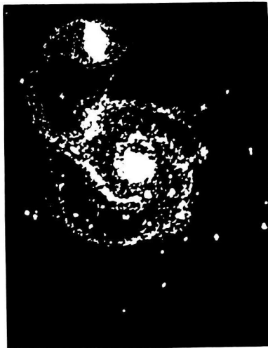
The Whirlpool Galaxy (M51)
