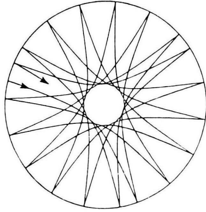
Ray Path of One Acoustic Wave Mode Traveling through the Sun's Interior
