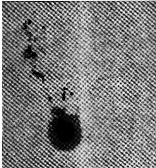
An Active Region Photographed in White Light
