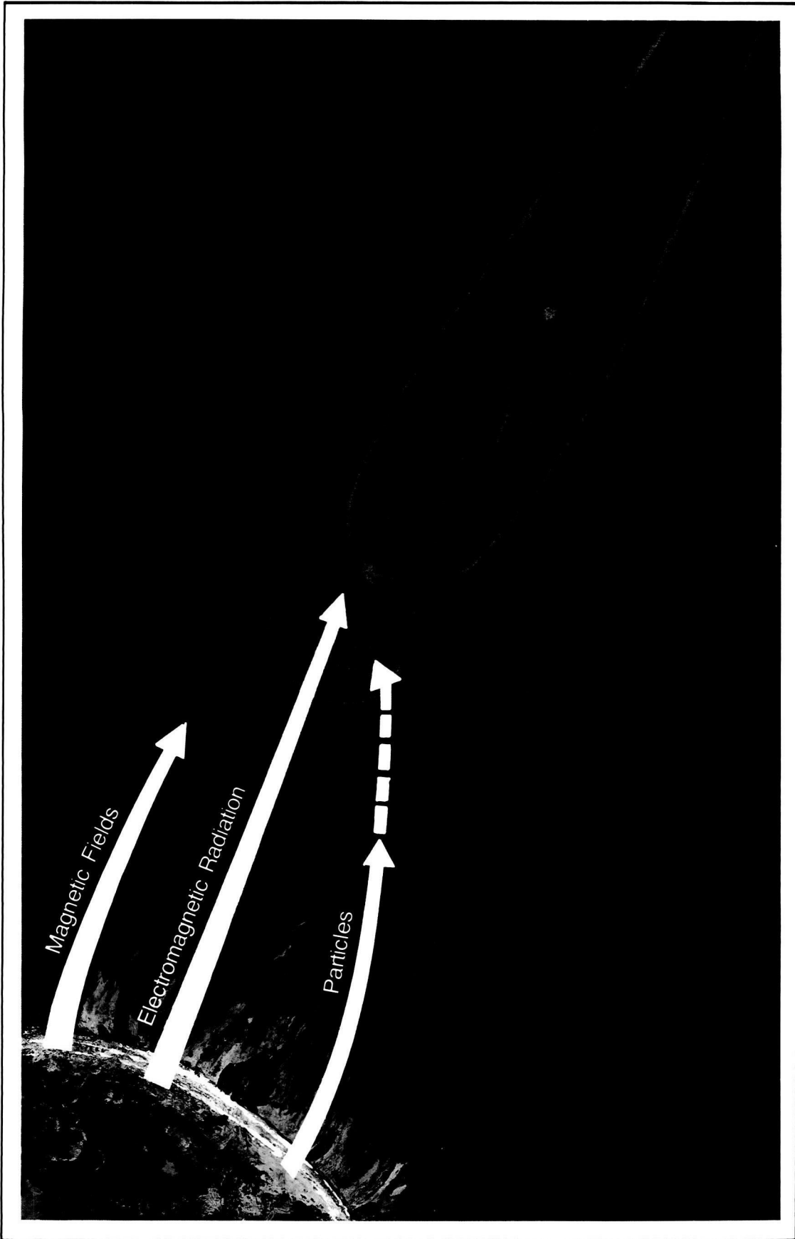
Solar Effects on the Earth (Drawing Not to Scale)
