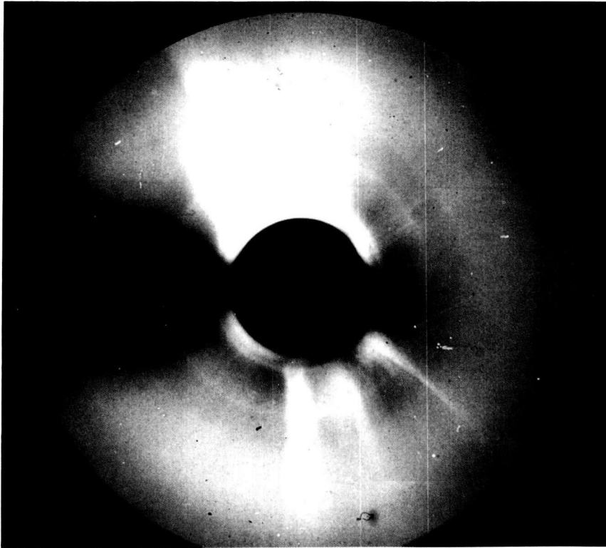
Corona Observed from Space with Coronagraph
