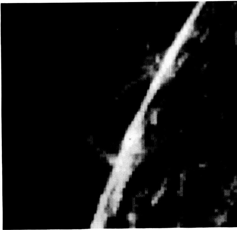
The Active Sun—Active Region Loops at Limb
