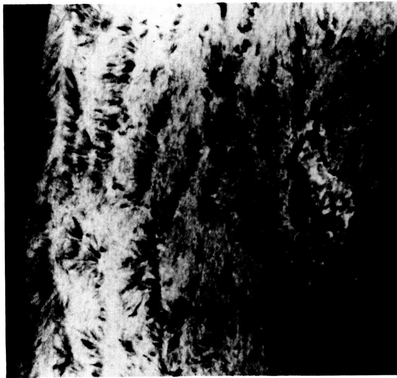
The Quiet Sun—Supergranules with Boundaries Marked by Spicules
