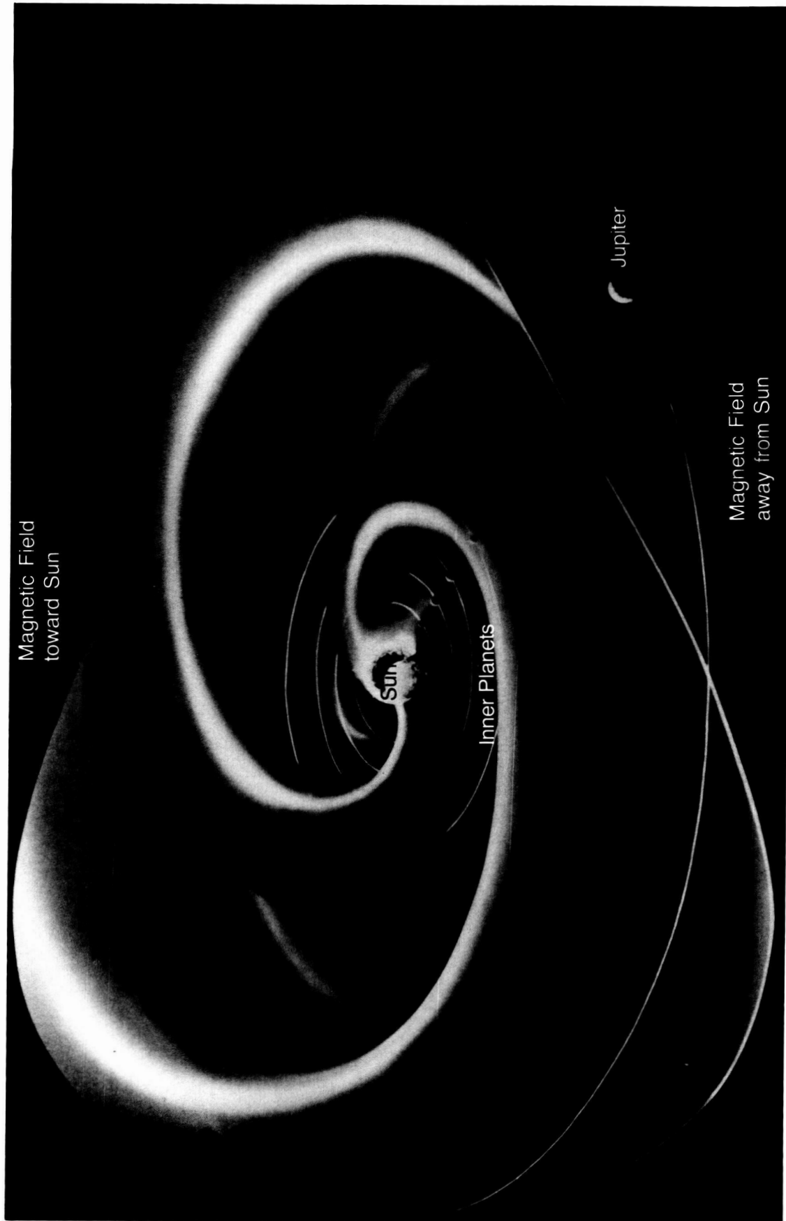
Three-Dimensional Structure of the Boundary between Magnetic Field Sectors in the Solar Wind (Artist's Concept).
