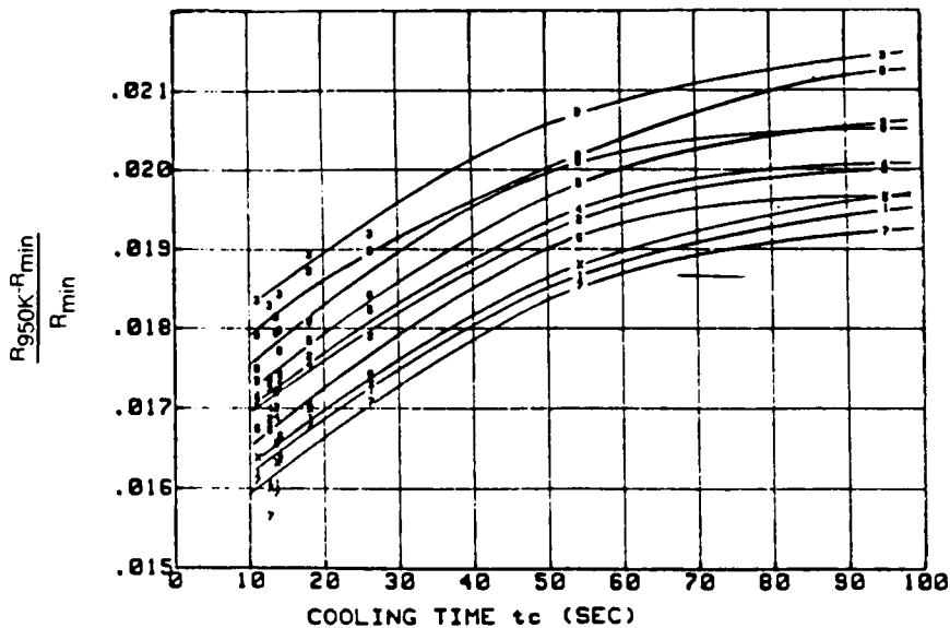
Figure 11 Gage Resistance Ratio for 8 Cooling Rates
