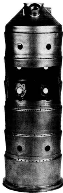
Figure 6 Burner Can with Section Cut Out
