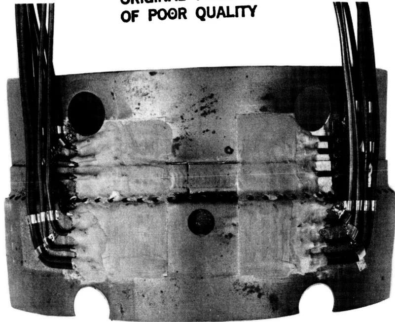
Figure 7 Instrumented Section of Burner Can
