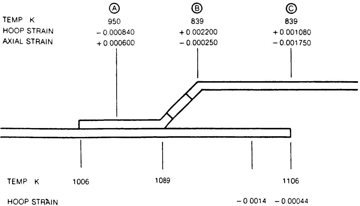
Figure 2 Strains Estimated For JT12D Burner Liner in Vicinity of Third Knuckle
