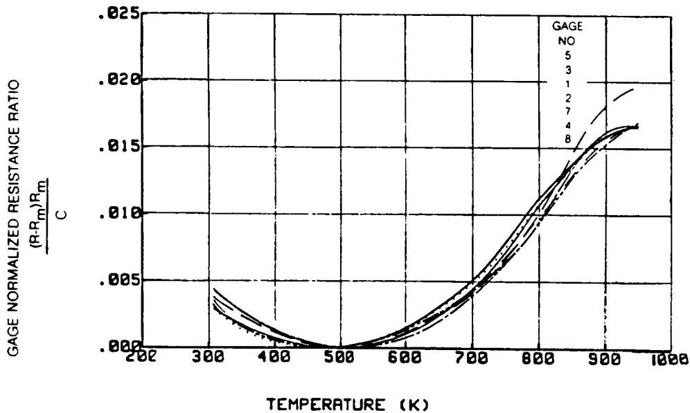
GAGE NORMALIZED RESISTANCE RATIO VERSUS TEMPERATURE DURING RAPID COOLING ( t_c = 12 seconds) FROM 950K FOR THE SEVEN GAGES ON THE BURNER LINER. AFTER THE COMBUSTOR TESTS THE CALIBRATION CONSTANT C FOR EACH GAGE IS THE SAME AS THAT USED IN FIGURE 13. THE RESULTS ARE ALL WITHIN THE ENVELOPE OF THE ORIGINAL CALIBRATION CURVES OF FIGURE 13 EXCEPT FOR GAGE NO. 5 WHICH EXPERIENCED OVER-TEMPERATURES TO 1041K DURING THE COMBUSTOR TESTS.
