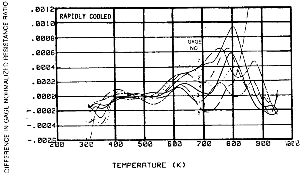
DIFFERENCE IN GAGE NORMALIZED RESISTANCE RATIO VERSUS TEMPERATURE FROM BEFORE TO AFTER THE BURNER TESTS FOR RAPID COOLING ( t_c = 12 seconds) FROM 950K. THE DIFFERENCE BETWEEN FIGURE 13 and FIGURE 14 IS PLOTTED FOR EACH GAGE.
