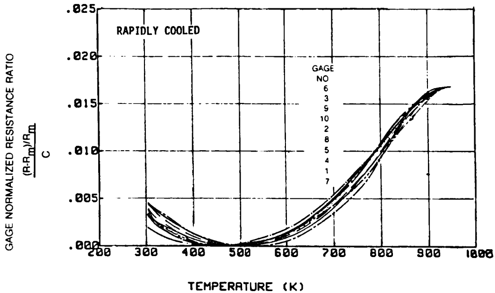
GAGE NORMALIZED RESISTANCE RATIO VERSUS TEMPERATURE DURING RAPID COOLING ( t_c = 12 seconds) FROM 950K FOR THE TEN GAGES ON THE BURNER LINER BEFORE THE COMBUSTOR TESTS.
