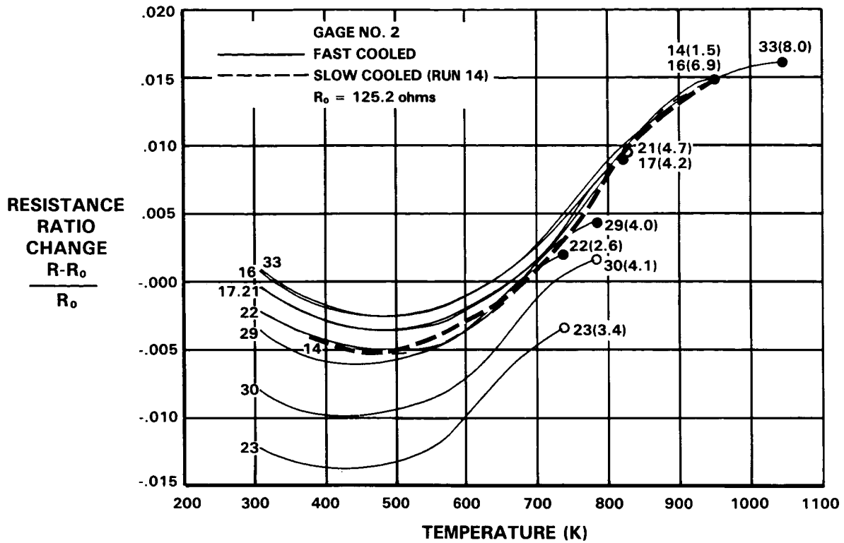
RESISTANCE RATIO CHANGE VERSUS TEMPERATURE OF KANTHAL A-1 STRAIN GAGE NO. 2 DURING RAPID COOLING FOR VARIOUS STARTING TEMPERATURES AND VARIOUS DWELL TIMES AT THE STARTING TEMPERATURE. A SOLID SYMBOL INDICATES DWELL TIME OF FIVE TO TEN MINUTES; AN OPEN SYMBOL INDICATES DWELL TIME OF TWENTY TO THIRTY MINUTES. THE NUMBER ON THE CURVE IS THE RUN NUMBER OF TABLE 1 AND THE NUMBER IN PARENTHESES IS THE COOLING RATE (K/SEC) IN THE 800K TO 700K RANGE.
