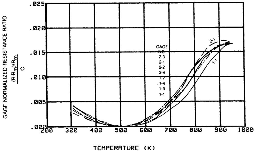
GAGE NORMALIZED RESISTANCE RATIO VERSUS TEMPERATURE DURING RAPID COOLING ( t_c = 12 seconds) FROM 950K FOR THE EIGHT GAGES ON THE TWO GAGE-FACTOR TEST BARS. ALL OF THESE CURVES FALL WITHIN THE ENVELOPE OF FIGURE 13.
