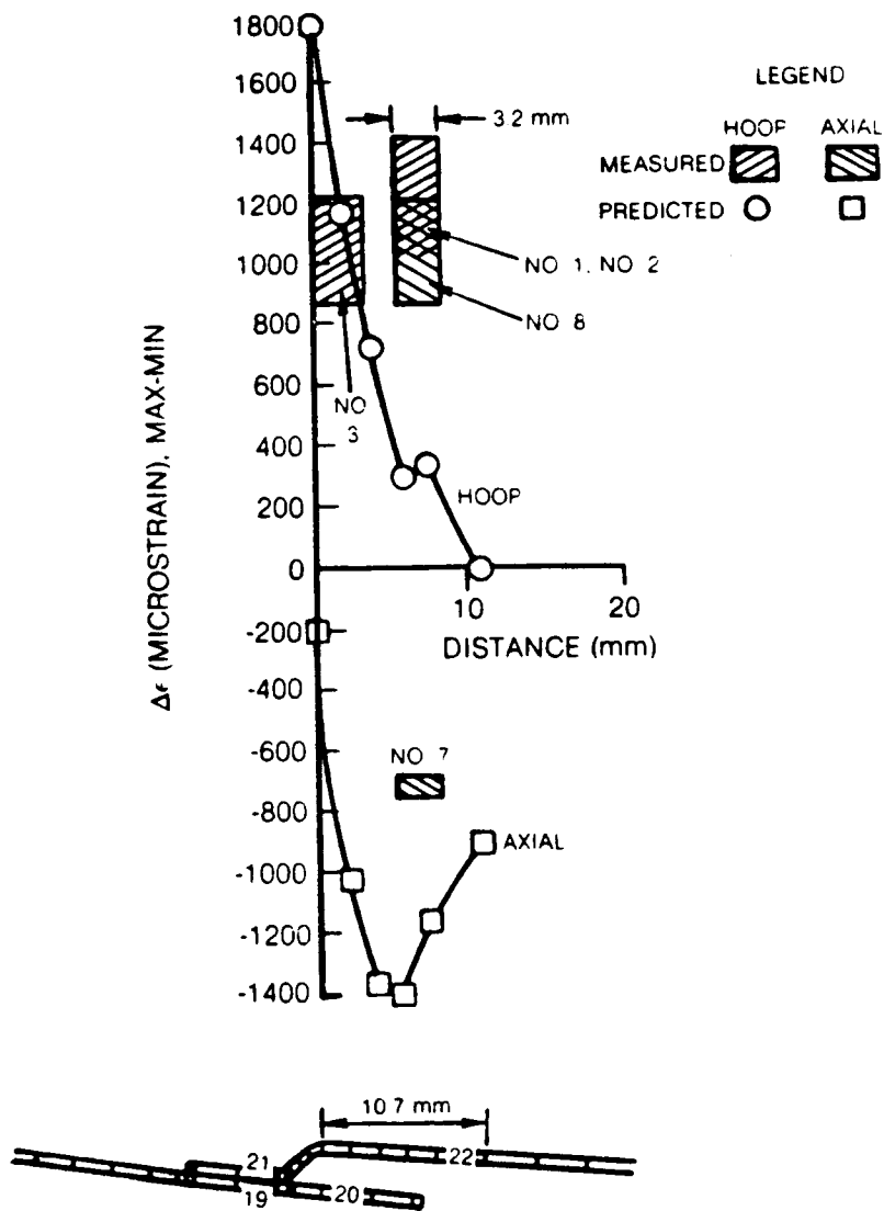
PREDICTED MECHANICAL STRAIN RANGE (USING AVERAGE TEMPERATURES) AND MEASURED STRAIN RANGE (USING KANTHAL A-1 GAGES) DURING BURNER CYCLES 4, 5, 6, 7.
