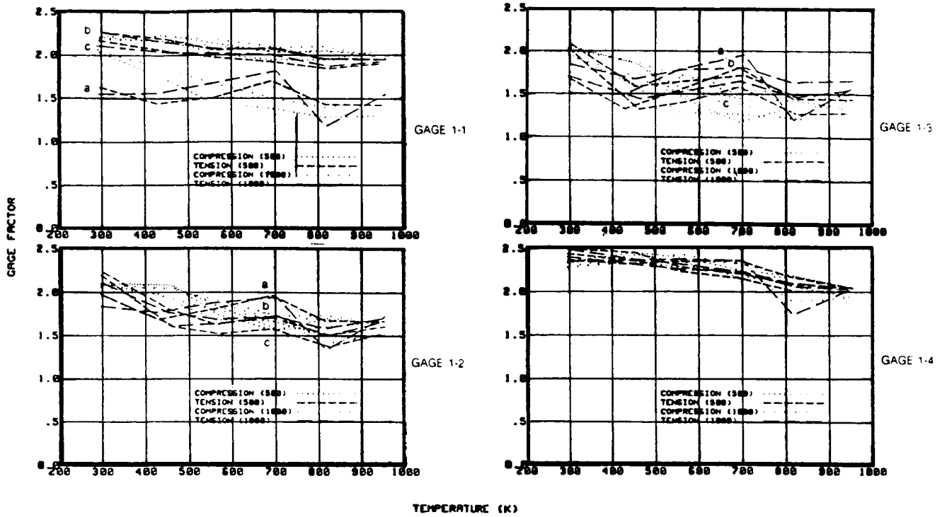
GAGE FACTOR VERSUS TEMPERATURE FOR THE FOUR GAGES ON BAR #1 (a) FIRST TEST, (b) AFTER 200 HOURS AT 950K, (c) Repeat of b.
