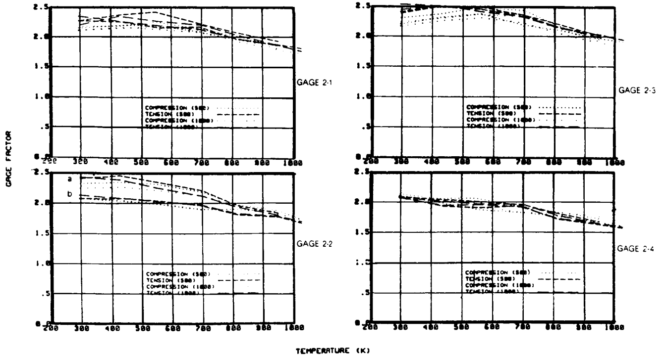
GAGE FACTOR VERSUS TEMPERATURE FOR FOUR GAGES ON BAR #2 (a) FIRST TEST, (b) AFTER RAPID COOLING FROM 950K TO ROOM TEMPERATURE AT t_c = 12 seconds.
