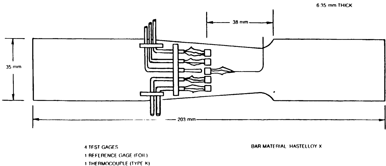
Figure 10 Gage Factor Test Bar
