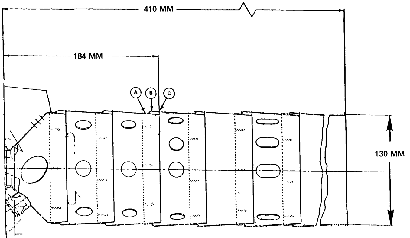
Figure 1 JT12D Burner Liner
