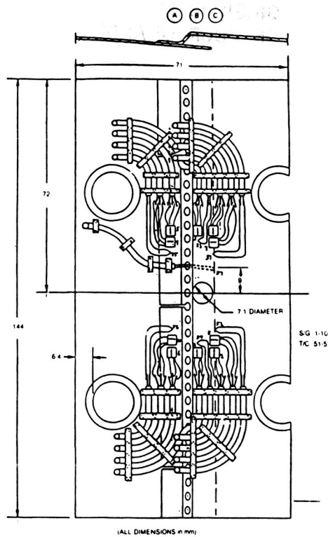
Figure 5 Strain Gage & Thermocouple Locations
