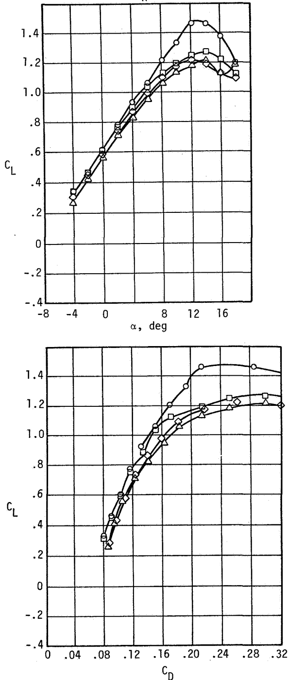
Figure 3. Effects of heavy rain on C_L and C_D
