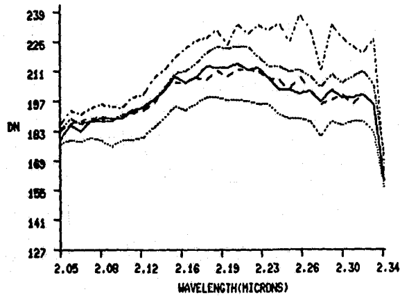
Fig. 3. The ratios of the Stanford data representing four rooftops from the section of the Stanford campus containing red tile roofs were determined from the formula: ratio = 50 + 75 * target/standard. The grass area of Fig. 2 served as the standard.
