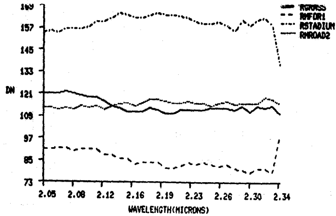
Fig. 2. The ratios of four ground targets in the Stanford flightline were determined from the formula: ratio = 50 + 75 * target/standard. The ground targets are bleachers in the football stadium (top curve), forest (bottom curve), playing field in stadium (solid curve), and a road surface. A large grass area served as the standard.
