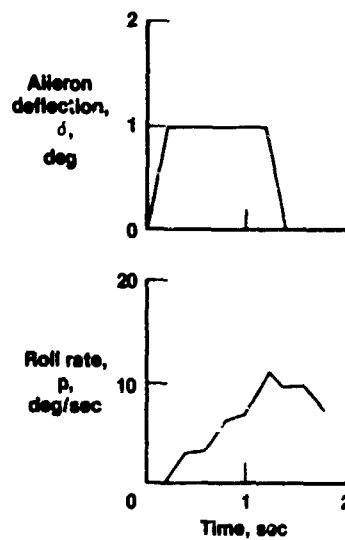
Fig. 5 Time history with measurement noise.
