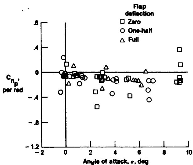
Fig. 28 Variations of C_{n_p}' with angle of attack without uncertainty levels.
