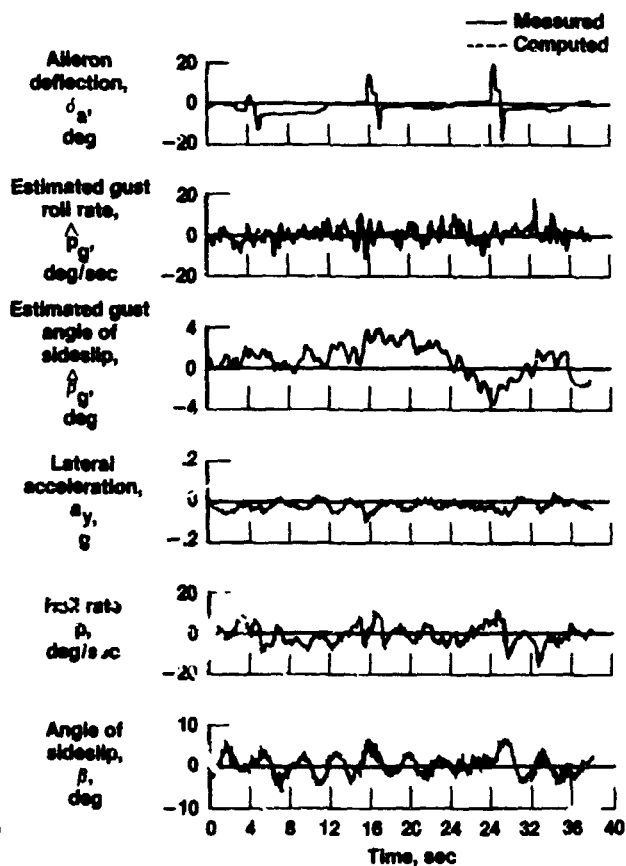
Fig. 31 Match of flight data obtained in turbulence (state noise) and computed data obtained from a maximum likelihood estimator that accounts for turbulence.
