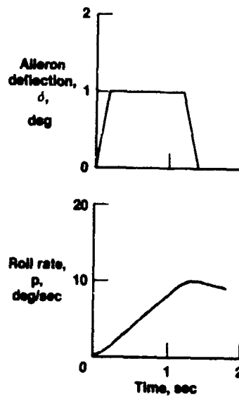
Fig. 3 Time history with no measurement noise.
