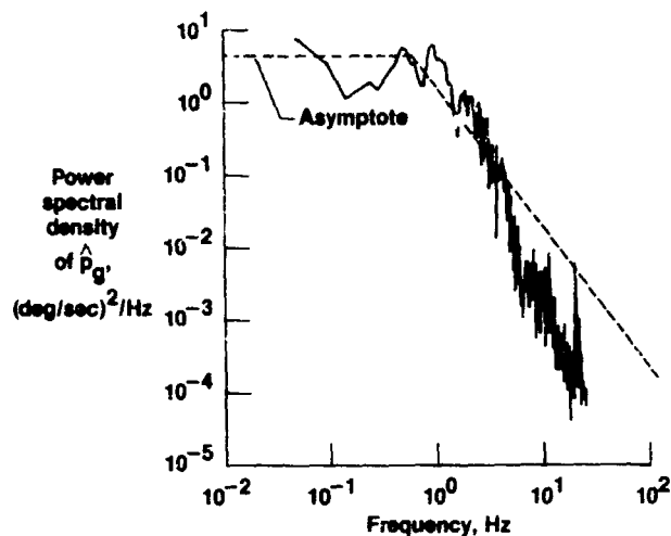
Fig. 33 Power spectral density of \hat{p}_g obtained from maneuver shown in Fig. 31.
