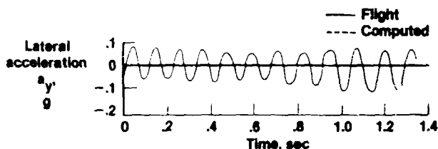
Fig. 34 Structural mode oscillation observed on the lateral acceleration.
