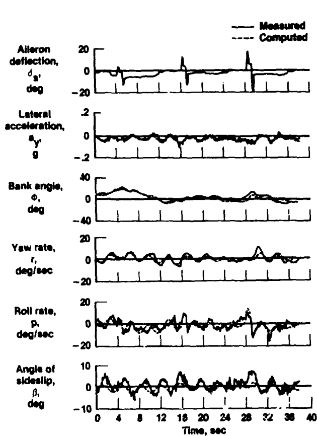
Fig. 30 Match of flight data obtained in turbulence (state noise) and computed data obtained from maximum likelihood estimator that does not account for turbulence.
