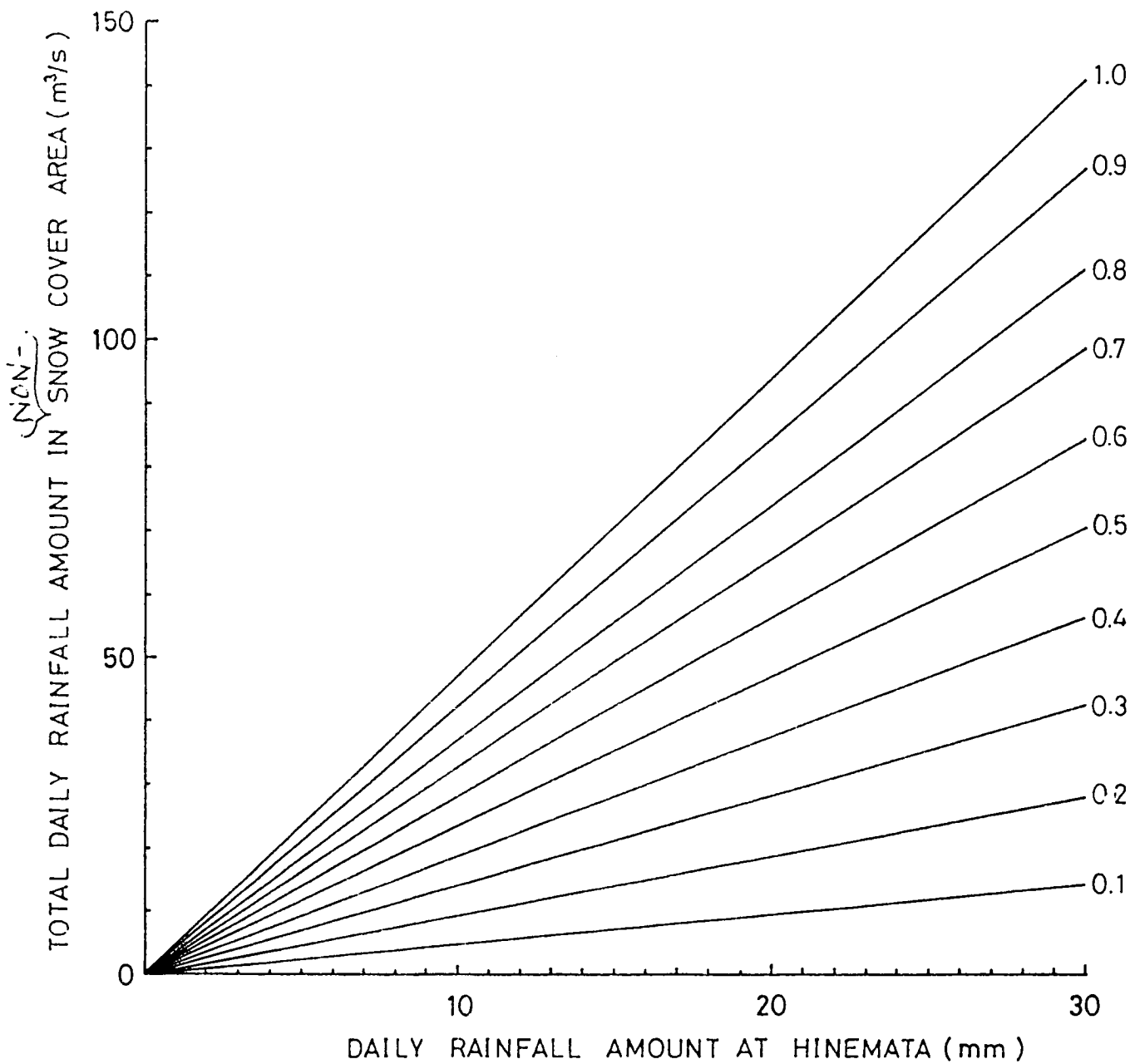
Figure 12. Nomograph(V) for Total Daily Rainfall Amount in Non-Snow Cover Area in Use of Daily Rainfall at Hinoemata Station. (Parameter: Relative Non-Snow Cover Area, 1-S_{n-}/A )
