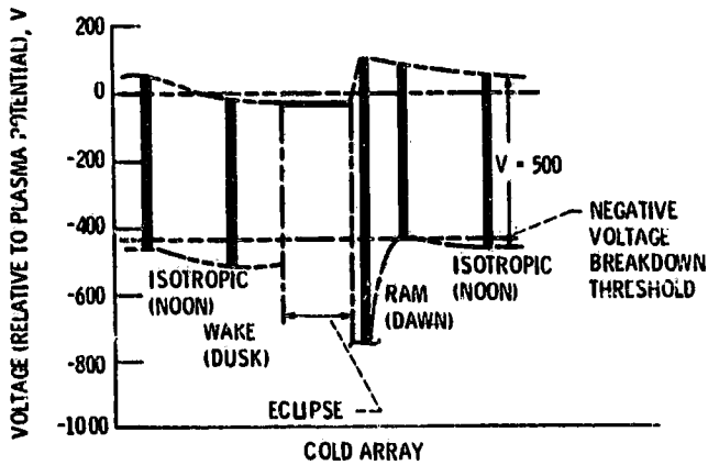
Figure 11. - Orbital variations in operating conditions - 400-km orbit.
