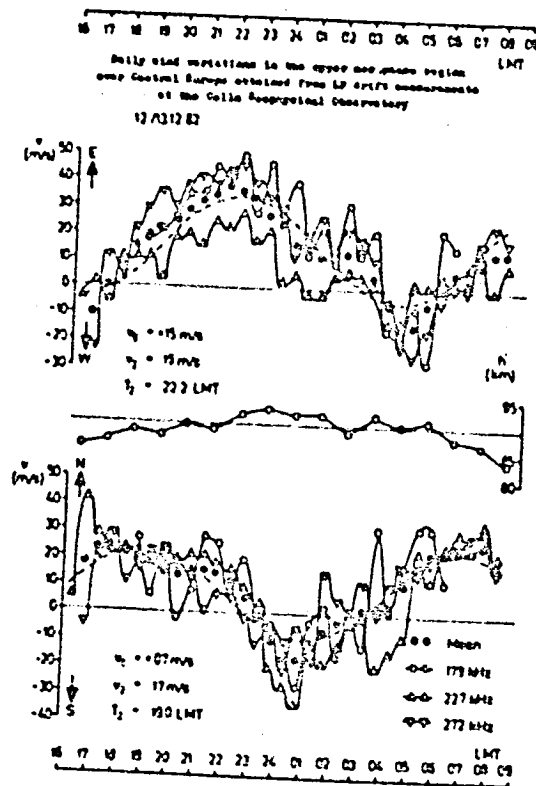
Figure 1. Daily wind variations in the upper mesopause region over Central Europe obtained from LF drift measurements at the Colln Geophysical Observatory.
