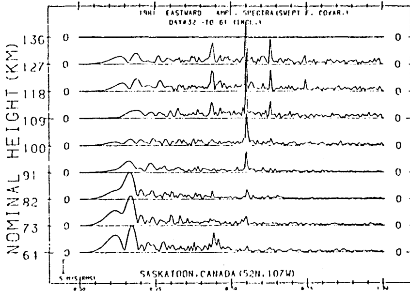
Figure 4. Spectra for February 1981 -- during STRATWARM (-5 km).
