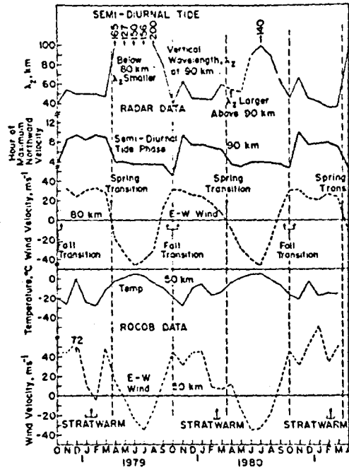
Figure 7. Semi-diurnal tidal variations.
