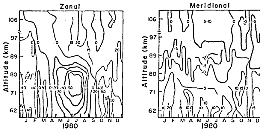
Figure 2. Zonal and meridional winds (10-d averages used): 1980.
