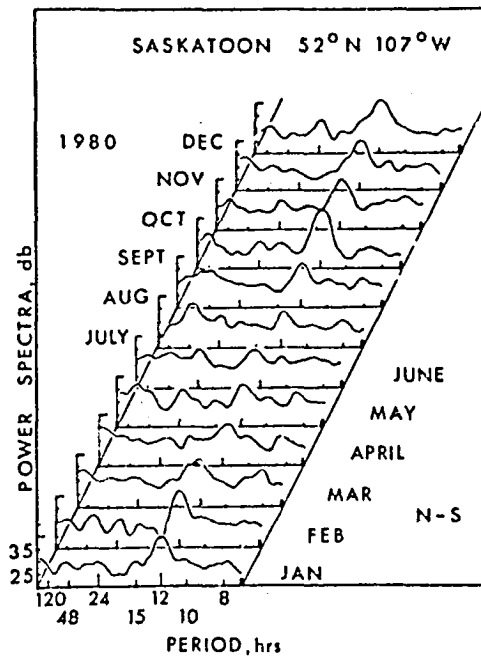
Figure 5. Fourier analysis for 89 km.
