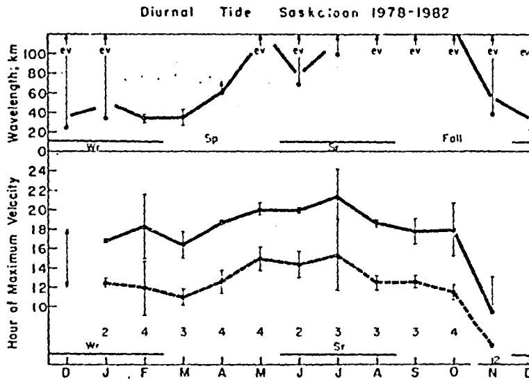
Figure 8. Diurnal tide variations.
