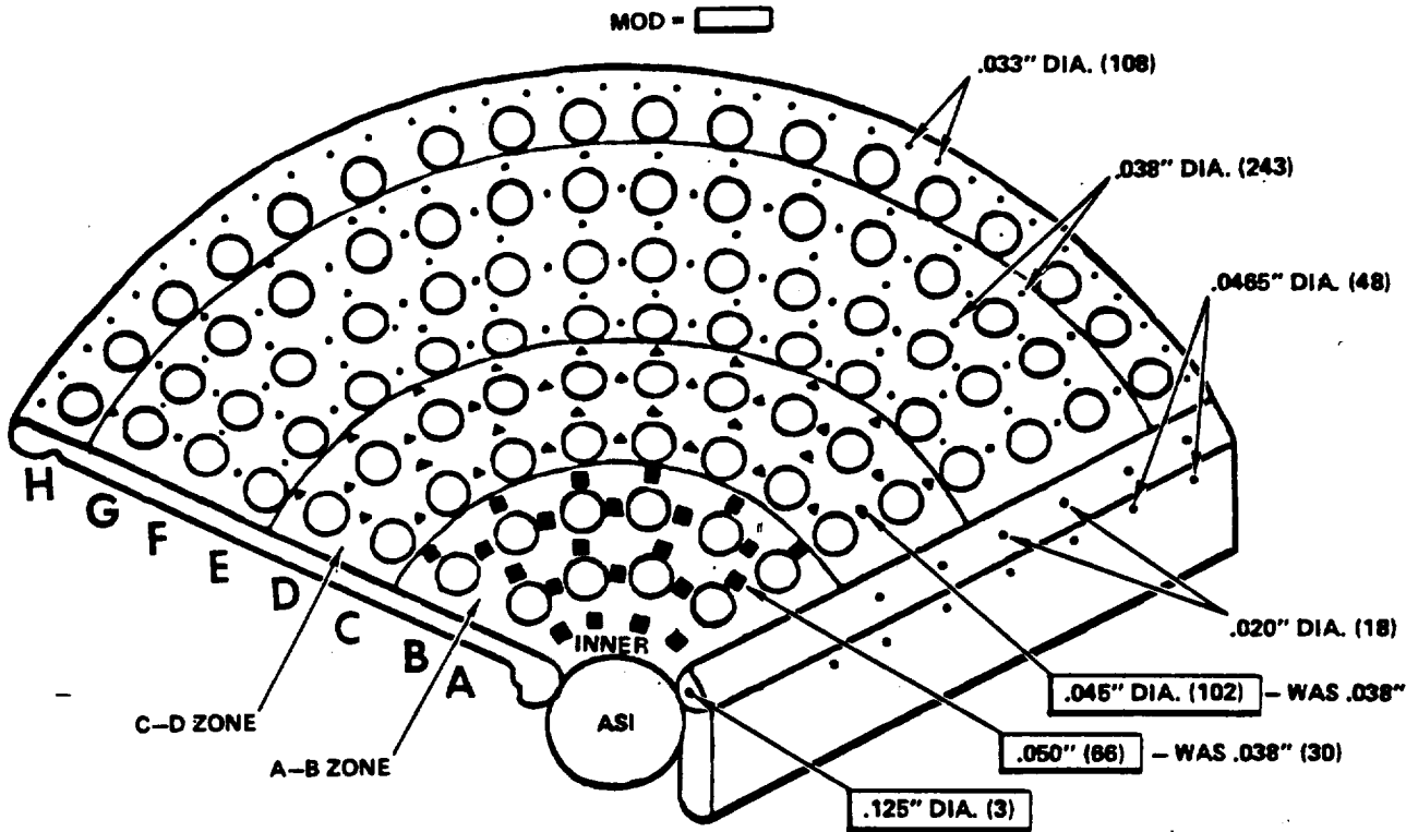
Figure 19. Fuel Preburner Injector Modification.
