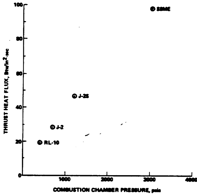
Figure 8. Combustion Chamber Heat Flux.
