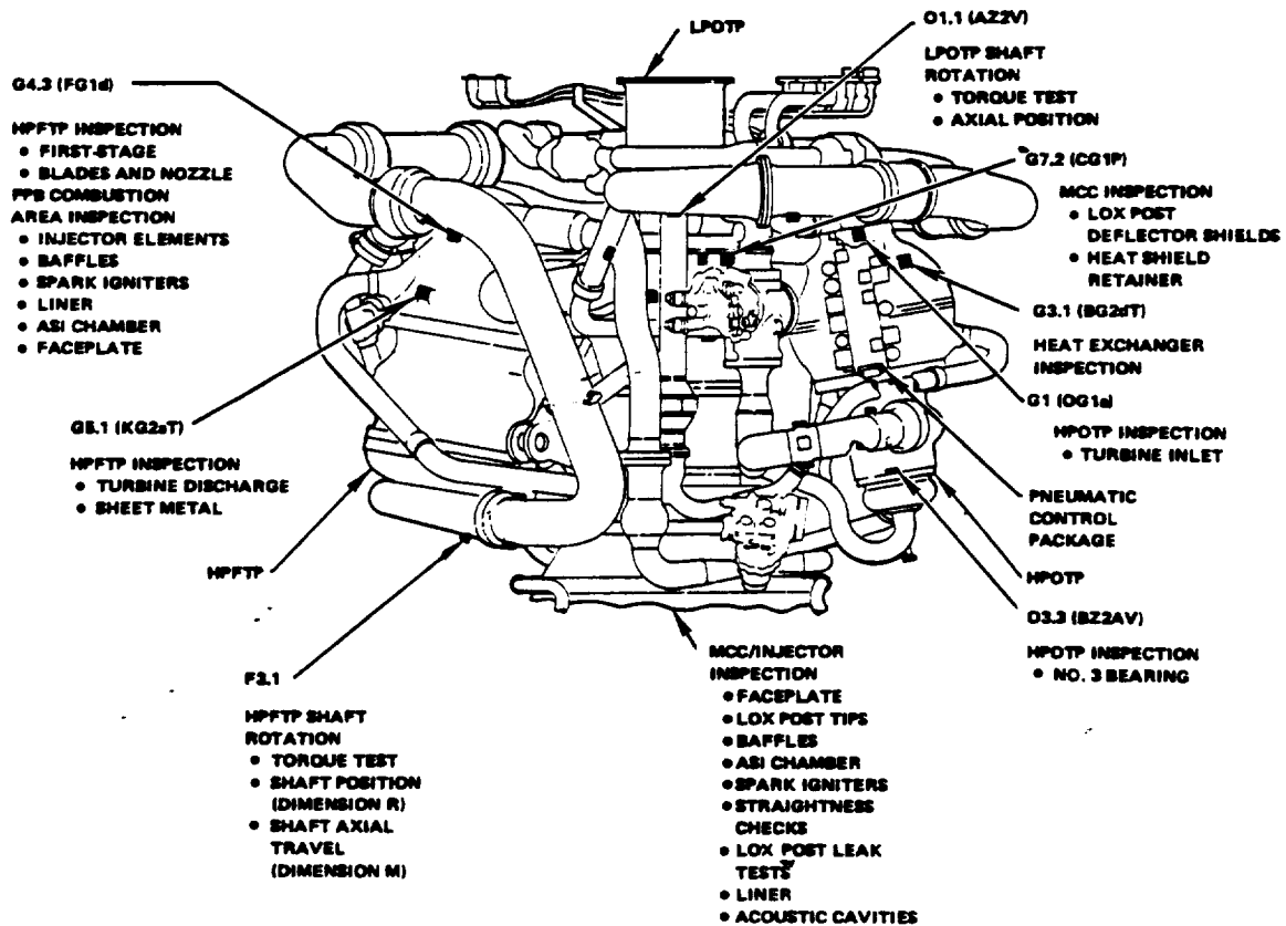
Figure 24. Internal Inspection and Shaft Rotation Access LPOTP Side of Engine.
