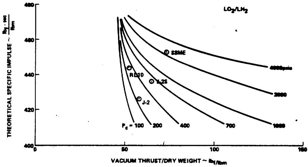
Figure 3. \text{LH}_2/\text{LO}_2 Rocket Engine Performance Characteristics.
