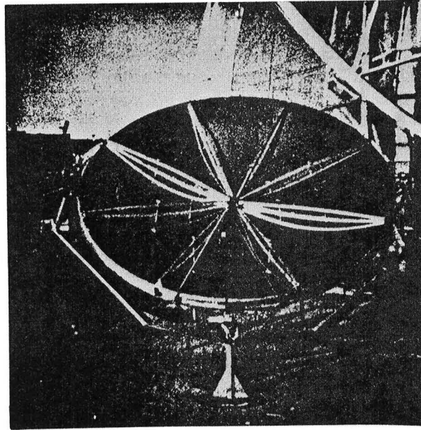
Fig. 16 3,5 m dish with sectorial reinforcement
