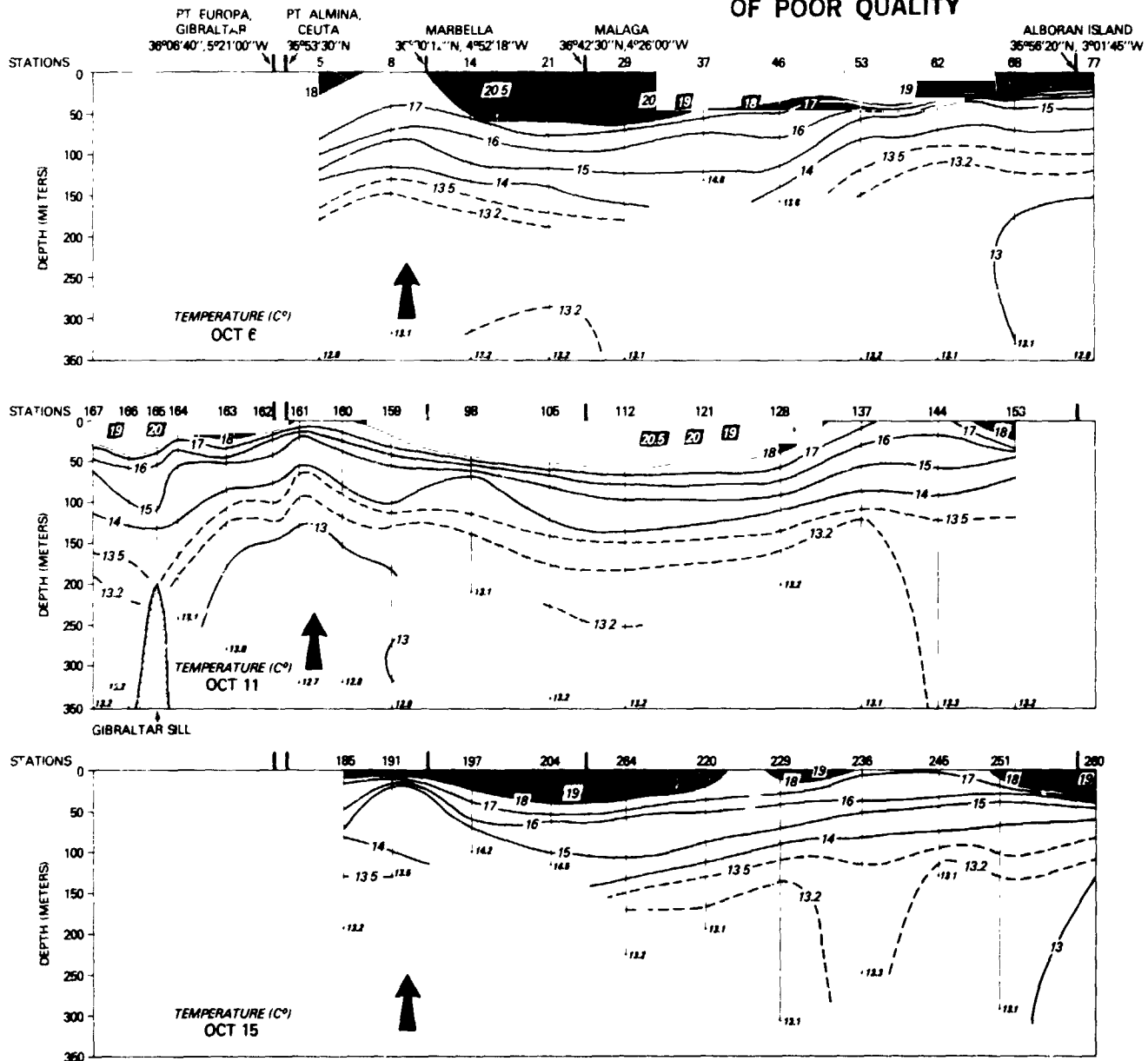
Figure 6. East-west vertical temperature sections taken along the 36° latitude (data based on aircraft XBTs). The arrows refer to cold water features found near the Strait of Gibraltar. The 6 October arrow refers to the "v's" in Figure 4, whereas the arrow on 11 October refers to the "bars" shown in the same figure (La Violette, 1984).
