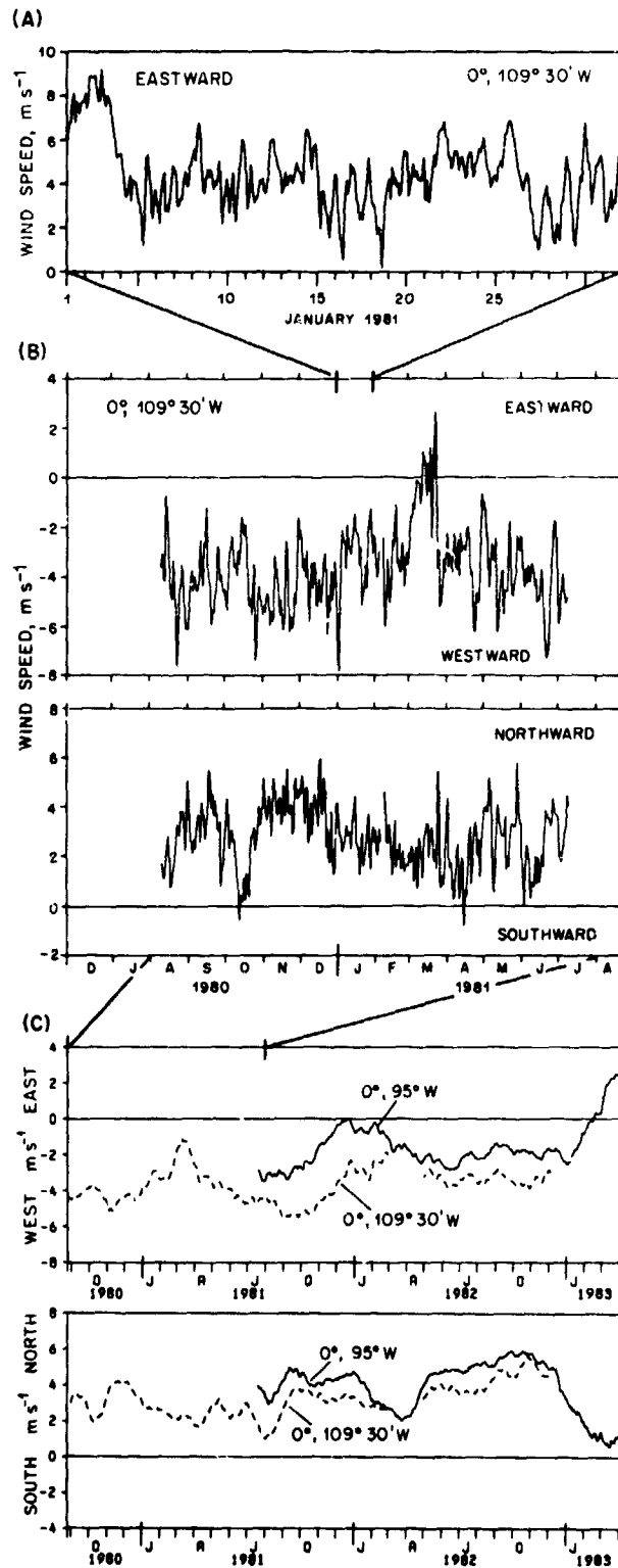
Figure 3. Time series of moored wind measurements. (A) Two-hour vector-averaged values of zonal wind at 0°, 109°30'W during January 1981. (B) Daily vector-averaged values of zonal and meridional wind at 0°, 109°30'W from August 1980 to July 1981. (C) Low-pass (31-day running mean) filtered zonal and meridional wind data at 0°, 109°30'W (dashed line) and 0°, 95°W (solid line).
