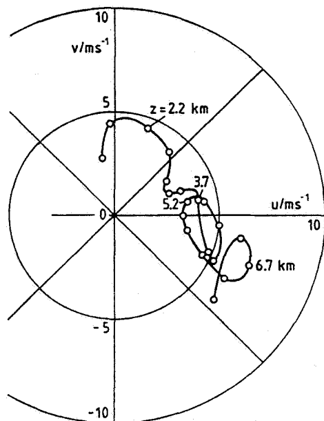
Figure 8. Polar plot of horizontal wind velocity measured during a lee wave event. The open circles denote height increments of 300 m.
