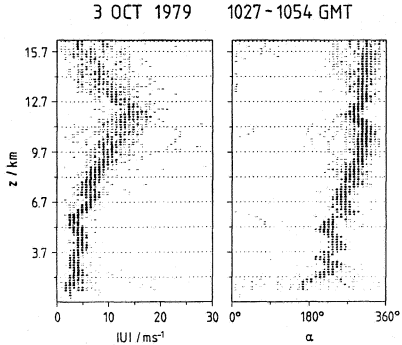
Figure 7. Height profiles of speed |U| and direction \alpha of the horizontal wind measured during a lee wave event over the Harz mountains.
