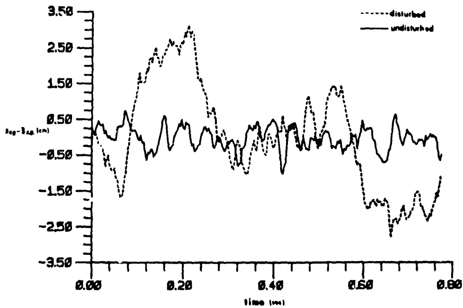
Figure 6. Variation of s Component of Centroid with Time J = 16, T_{jet} - T_{\infty} = 61.1^{\circ}C
