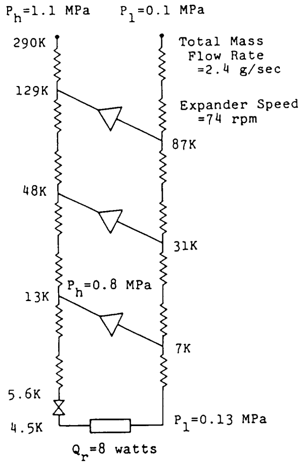
Fig. 6 Typical result of a test operation.
