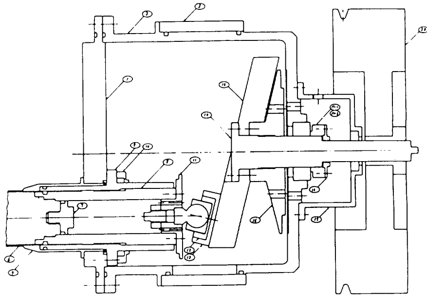
Fig. 2 Bottom end of the expansion engine and the swash plate mechanism.
